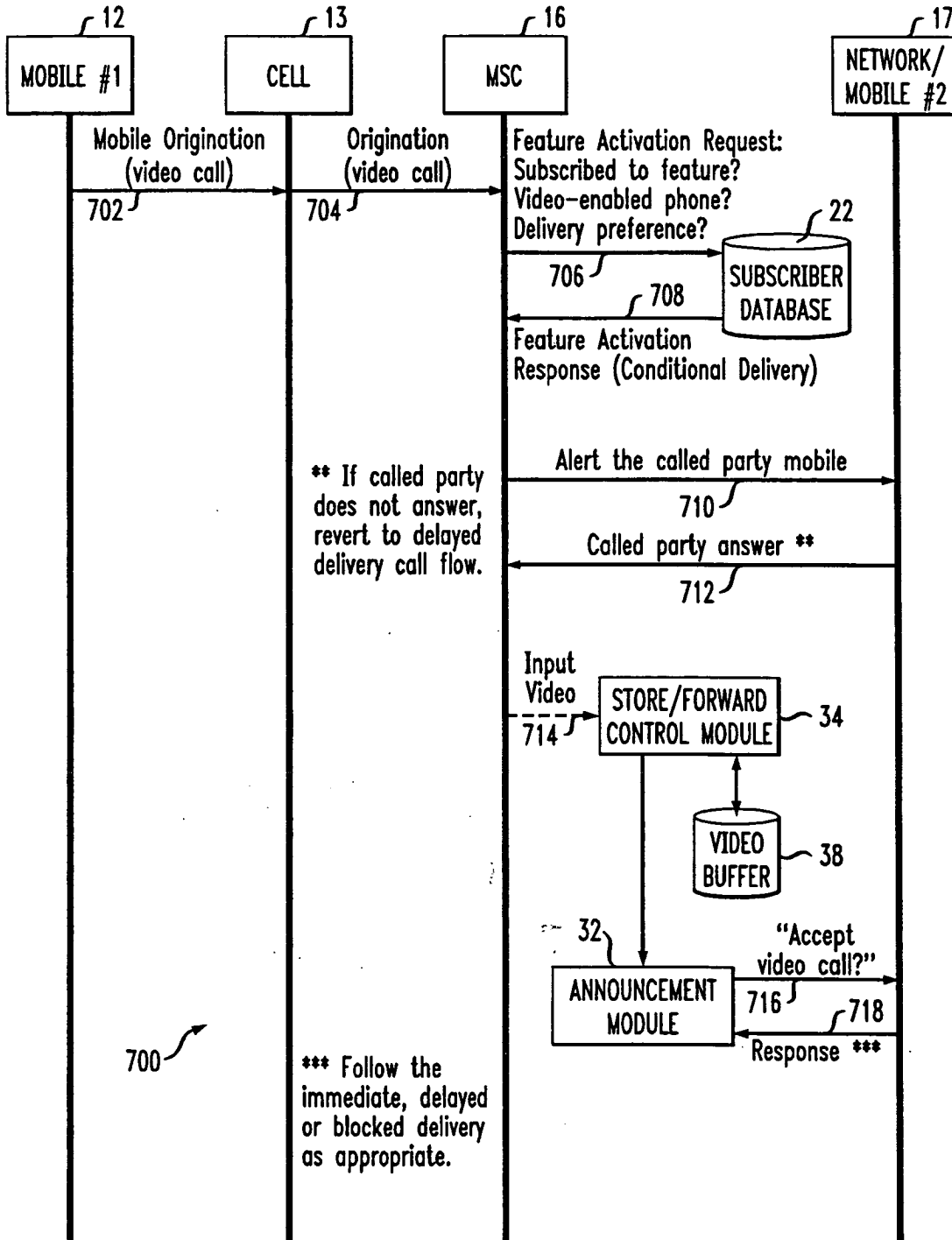
NETWORK SUPPORT FOR MOBILE-TO-MOBILE VIDEO (CONDITIONAL DELIVERY)
