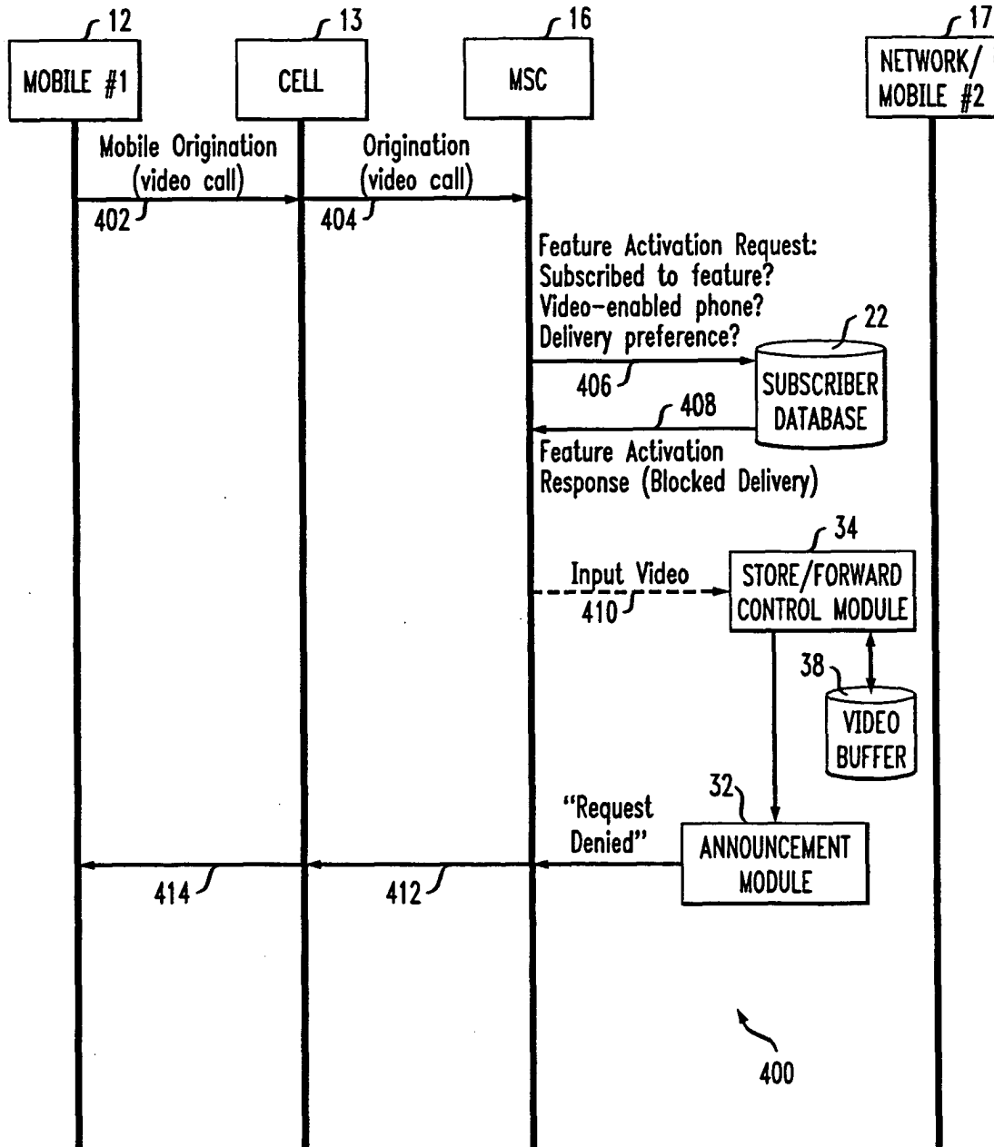
FIG. 5 NETWORK SUPPORT FOR MOBILE-TO-MOBILE VIDEO (BLOCKED DELIVERY)
