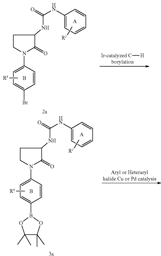
Scheme 3
