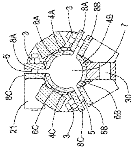
FIG. 2C VIEW B-B
