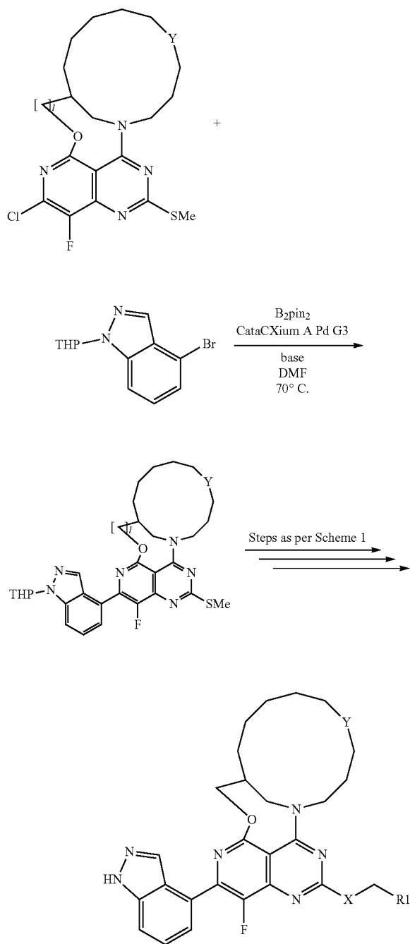
Scheme 2: General Method B
