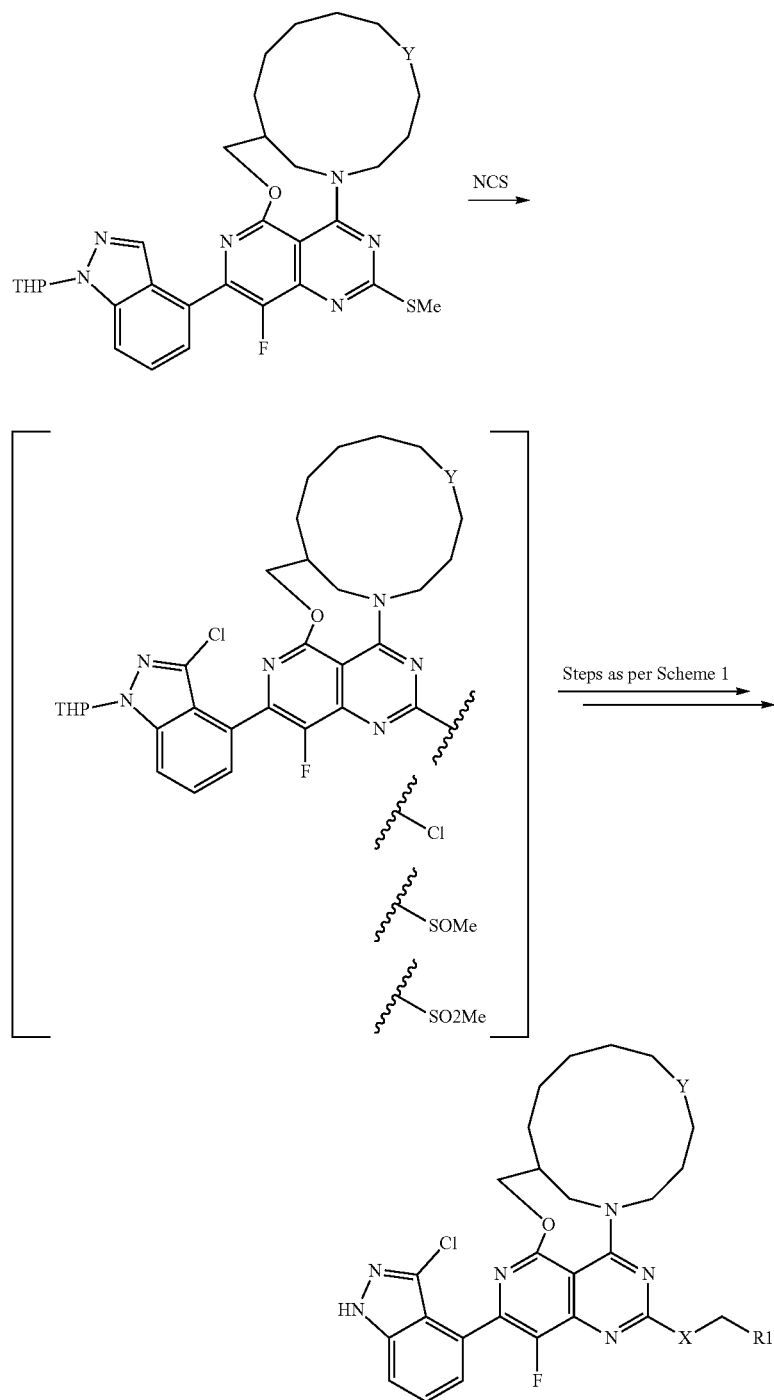
Scheme 4: General Method D
