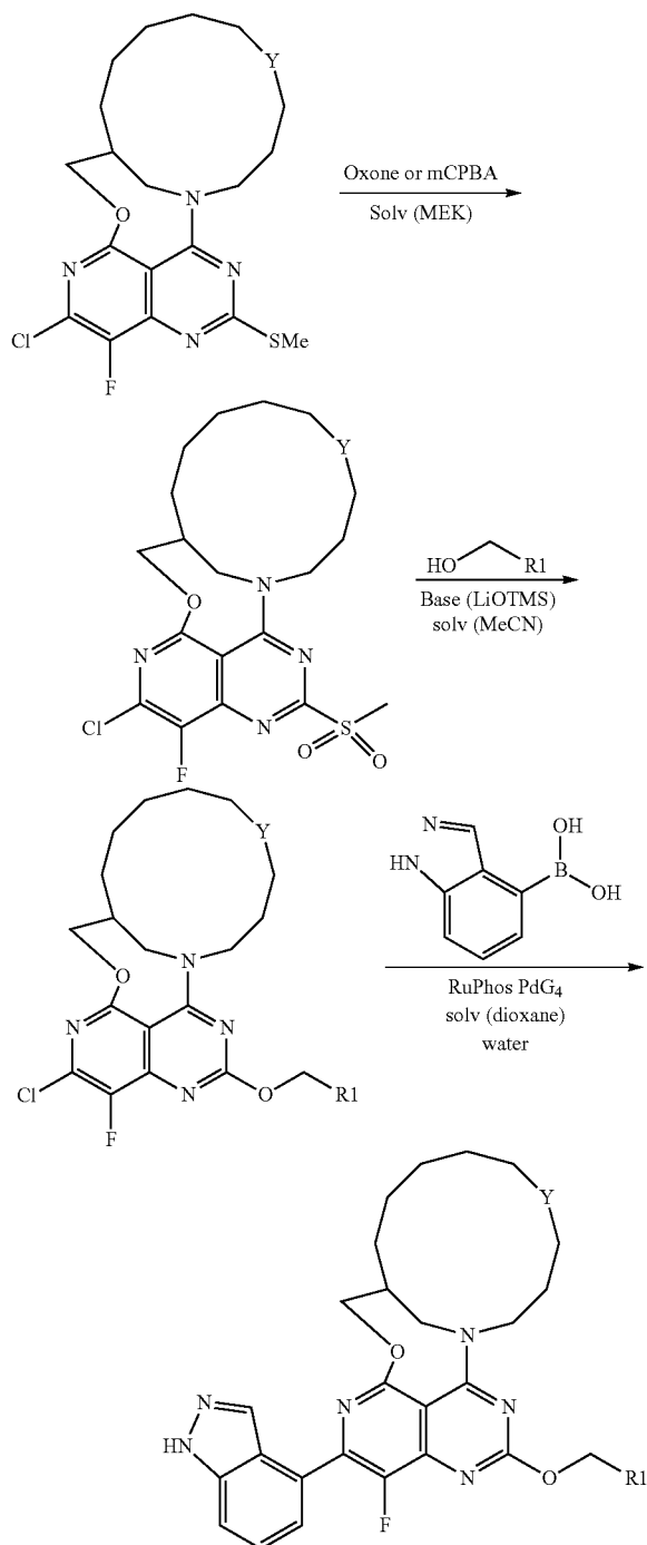
Scheme 5: General Method E
