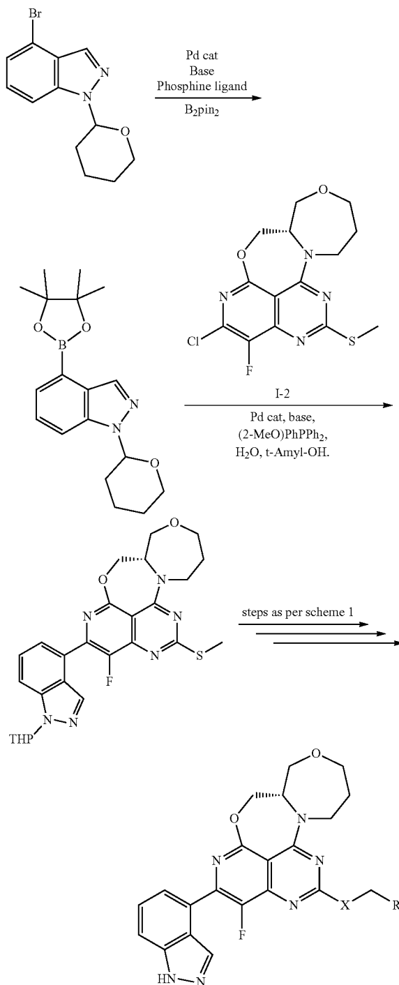
Scheme 3: General Method C
