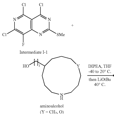
Scheme 1: General Method A
