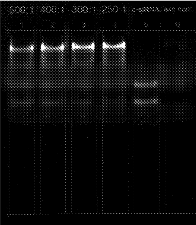
Fluorophore
