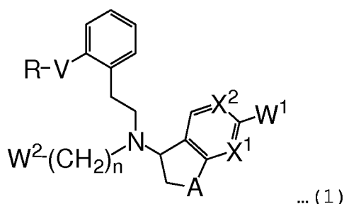
General Formula (1)
