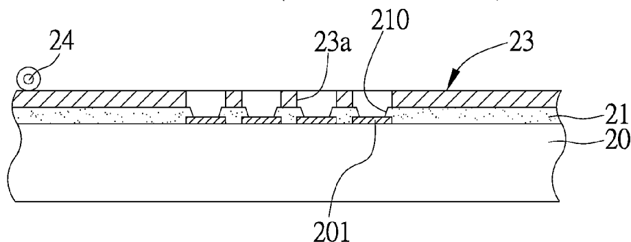
FIG. 2C (PRIOR ART)
