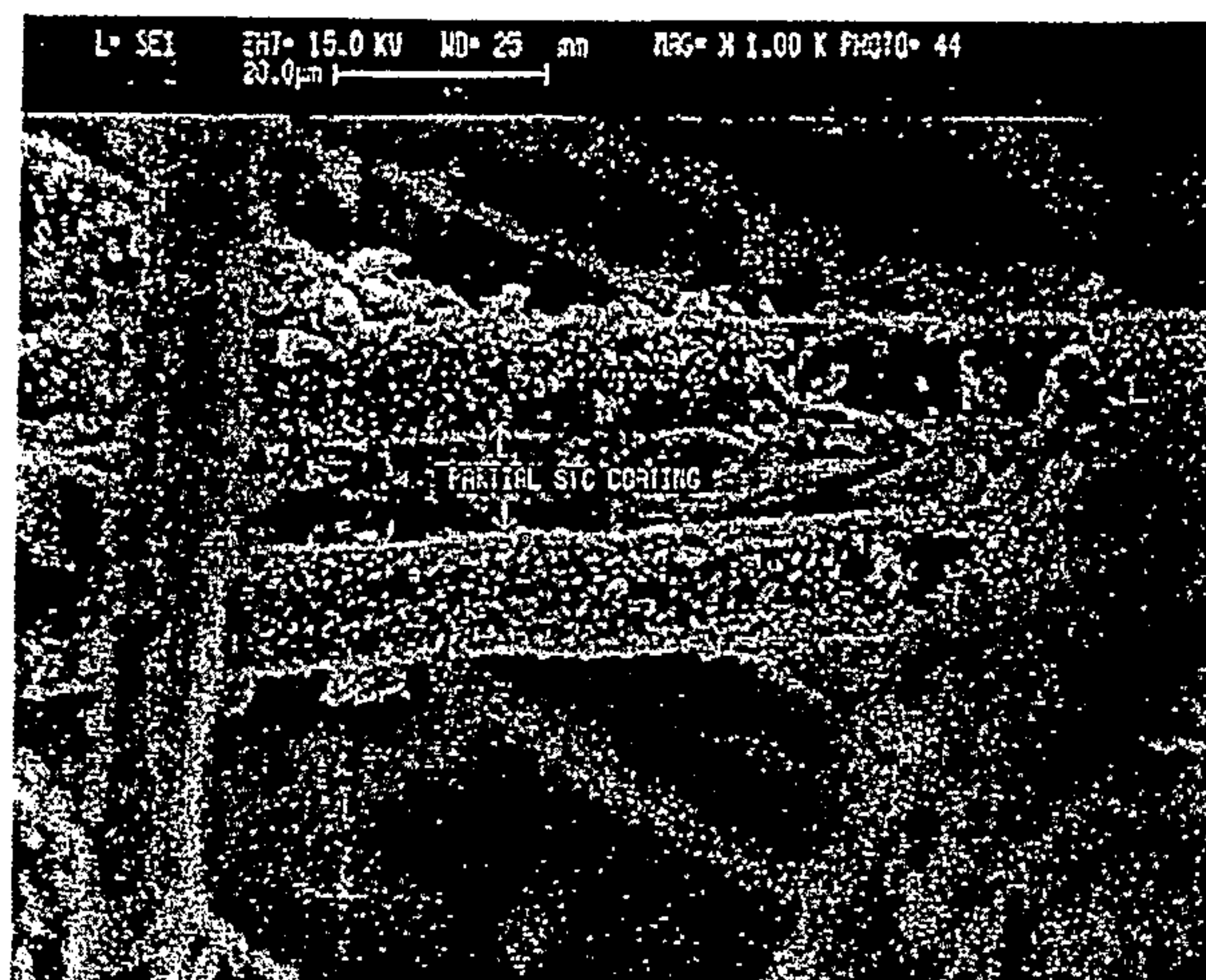
Figure 7: Damaged coating.
