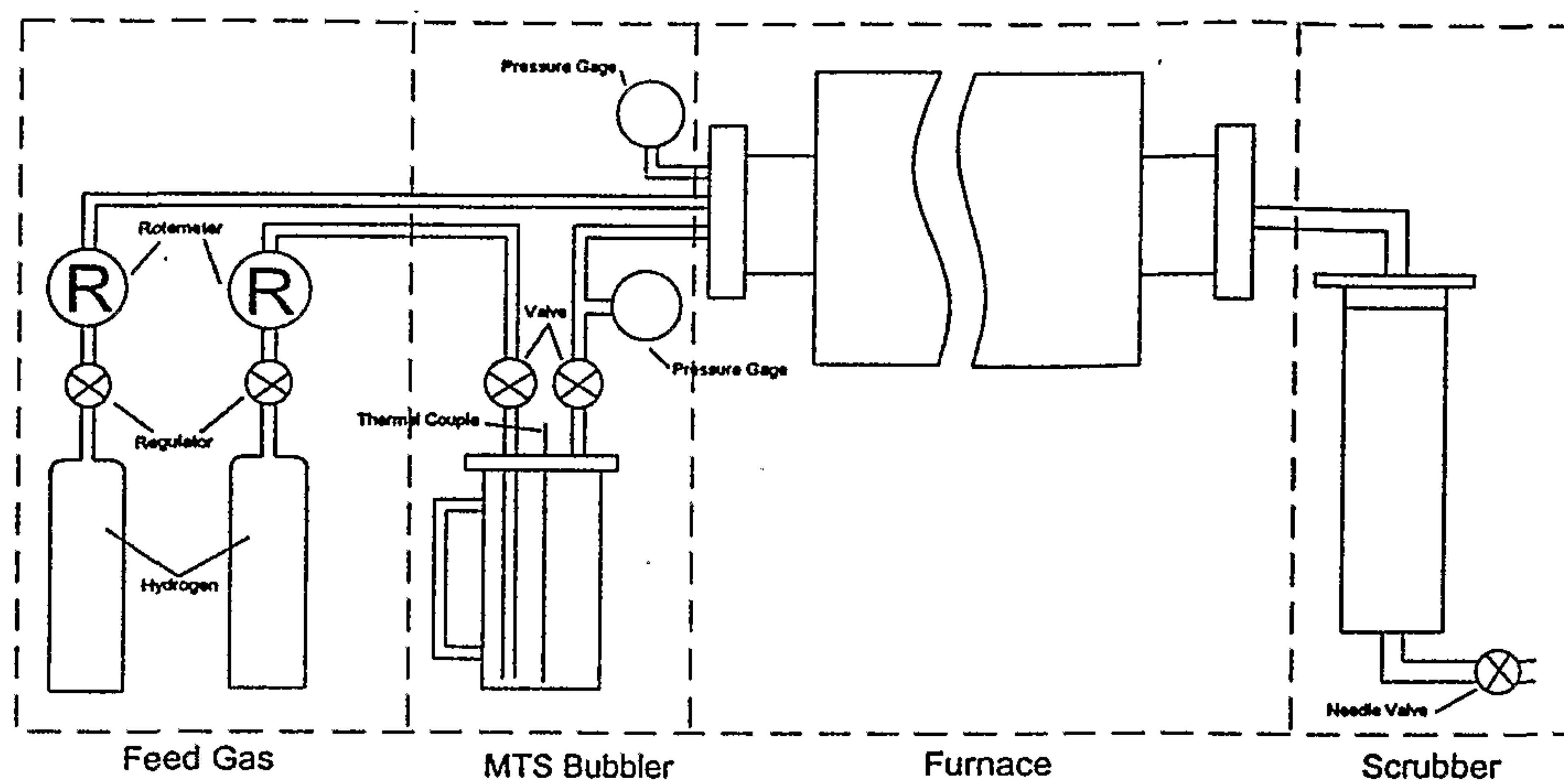
Figure 9: SiC coating equipment.
