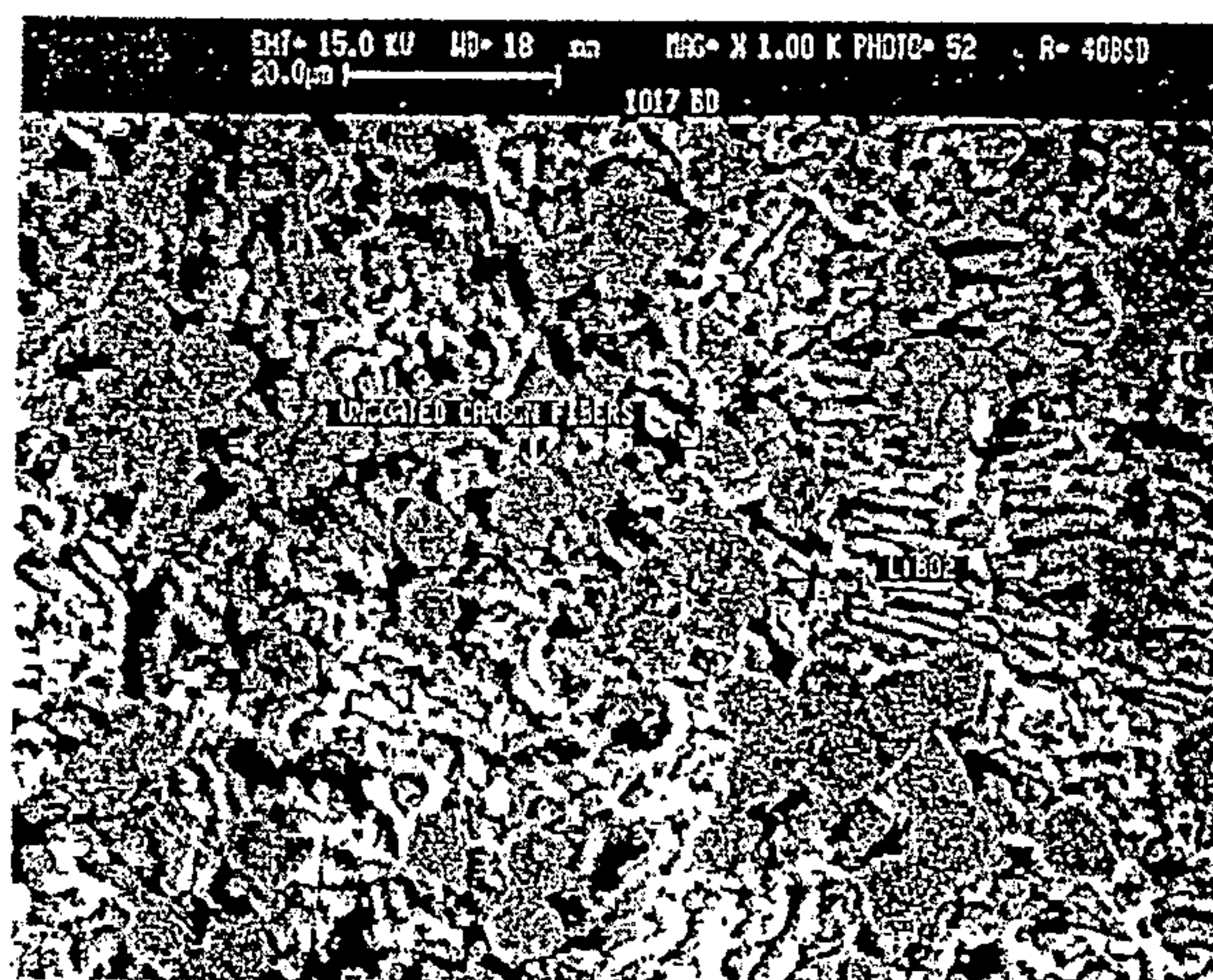
Figure 8: Post torch test SEM picture.
