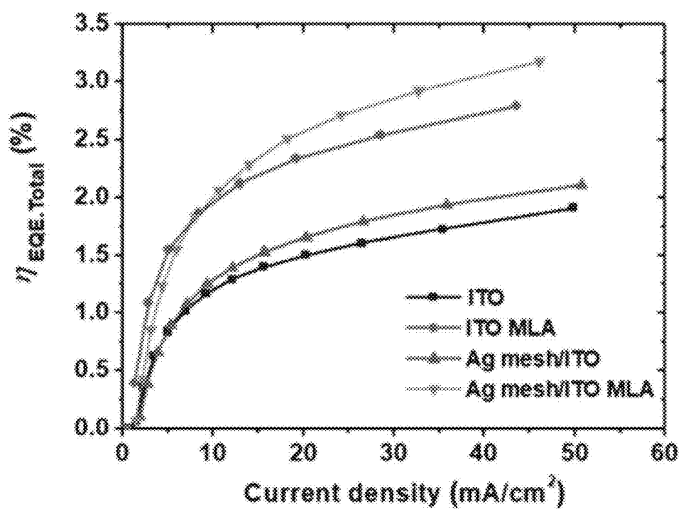
Figure 59. Plot of external quantum efficiency vs current density with different substrates.
