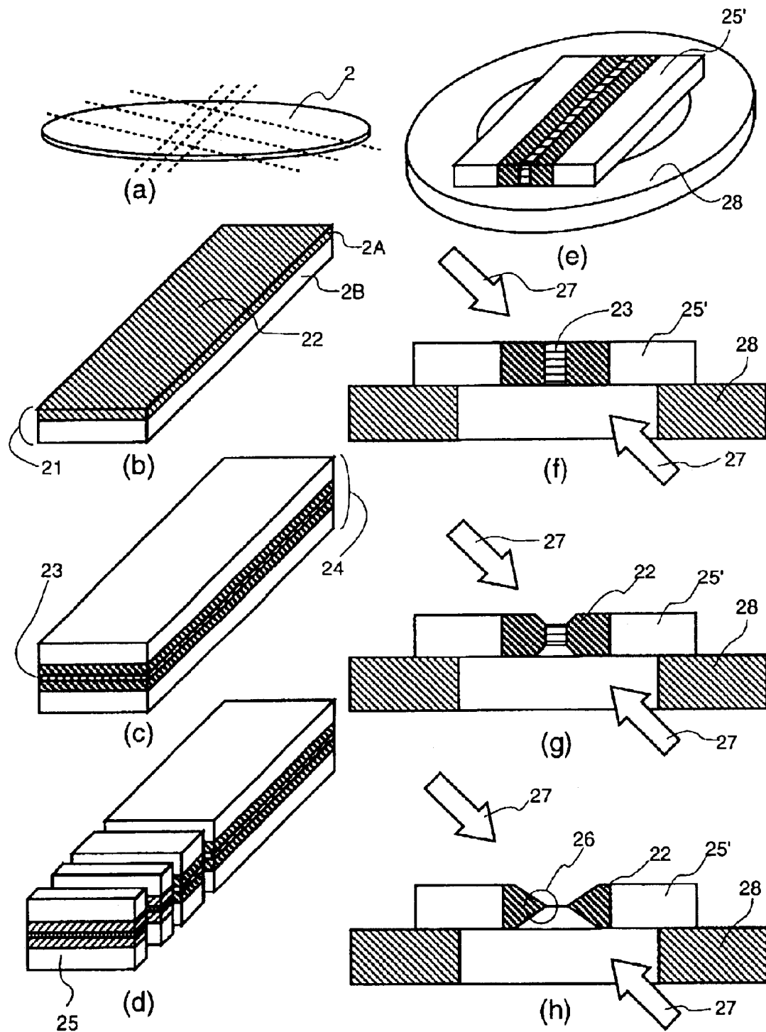
FIG.2 (PRIOR ART)
