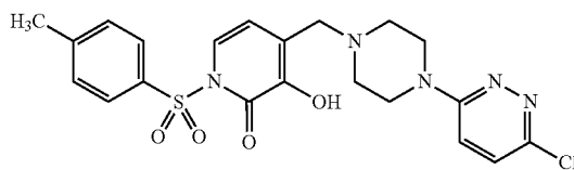
1-(4'-Methylbenzenesulfonyl)-3-hydroxy-4-[4-(6-chloropyridazin-3-yl)piperazin-1-ylmethyl]pyridin-2(1H)-one
