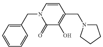
1-Benzyl-3-hydroxy-4-(pyrrolidin-1-ylmethyl)pyridin-2(1H)-one
