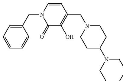
1-Benzyl-3-hydroxy-(1,4'-biperidiny-1'-ylmethyl)pyridin-2(1H)-one
