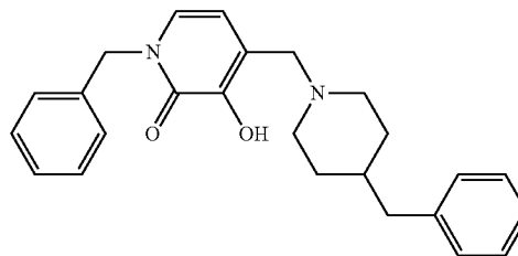
1-Benzyl-3-hydroxy-4-(4-benzylpiperidin-1-ylmethyl)pyridin-2(1H)-one
