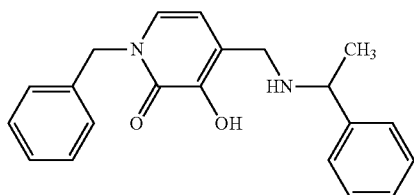
1-Benzyl-3-hydroxy-4-[(1-phenylethylamino)methyl]pyridin-2(1H)-one
