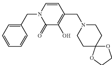
1-Benzyl-3-hydroxy-4-(1,4-dioxo-8-azaspiro[4,5]dec-8-ylmethyl)pyridin-2(1H)-one
