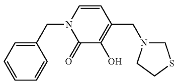
1-Benzyl-3-hydroxy-4-(thiazolidin-3-ylmethyl)pyridin-2(1H)-one
