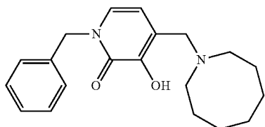
1-Benzyl-3-hydroxy-4-(azocan-1-ylmethyl)pyridin-2(1H)-one
