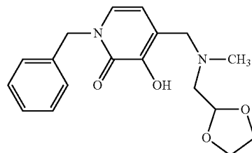
1-Benzyl-3-hydroxy-4-[[[1,3]dioxolan-2-ylmethylmethylamino]methyl]pyridin-2(1H)-one
