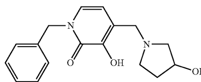
1-Benzyl-3-hydroxy-4-[(3-hydroxypyrrolidin-1-yl)methyl]pyridin-2(1H)-one
