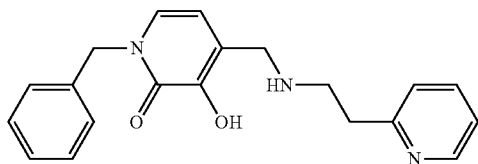
1-Benzyl-3-hydroxy-4-[(2-(pyridin-2-yl)ethylamino)methyl]pyridin-2(1H)-one
