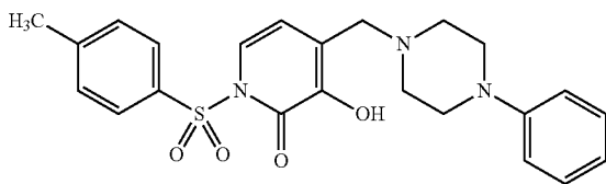
1-(4'-Methylbenzenesulfonyl)-3-hydroxy-4-(4-phenylpiperazin-1-ylmethyl)-pyridin-2(1H)-one
