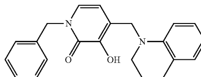
1-Benzyl-3-hydroxy-4-[(3,4-dihydroquinolin-1(2H)-yl)methyl]pyridin-2(1H)-one
