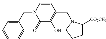
Methyl 1-[(1-benzyl-3-hydroxy-2-oxo-1,2-dihydropyridin-4-yl)methyl]pyrrolidine-2-carboxylate
