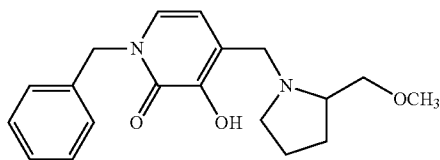
1-benzyl-3-hydroxy-4-{[2-(methoxymethyl)pyrrolidin-1-yl]methyl}pyridin-2(1H)-one
