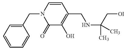
1-Benzyl-3-hydroxy-4-[(1-hydroxy-2-methylpropan-2-ylamino)methyl]pyridin-2(1H)-one
