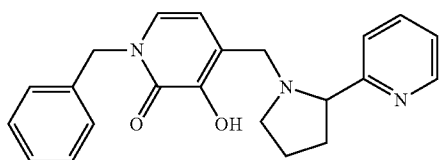
1-Benzyl-3-hydroxy-4-{[2-(pyridin-2-yl)pyrrolidin-1-yl]methyl}pyridin-2(1H)-one
