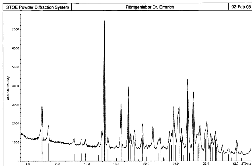
Figure 5: XRPD pattern of crystalline (E)-N-(2-amino-phenyl)-3-{1-[4-(1-methyl-1H-pyrazol-4-yl)-benzenesulfonyl]-1H-pyrrol-3-yl}-acrylamide dihydrochloride
