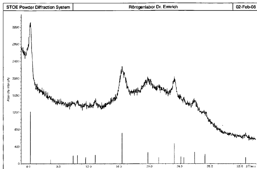
Figure 1: XRPD pattern of partially amorphous (E)-N-(2-amino-phenyl)-3-{1-[4-(1-methyl-1H-pyrazol-4-yl)-benzenesulfonyl]-1H-pyrrol-3-yl}-acrylamide
