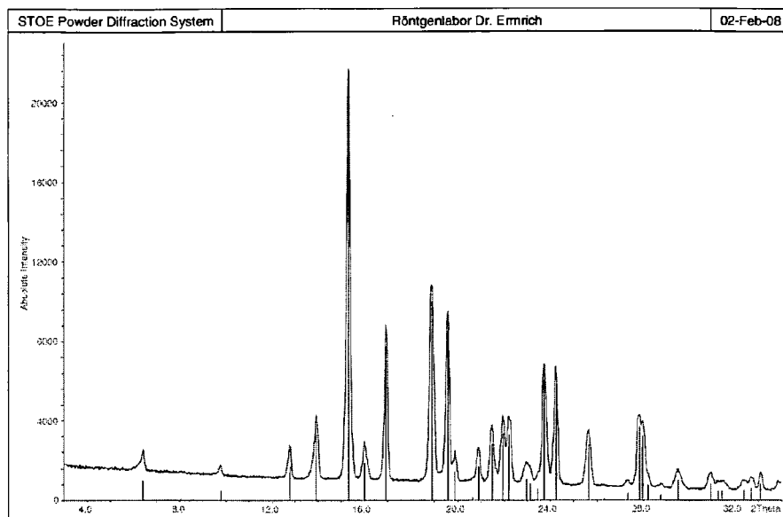
Figure 3: XRPD pattern of crystalline (E)-N-(2-amino-phenyl)-3-{1-[4-(1-methyl-1H-pyrazol-4-yl)-benzenesulfonyl]-1H-pyrrol-3-yl}-acrylamide polymorph B
