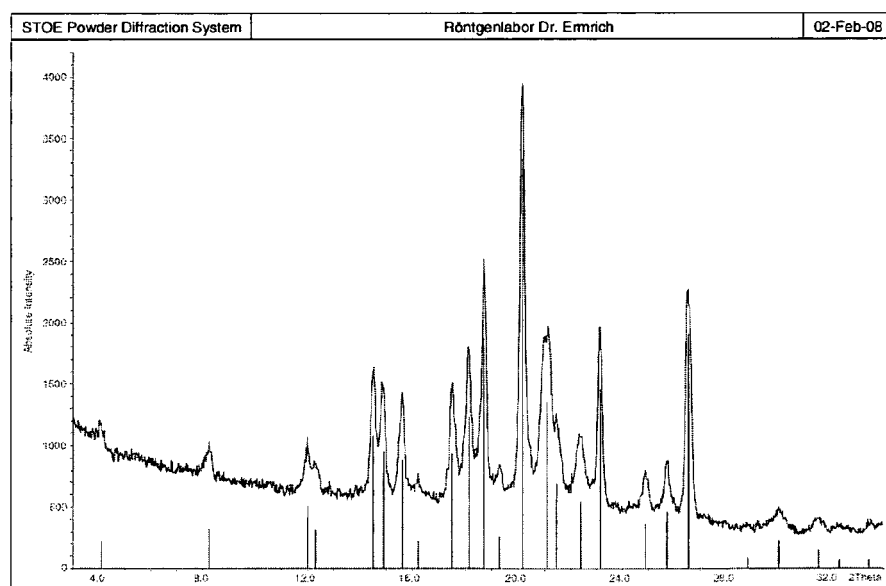
Figure 2: XRPD pattern of crystalline (E)-N-(2-amino-phenyl)-3-{1-[4-(1-methyl-1H-pyrazol-4-yl)-benzenesulfonyl]-1H-pyrrol-3-yl}-acrylamide polymorph A
