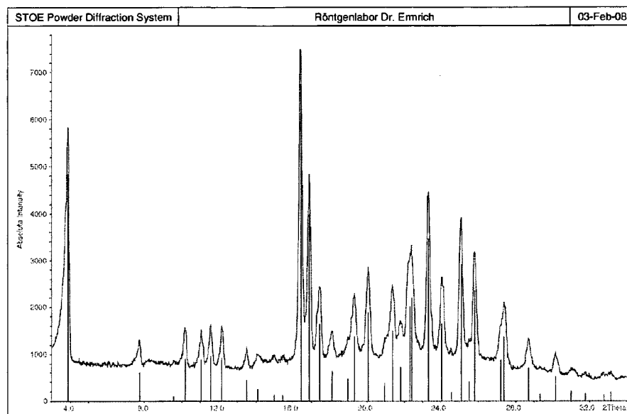
Figure 7: XRPD pattern of crystalline (E)-N-(2-amino-phenyl)-3-{1-[4-(1-methyl-1H-pyrazol-4-yl)-benzenesulfonyl]-1H-pyrrol-3-yl}-acrylamide methanesulfonate
