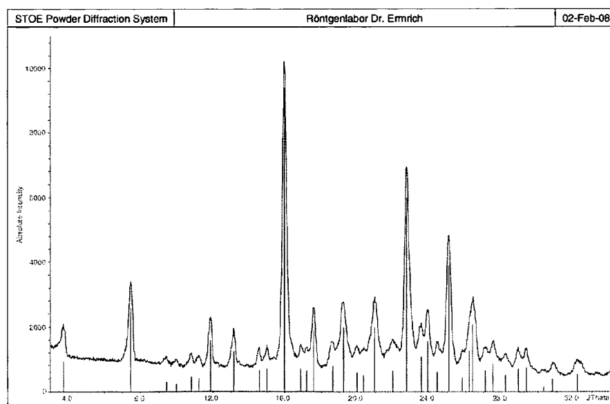
Figure 8: XRPD pattern of (E)-N-(2-amino-phenyl)-3-{1-[4-(1-methyl-1H-pyrazol-4-yl)-benzenesulfonyl]-1H-pyrrol-3-yl}-acrylamide hemi ethane-1,2-sulfonate
