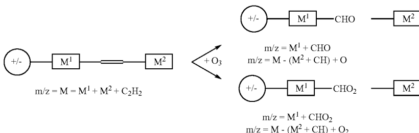
Scheme 2: General scheme applicable to any unsaturated compound comprising carbon-carbon double bonds, detailing the fragments obtained following reaction of mass-selected ions with ozone, and the determination of double bond position based on the mass of fragments on each side of the double bond.
