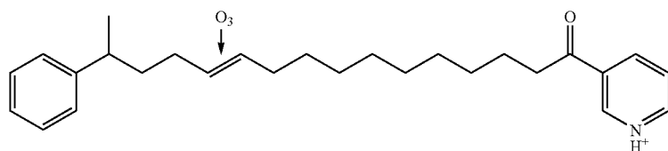
Scheme 4: Determination of double bond position in an unsaturated compound based on the mass of fragments on each side of the double bond, as calculated from fragments obtained following ozone induced dissociation of a mass-selected ion.
