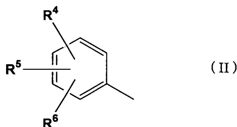
[Chemical formula 2]
