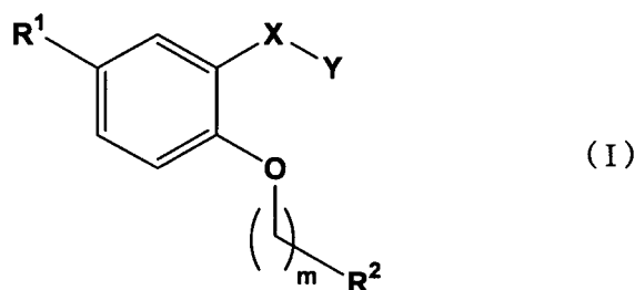
[Chemical formula 1]
