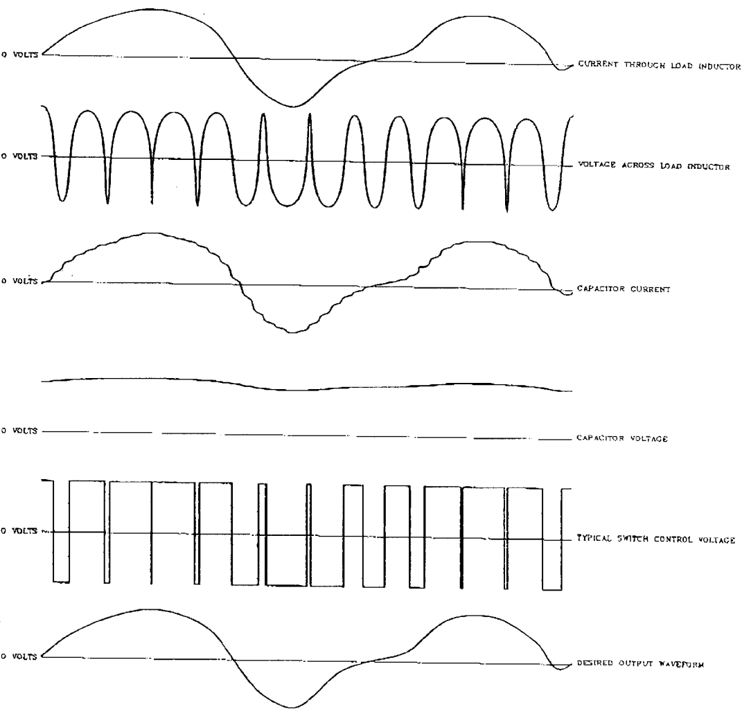
FIGURE 4-3 SWITCHED CAPACITOR CIRCUIT WAVEFORMS
