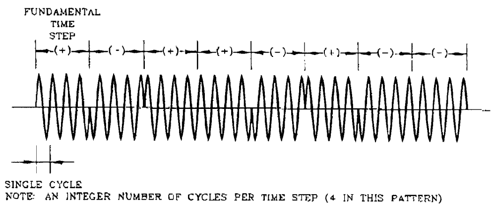
FIGURE 1-10 AN 8 SECTION (+ - + + ~ + - -) TIME ENCODED WAVEFORM
