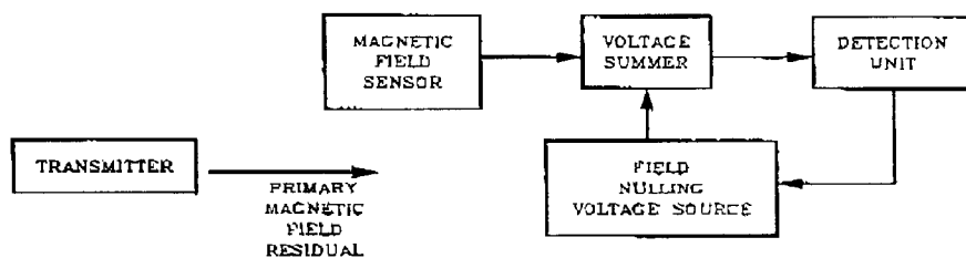
FIGURE 1-4B VOLTAGE NULLING OF RESIDUAL FIELD SENSOR OUTPUT
