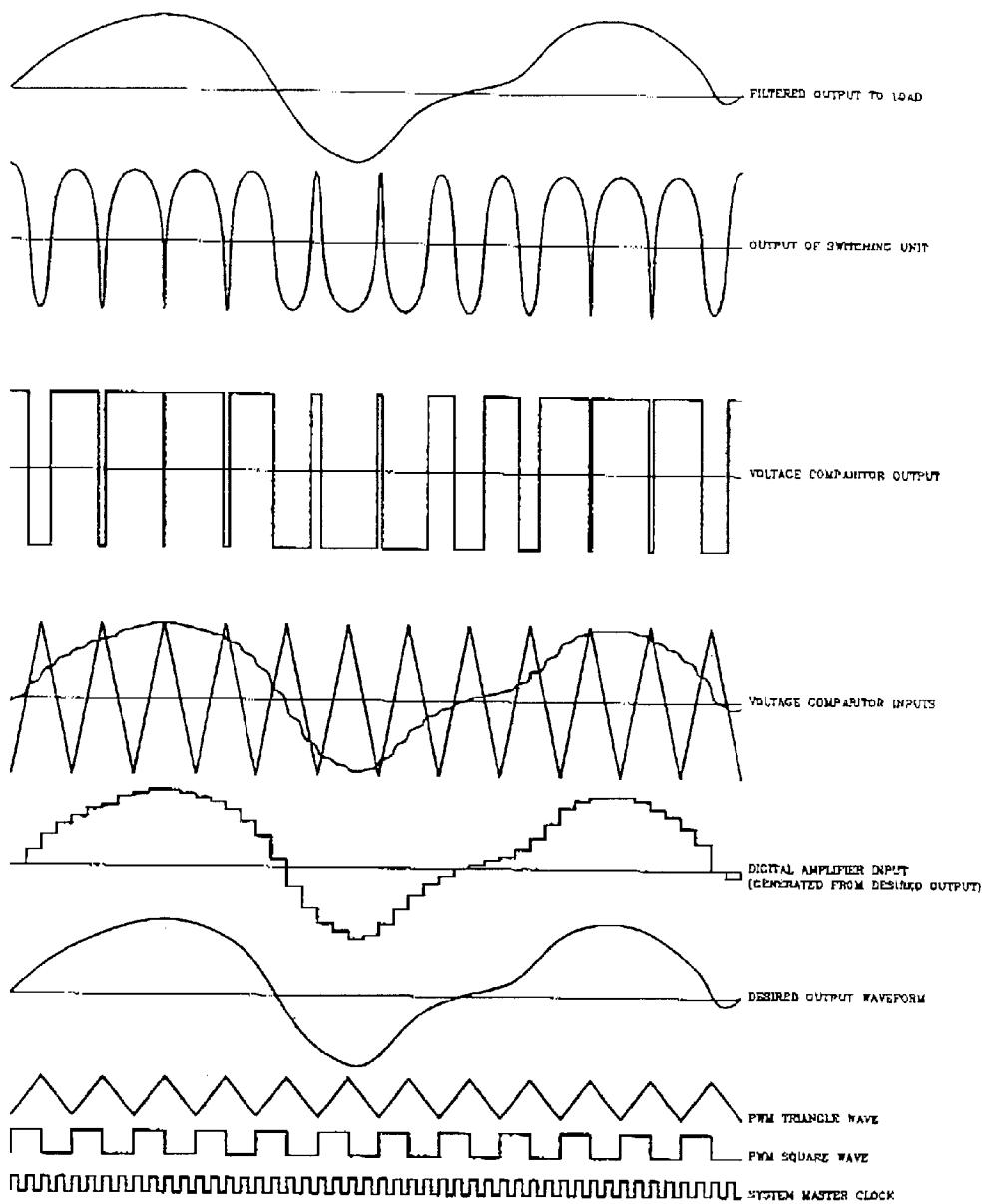
FIGURE 2-2 TYPICAL PULSE WIDTH MODULATION WAVEFORMS
