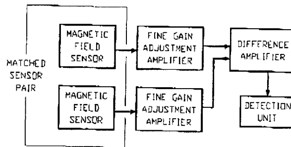
FIGURE 1-6 GRADIENT SENSING USING A MATCHED SENSOR PAIR
