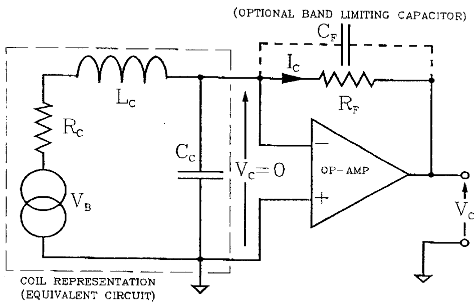
FIGURE 5-2 OPERATIONAL AMPLIFIER BASED VOLTAGE TO CURRENT CONVERSION CIRCUIT
