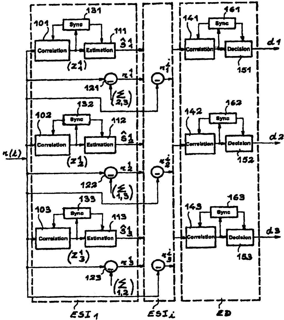
FIG. 7 - PRIOR ART -
