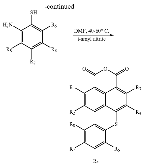
Scheme 1. Synthesis of benzo[k,l] thioxanthene-3,4-dicarboxylic anhydride
