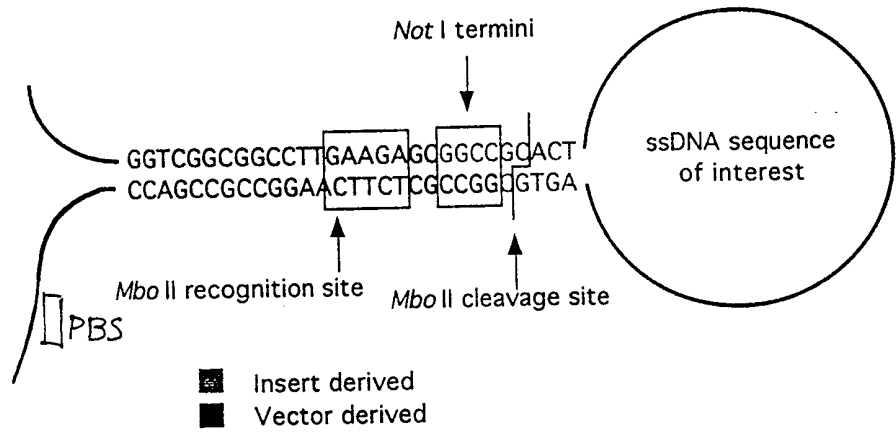
Stem-loop structure formed by single-stranded DNA.
