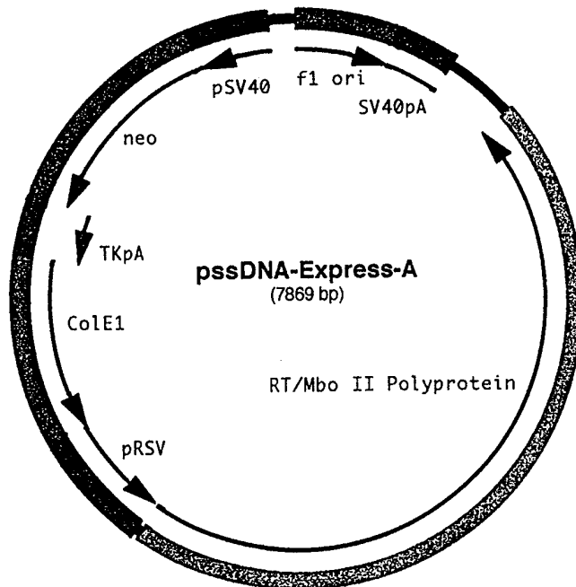
Structure of the pssDNA-Express-A plasmid. The plasmid was constructed by inserting sequences encoding a reverse transcriptase- Mbo II polyprotein (red) between the Nhe I and Xma I sites of the eukaryotic expression vector pBK-RSV (Stratagene; green, blue and black regions). The RT and Mbo II domains are separated by a short, proline-rich spacer.
