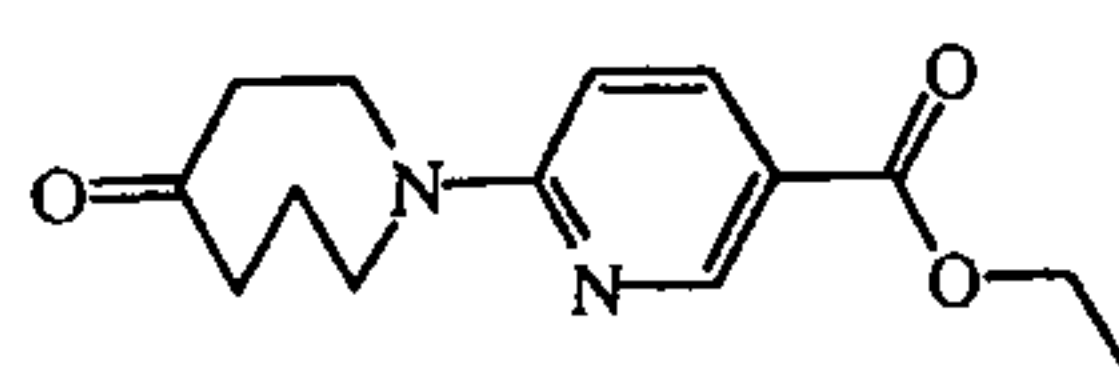
intermediate 23
