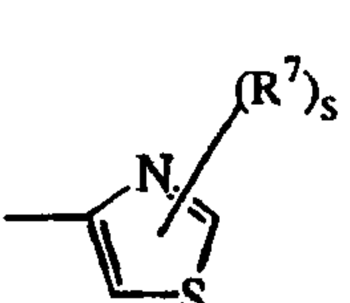
(a-15)
