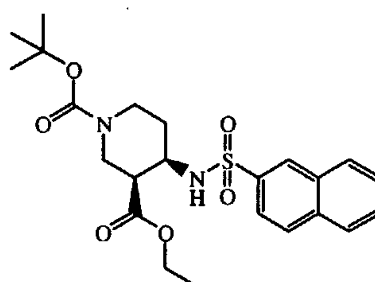
CIS intermediate 15
