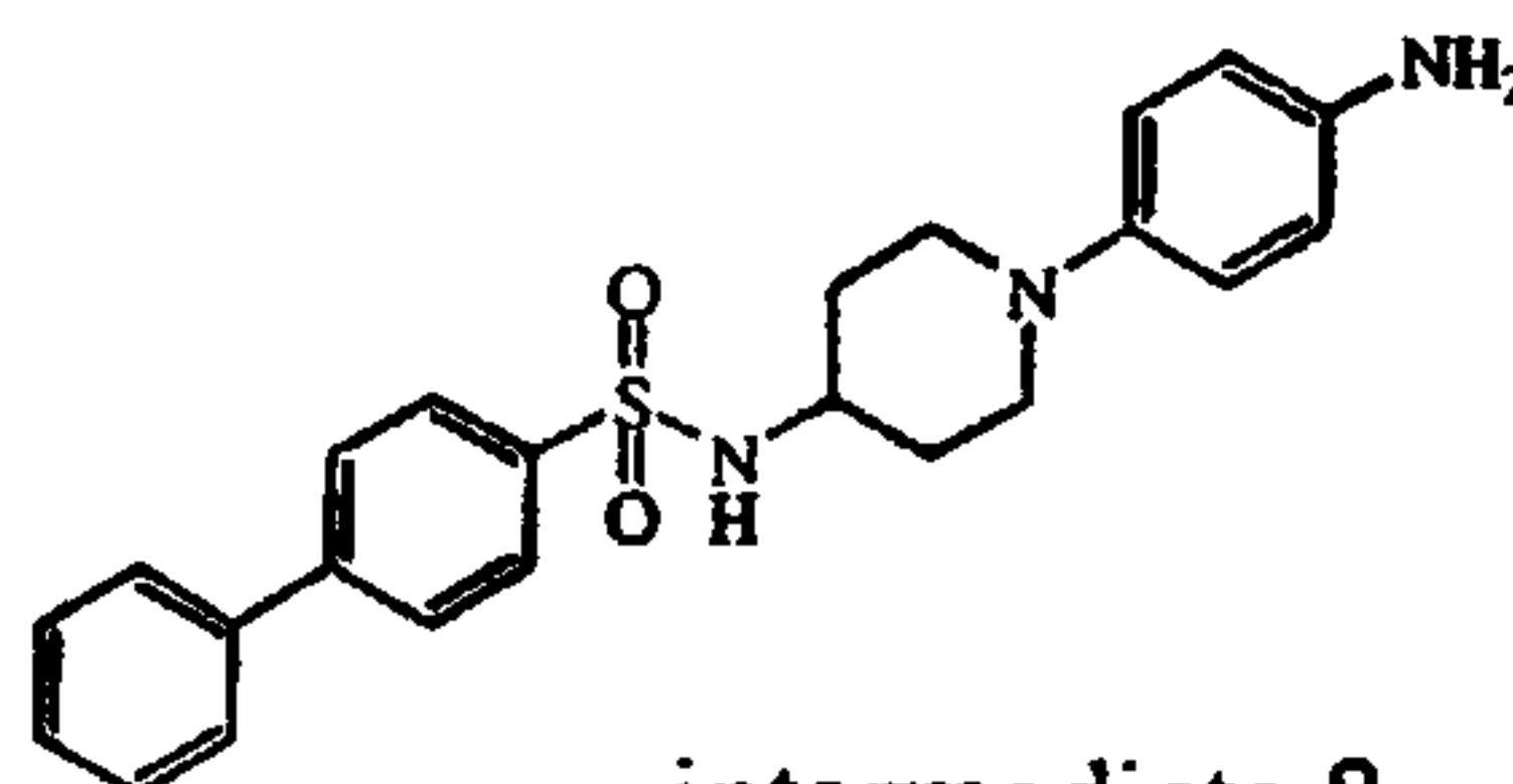
intermediate 8
