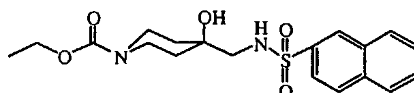
intermediate 20
