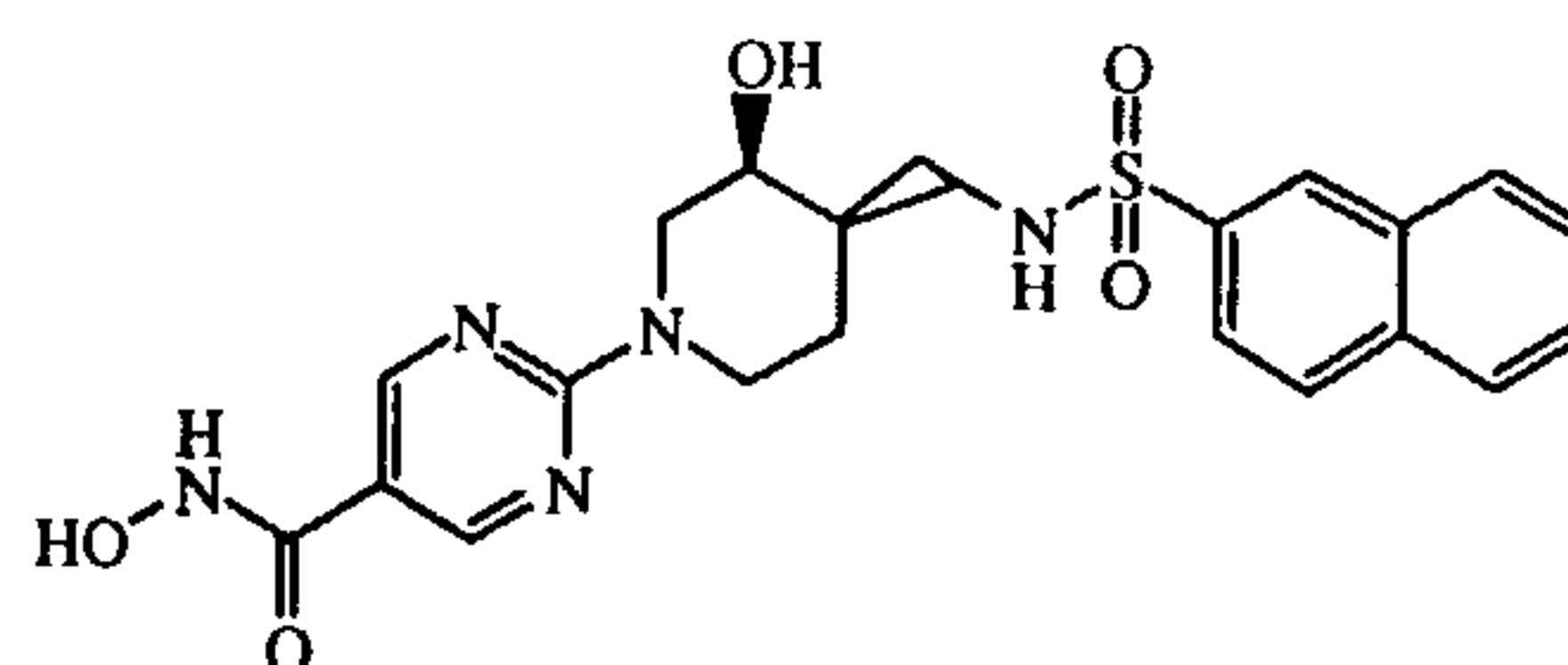
(3S-TRANS) compound 8
