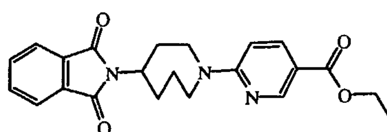
intermediate 25
