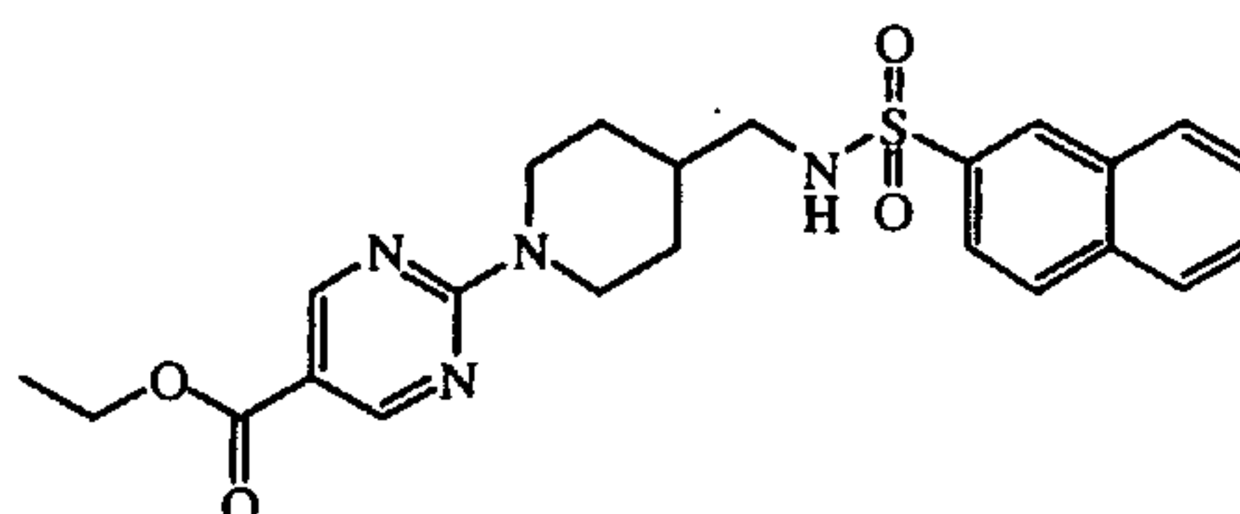
intermediate 31
