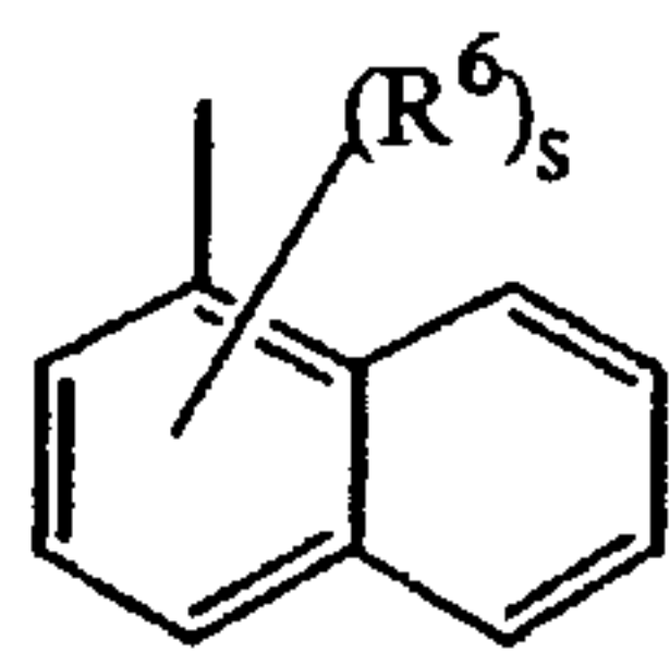
(a-21)
