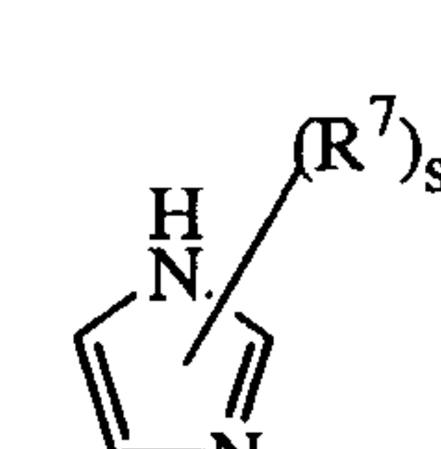
(a-14)
