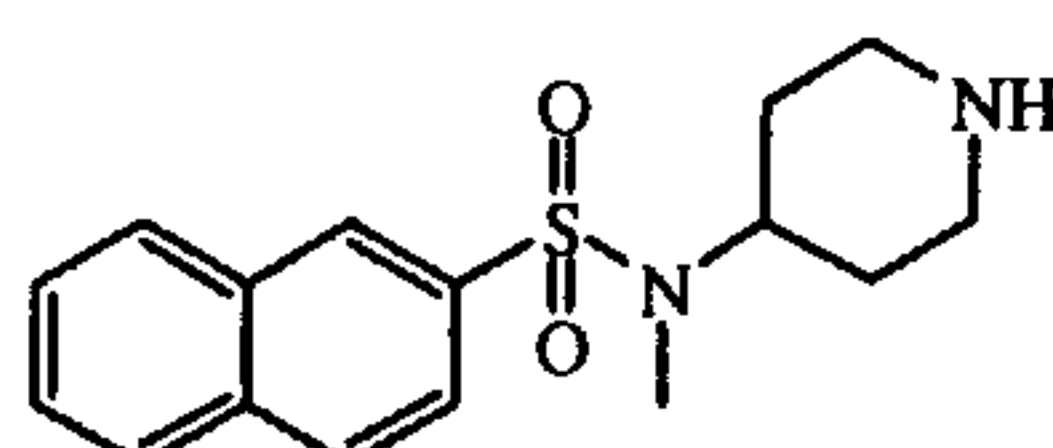
intermediate 47
