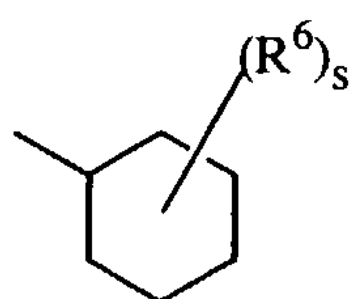
(a-2)
