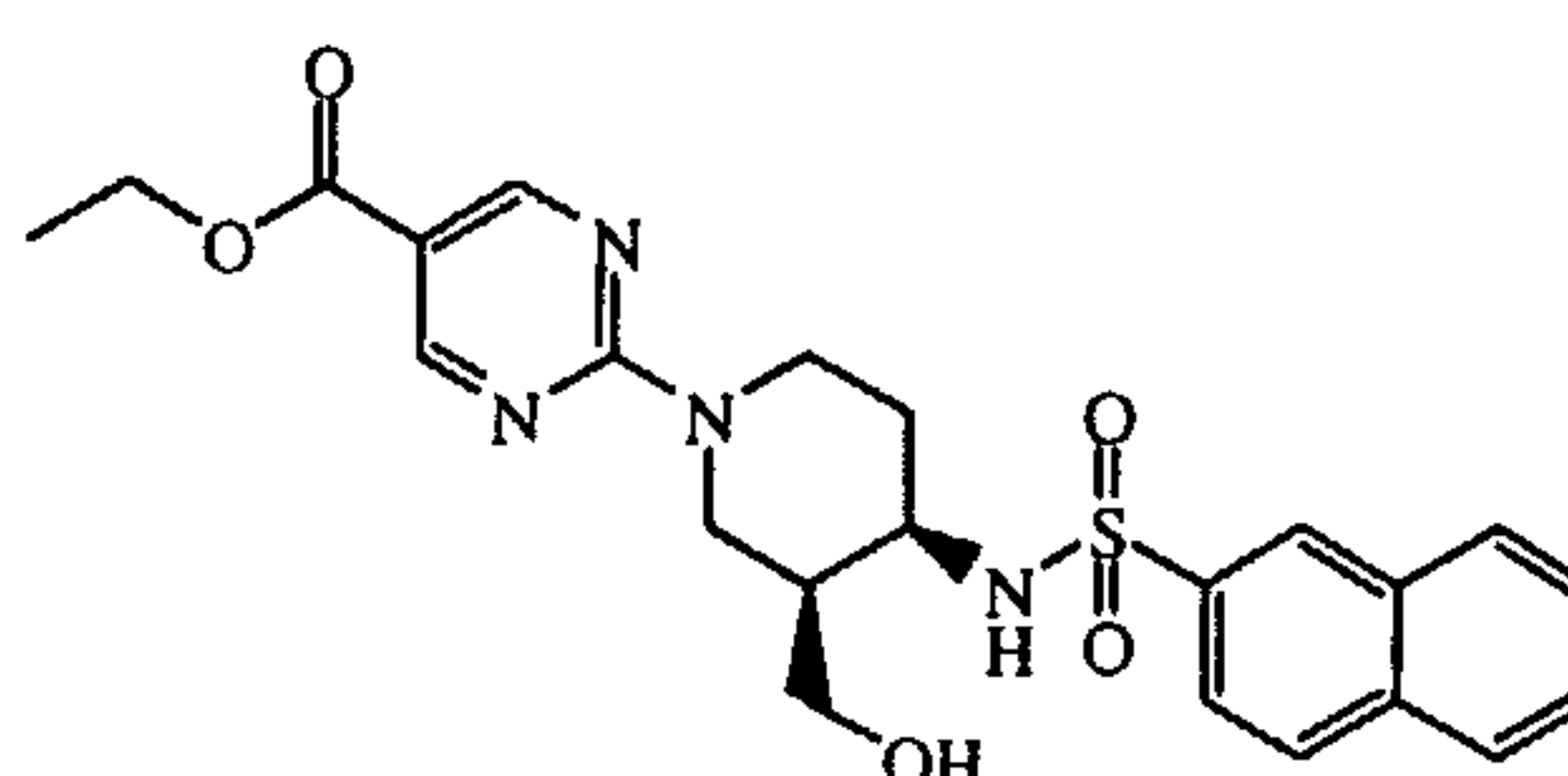
CIS intermediate 33
