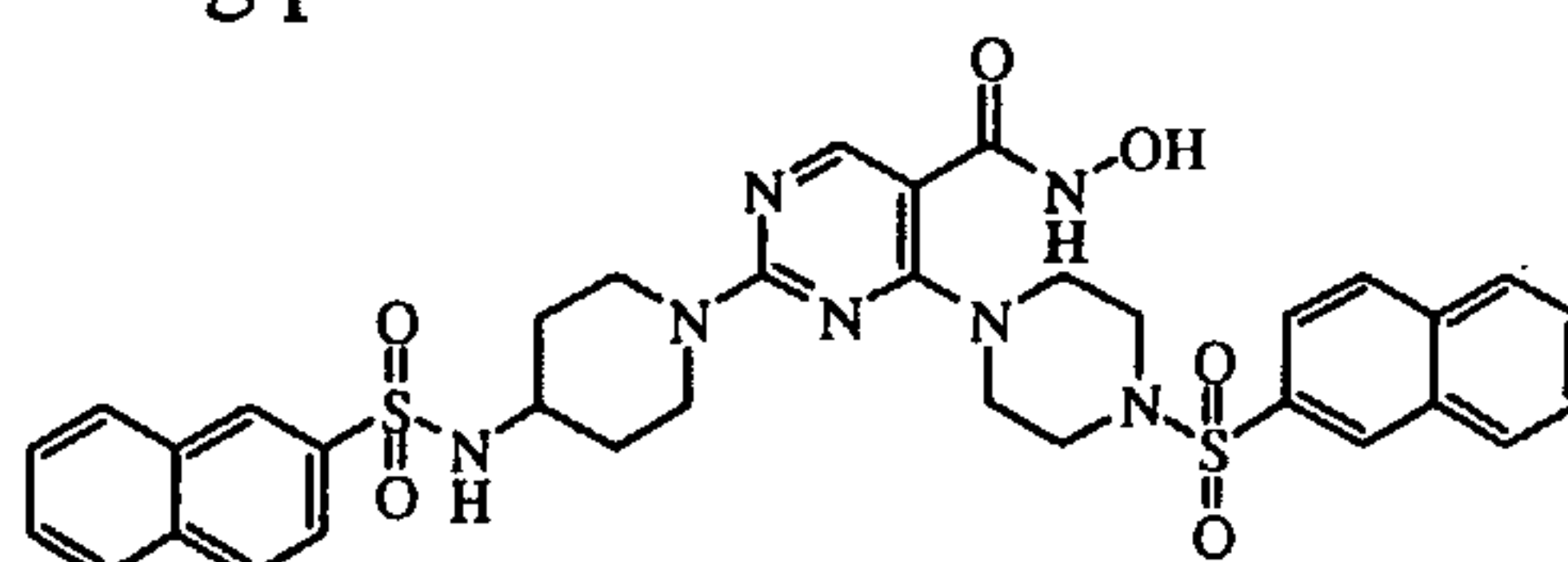
trifluoroacetate (1:1) compound 6
