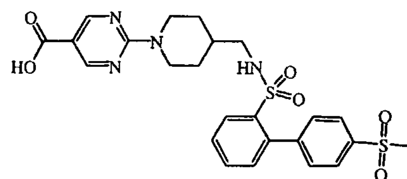
intermediate 50
