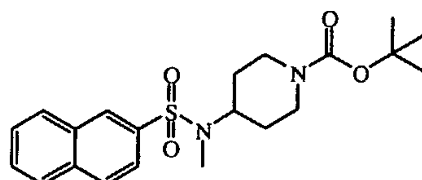
intermediate 46
