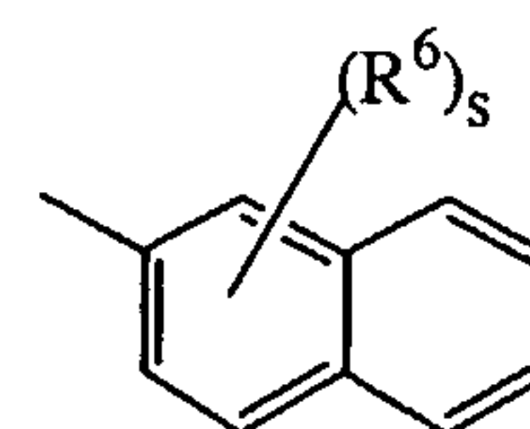
(a-20)
