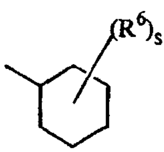
(a-2)
