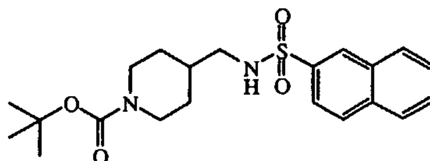
intermediate 10
