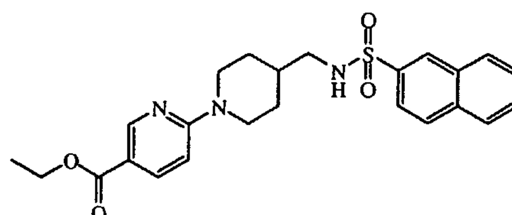
intermediate 12
