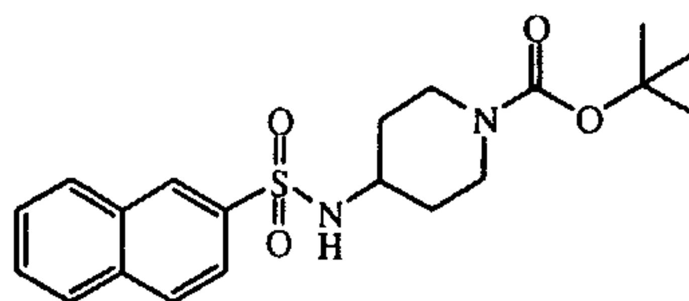
intermediate 45
