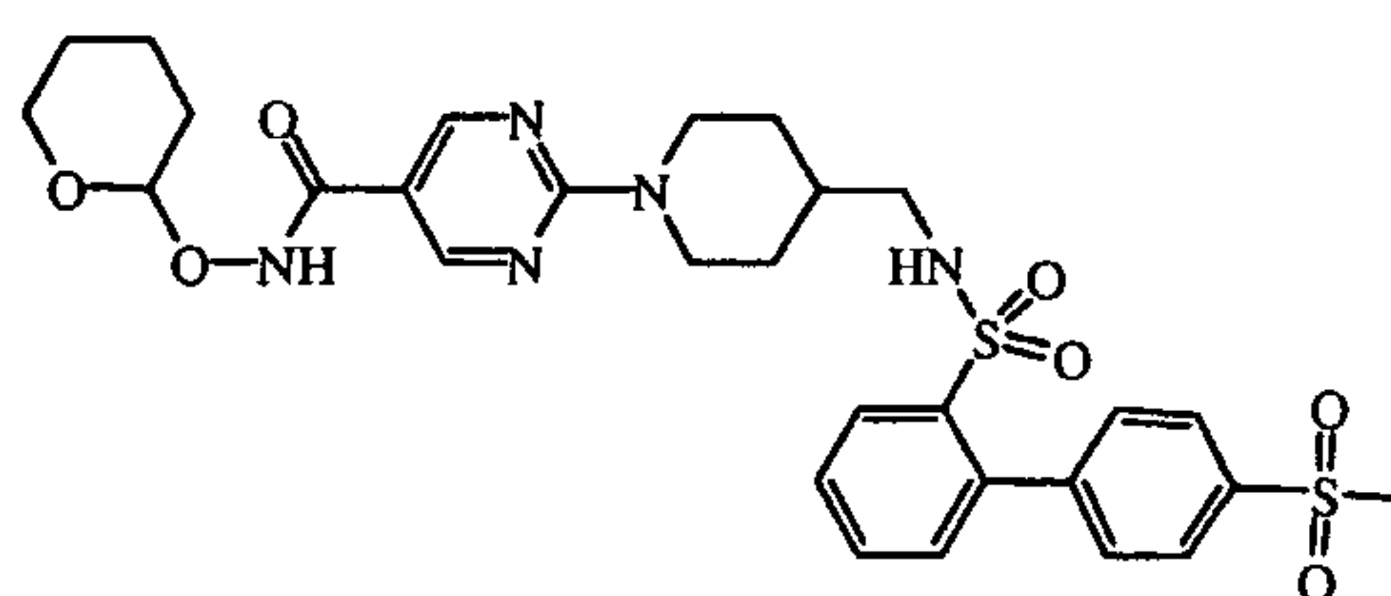
intermediate 51
