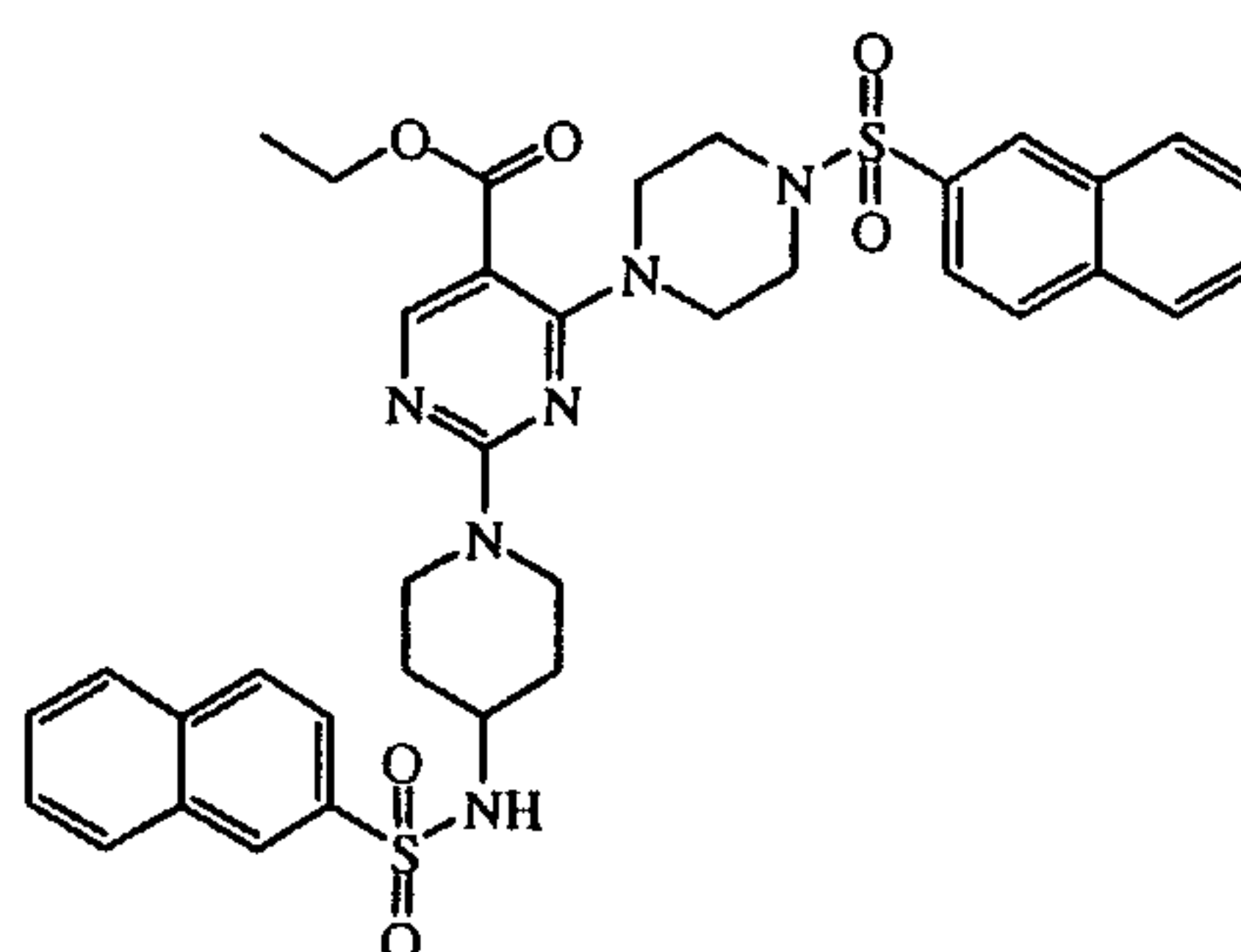
intermediate 32
