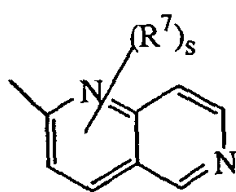
(a-25)
