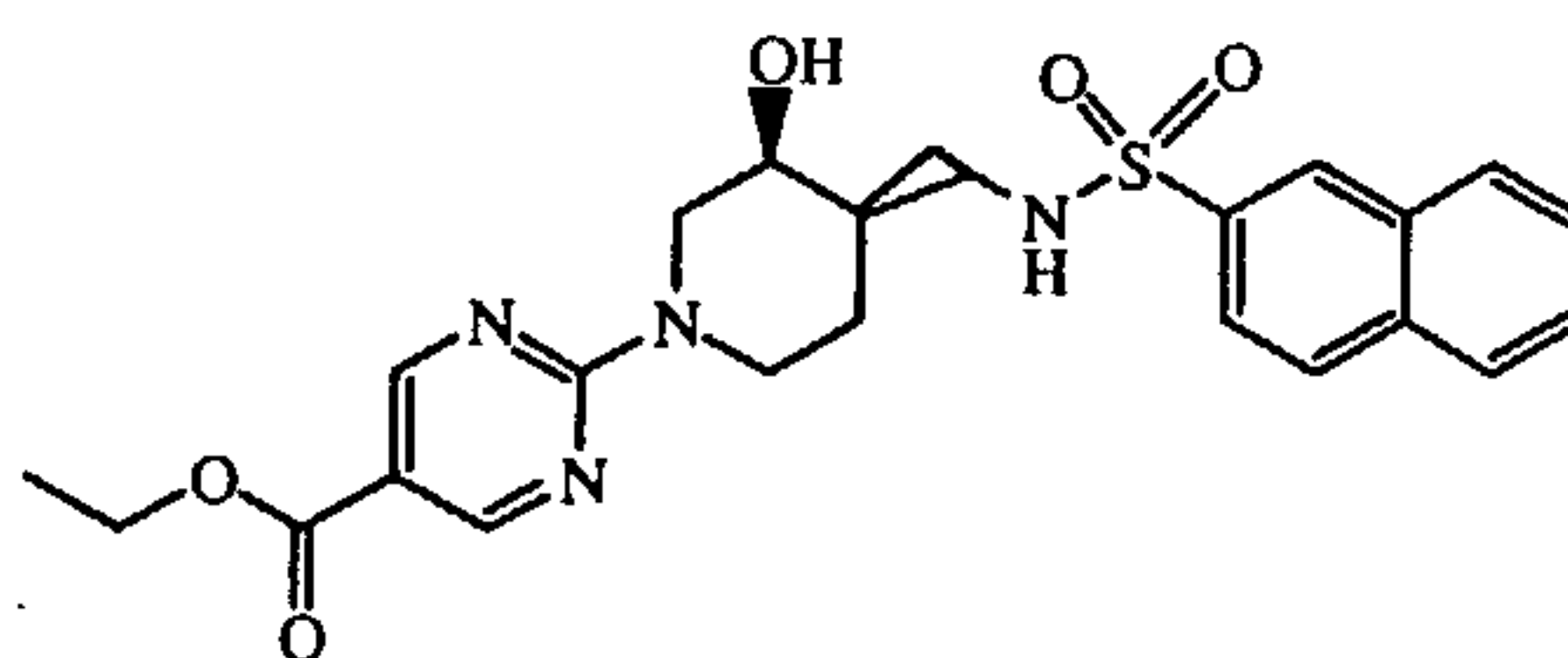
(3S-TRANS) intermediate 34
