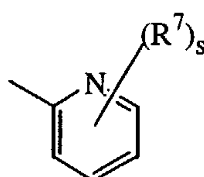
(a-3)
