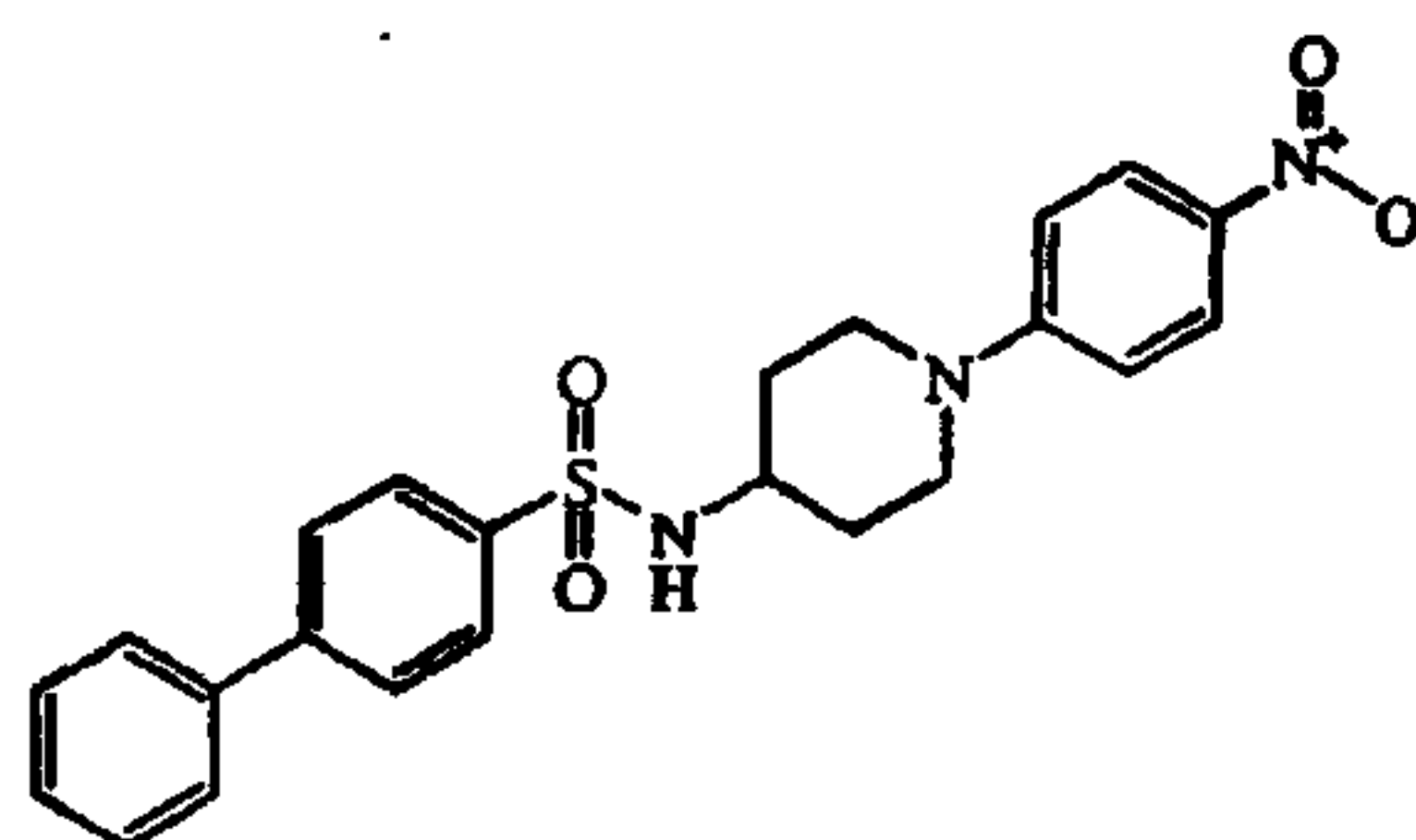
intermediate 7
