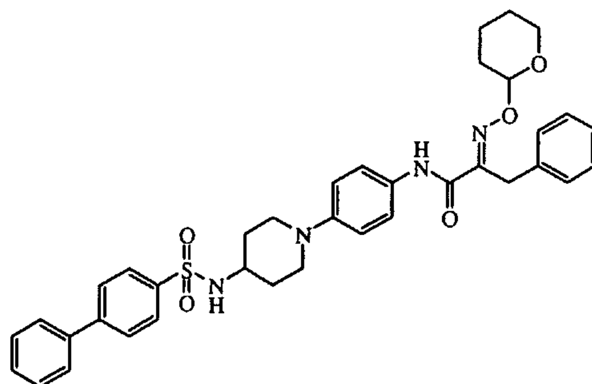
intermediate 9
