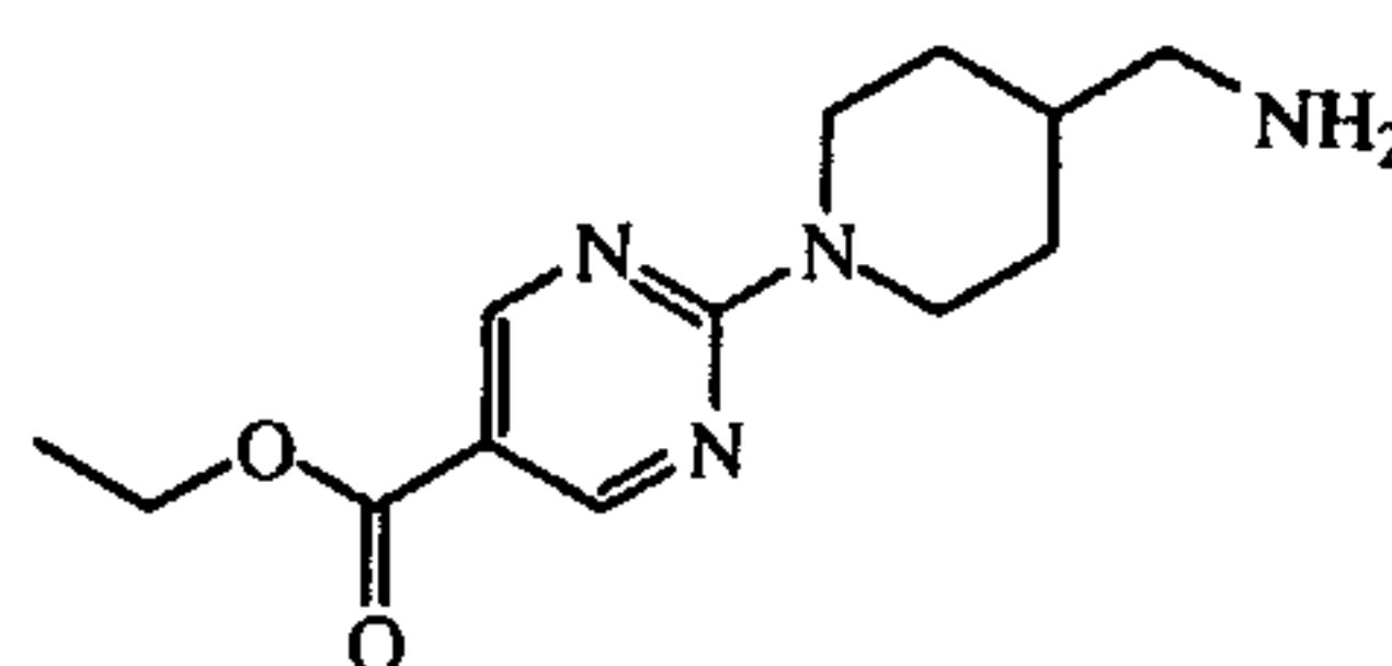
intermediate 44
