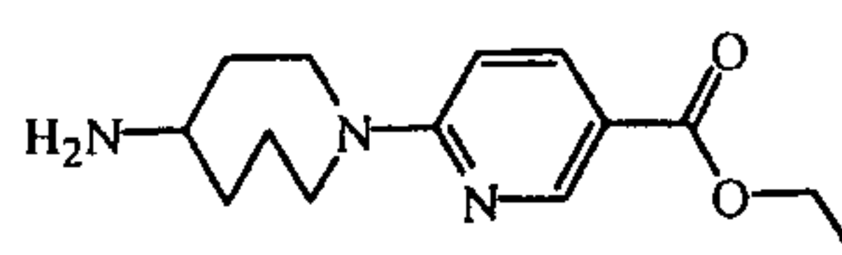
intermediate 26
