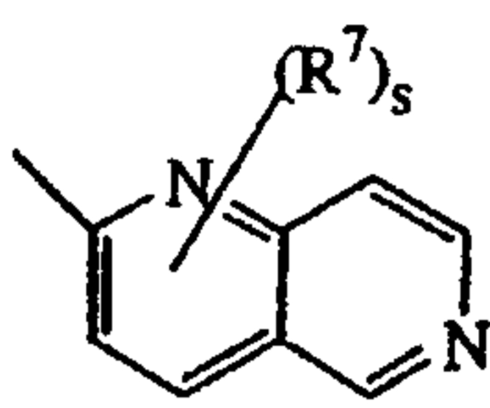
(a-25)
