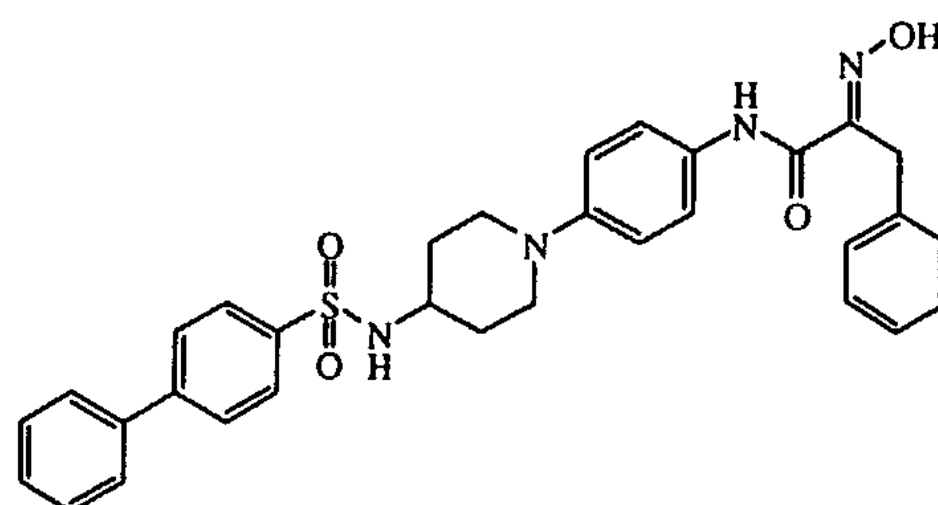
compound 3
