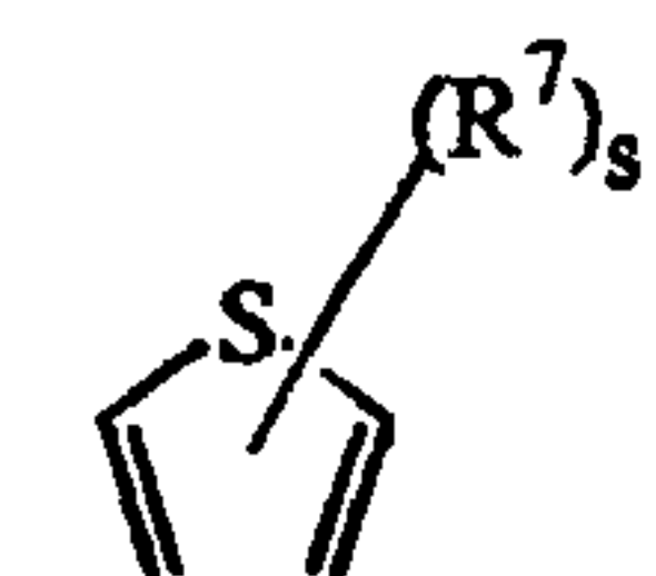
(a-10)
