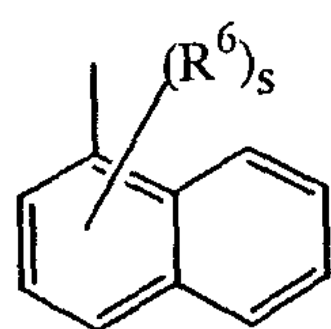
(a-21)
