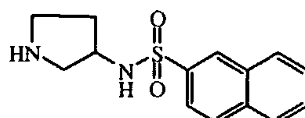
intermediate 42
