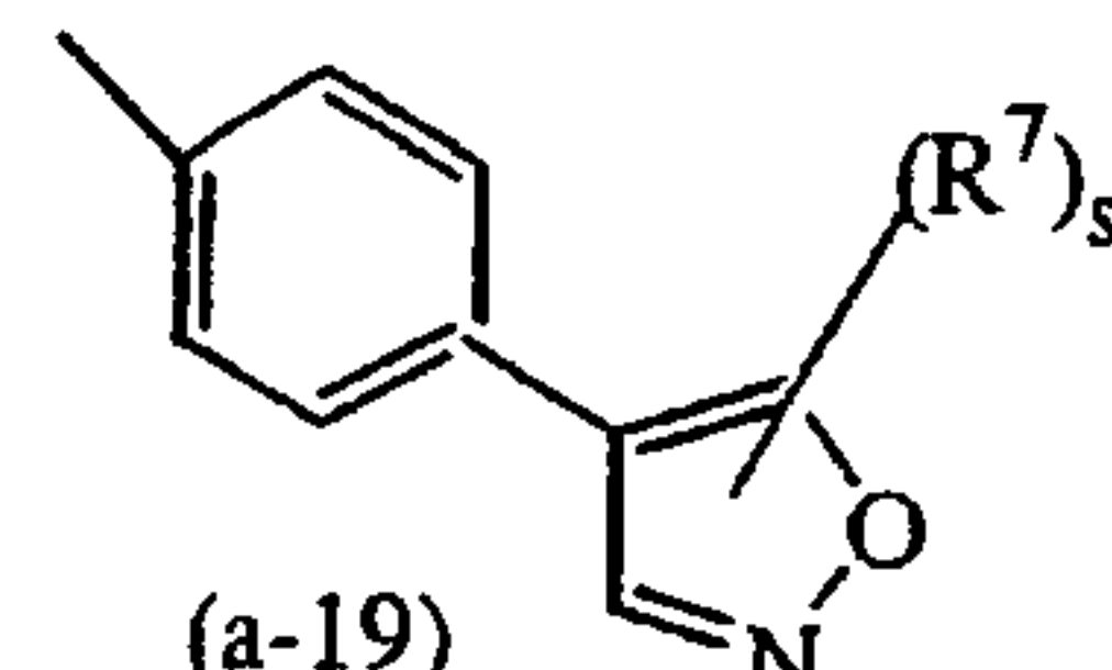
(a-19)
