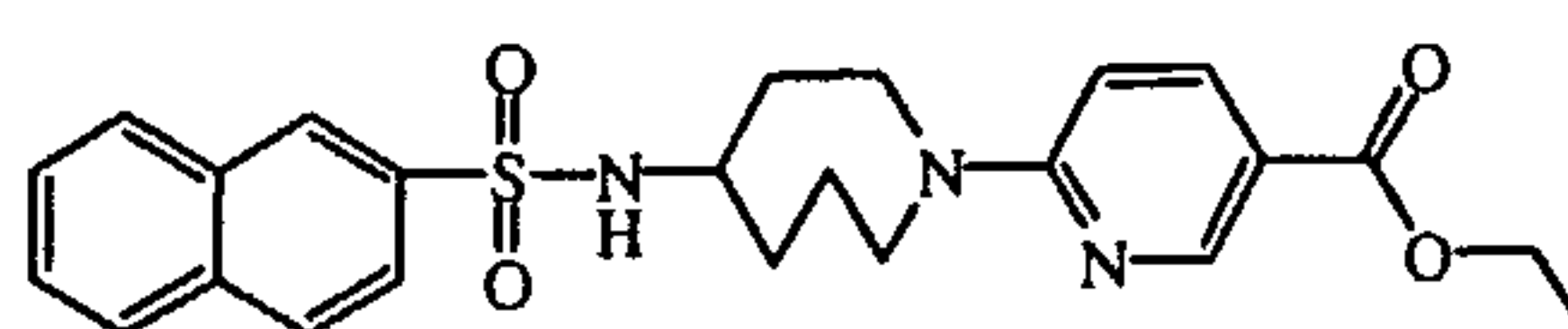
intermediate 36
