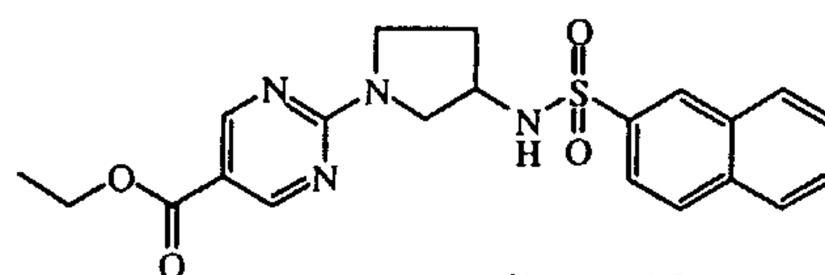
intermediate 43
