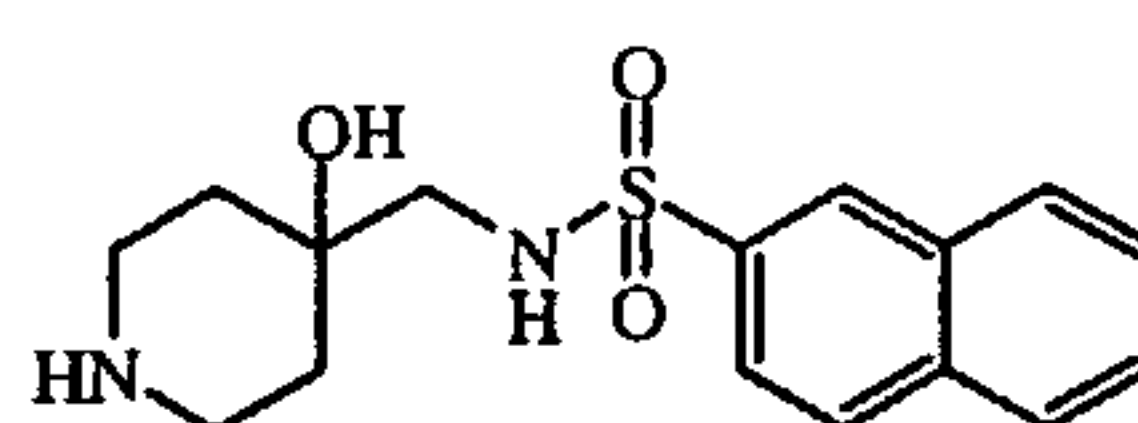
intermediate 21
