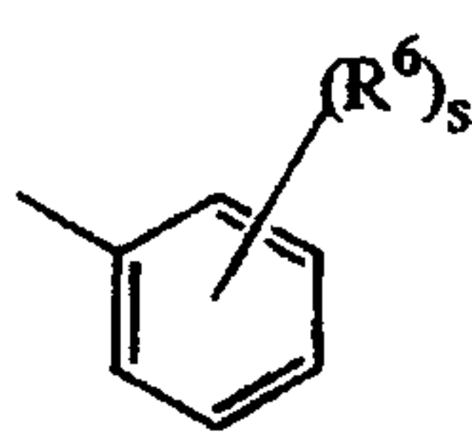
(a-1)
