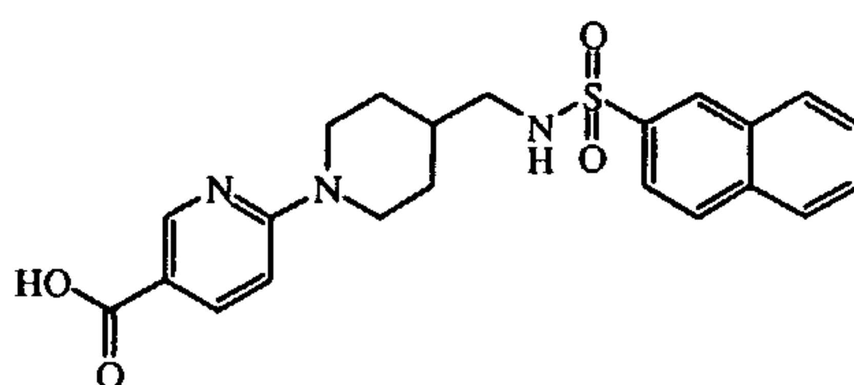
Sodium salt intermediate 29
