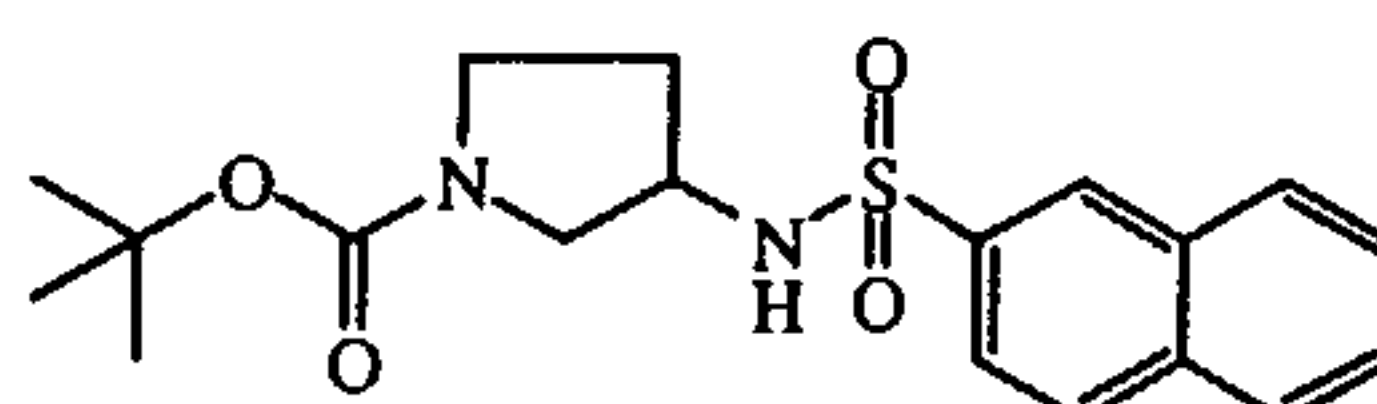
intermediate 41
