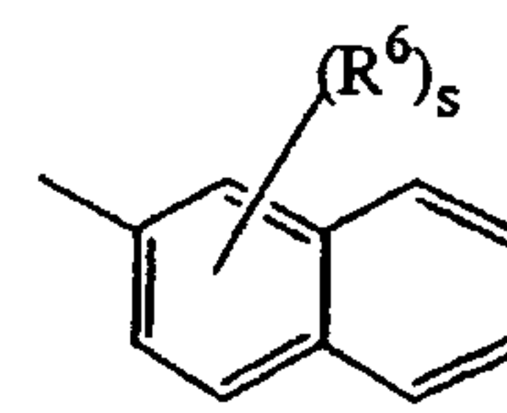
(a-20)
