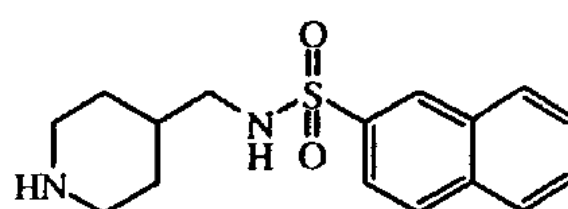
intermediate 11
