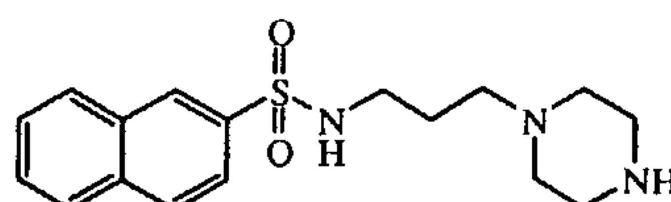
.HCl intermediate 40
