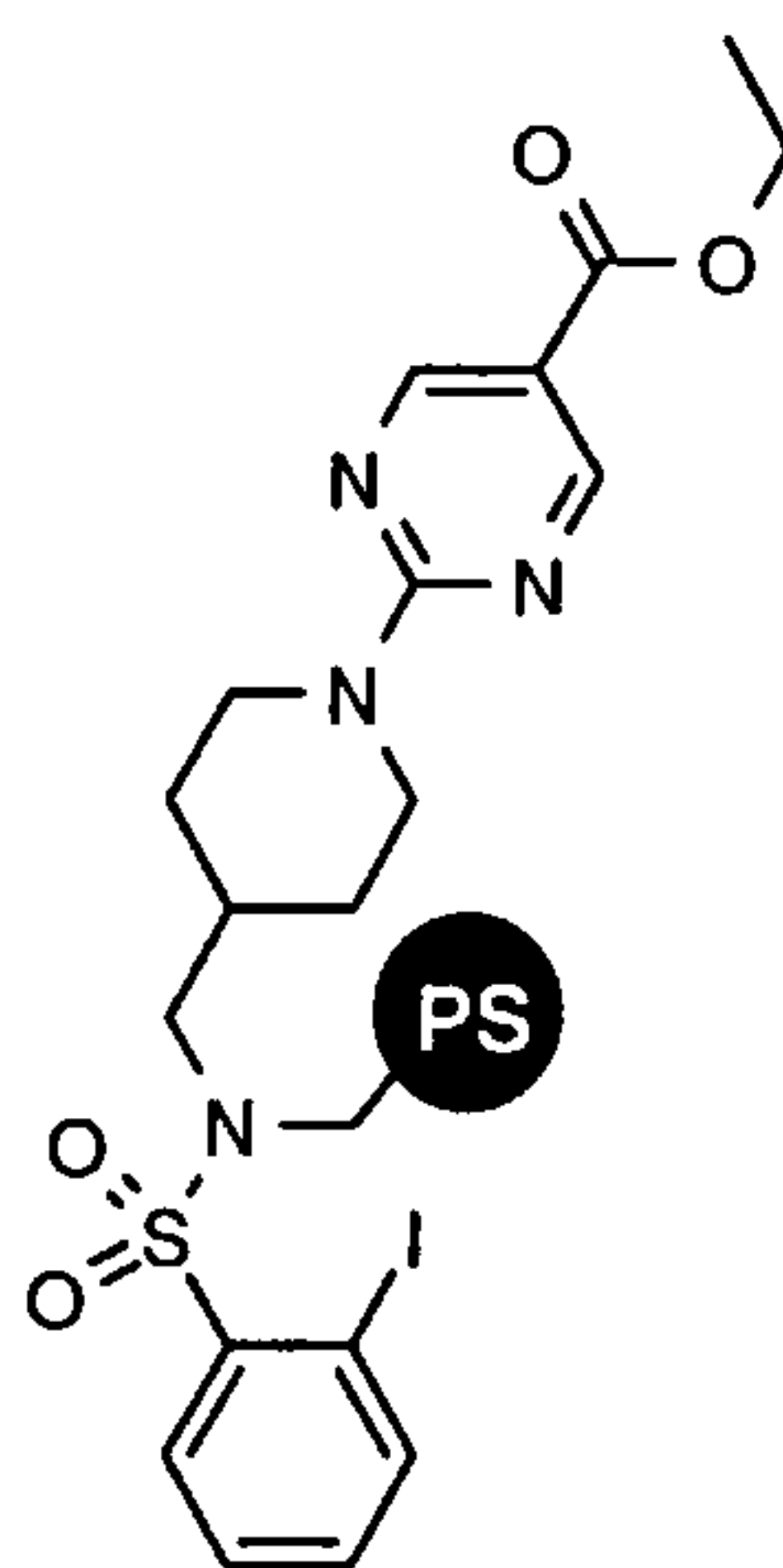
intermediate 49
