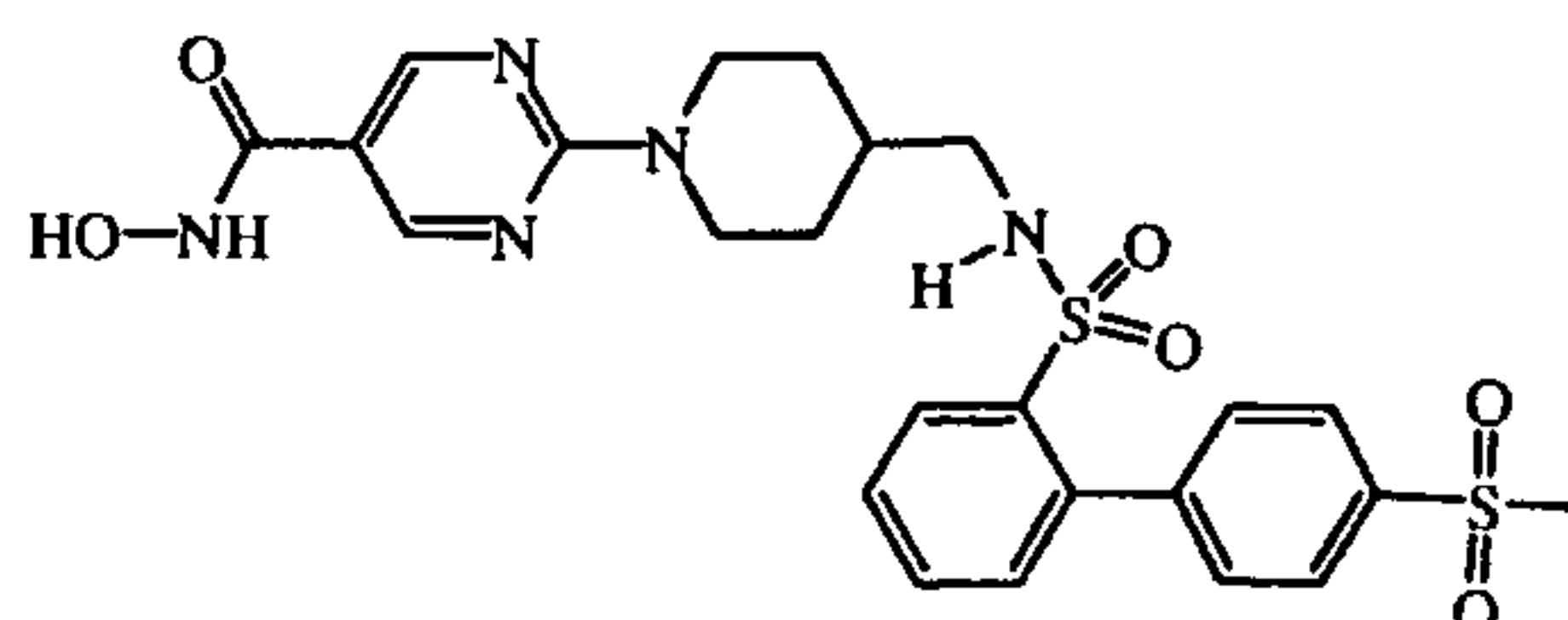
compound 30
