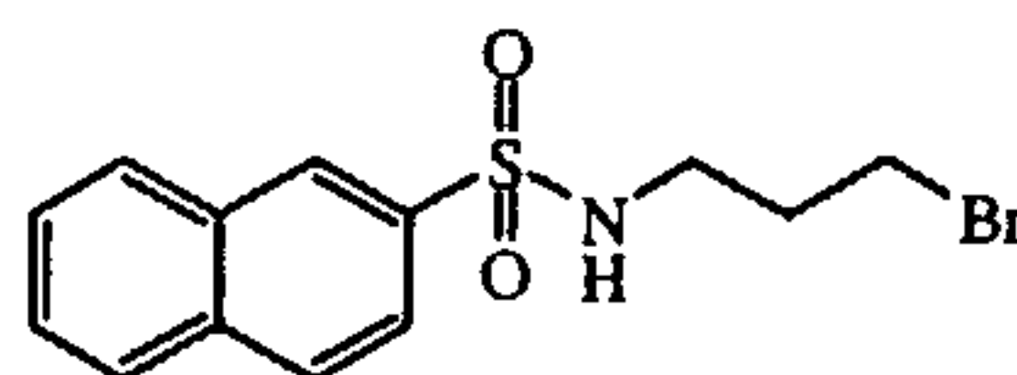
intermediate 38
