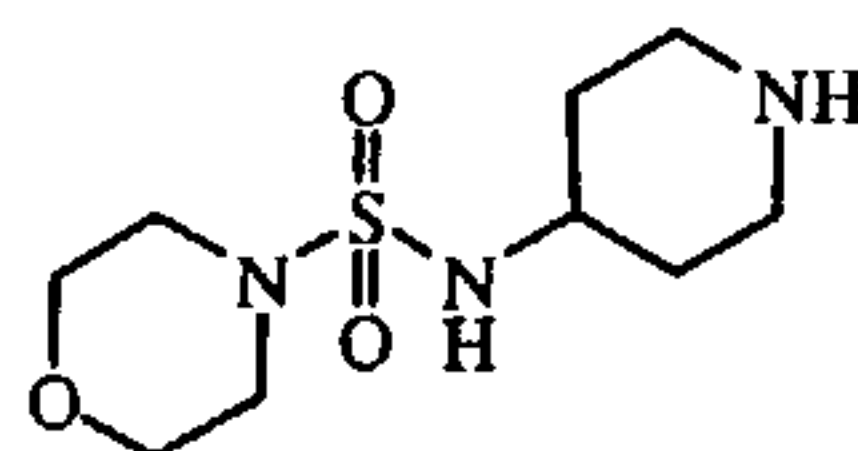
.HCl intermediate 37
