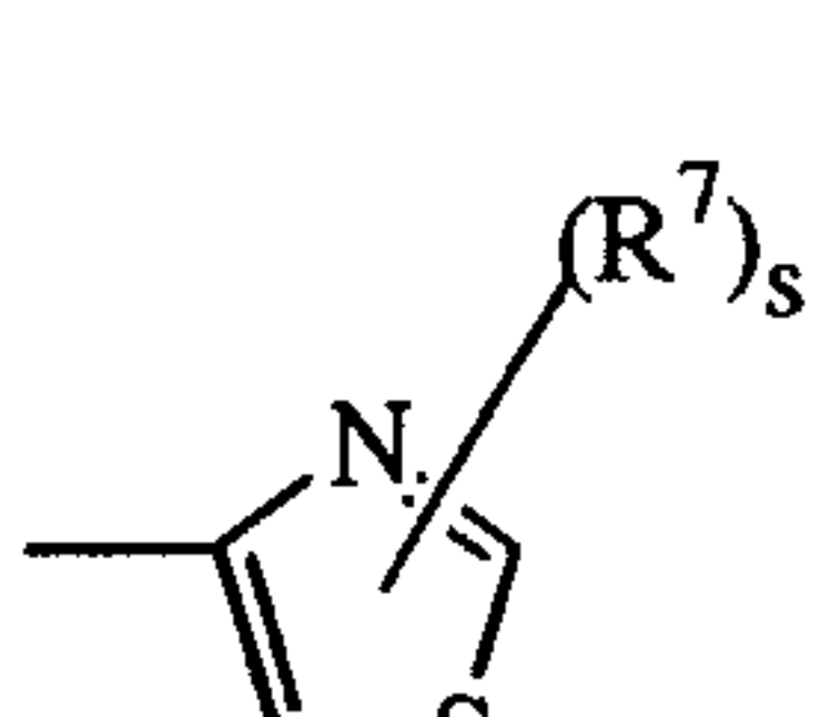
(a-15)
