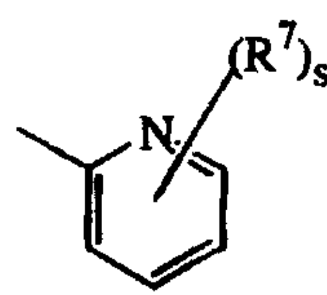
(a-3)
