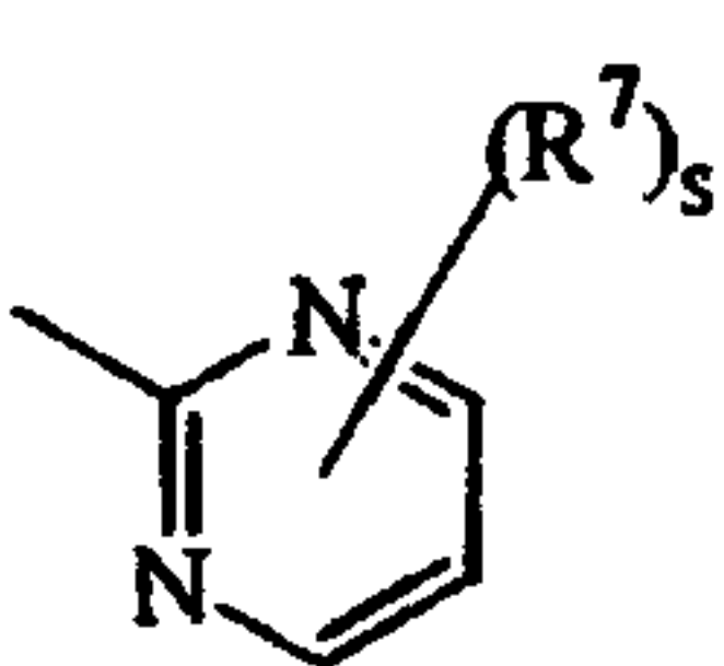
(a-5)
