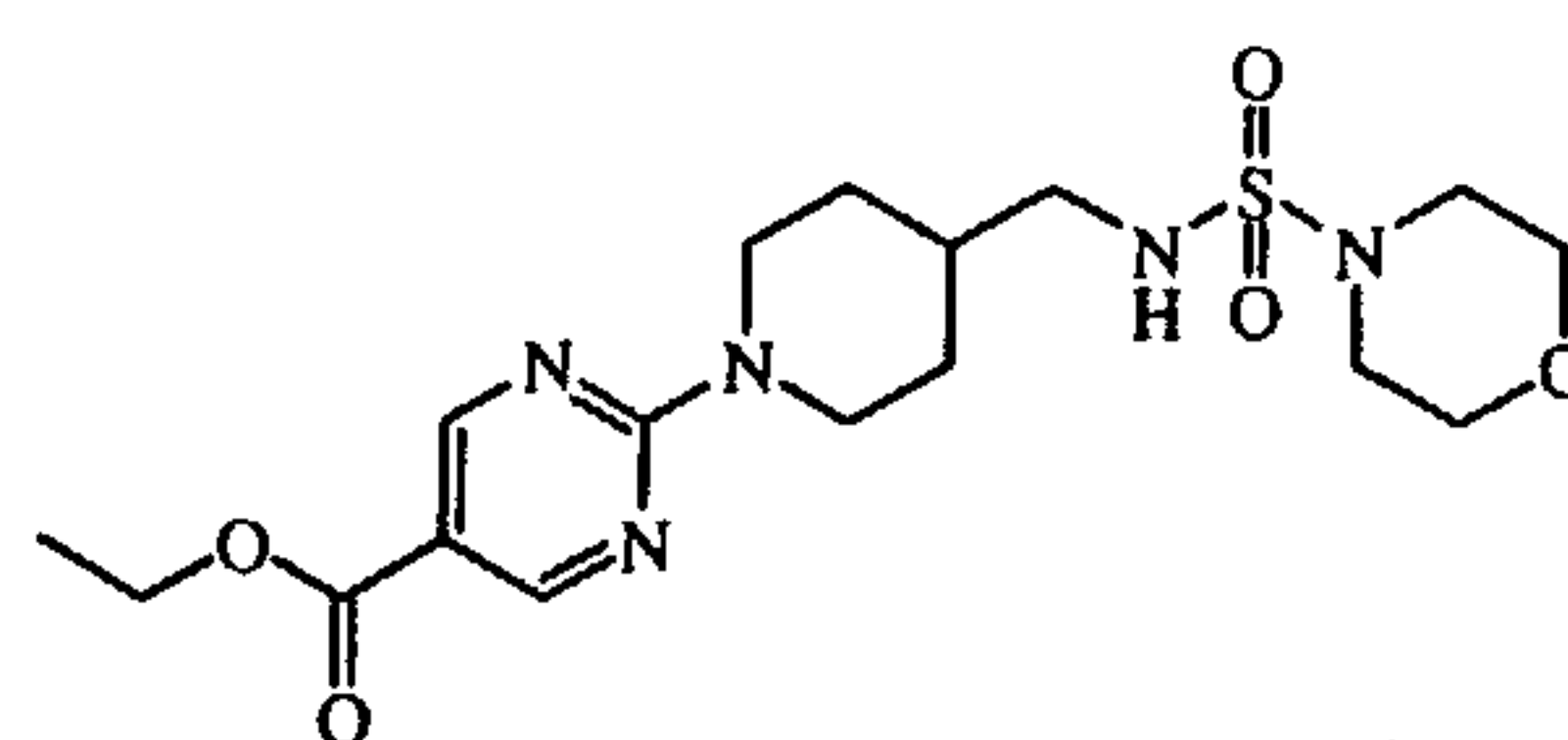
intermediate 55
