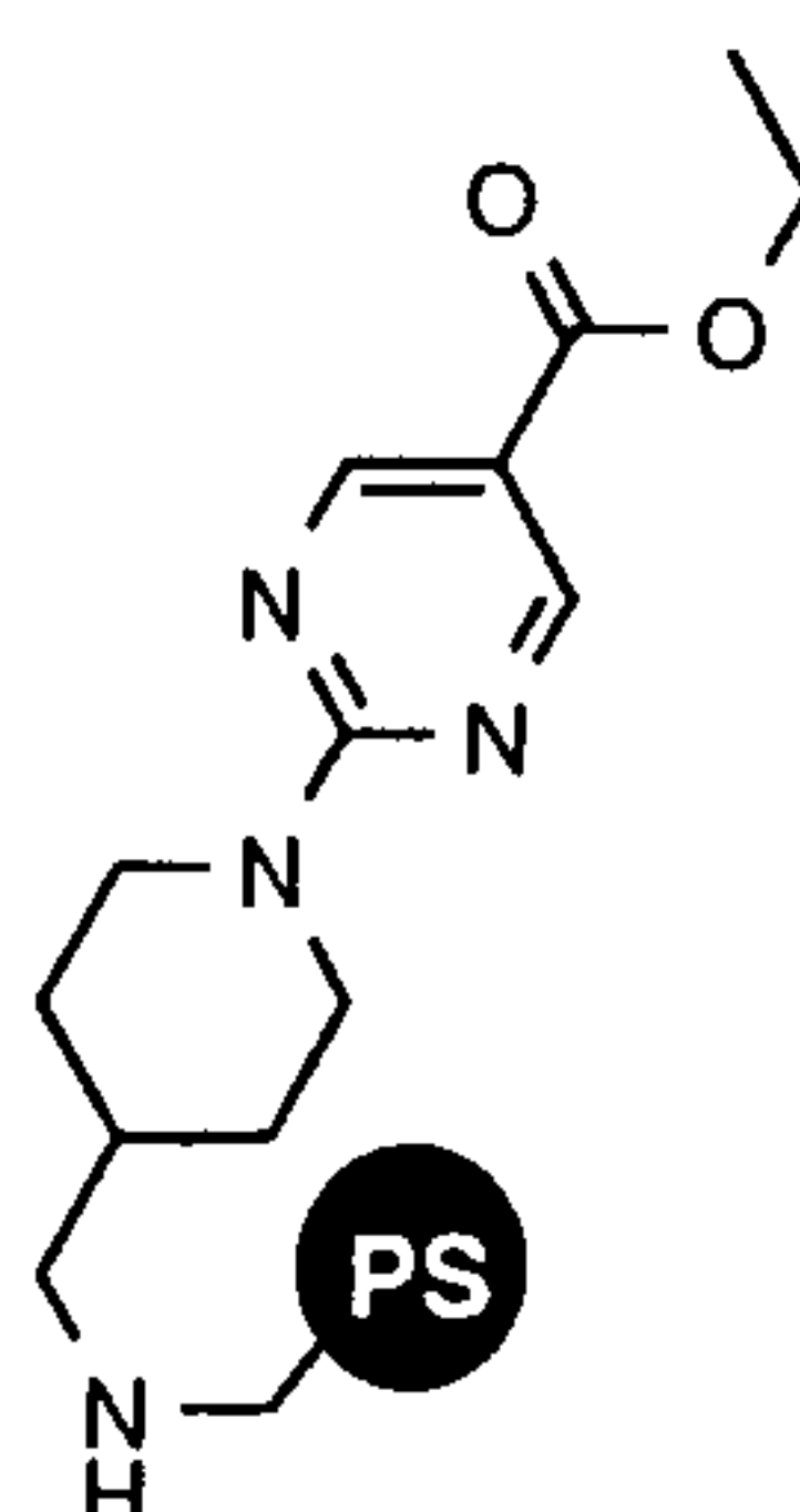
intermediate 48
