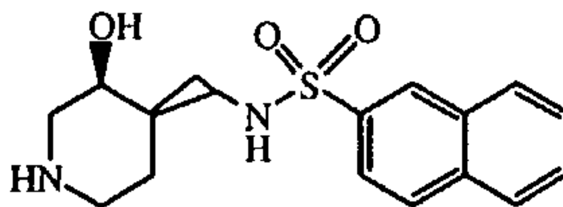
((3S-TRANS)) intermediate 19
