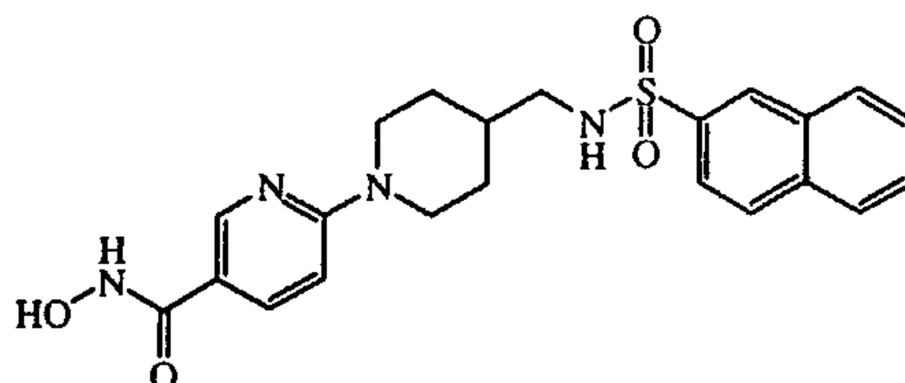
compound 4
