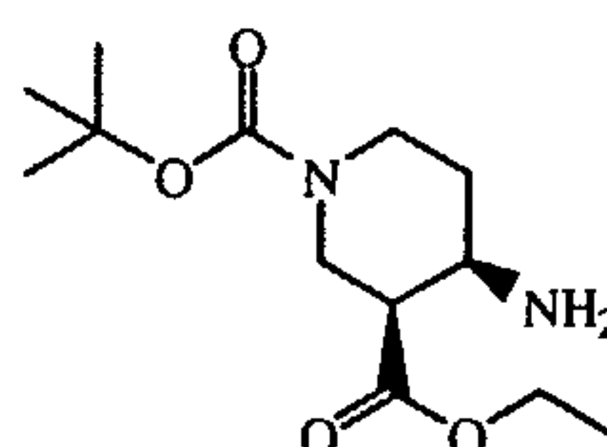
CIS intermediate 14
