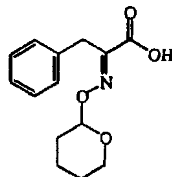
intermediate 6
