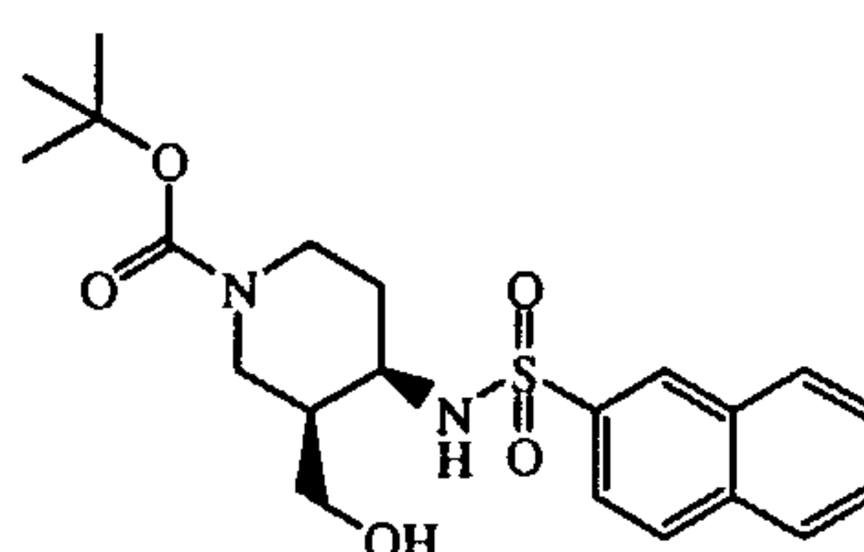
CIS intermediate 16
