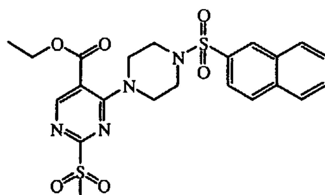
intermediate 13
