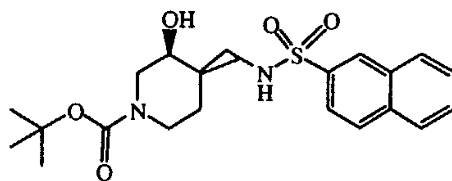
((3S-TRANS)) intermediate 18
