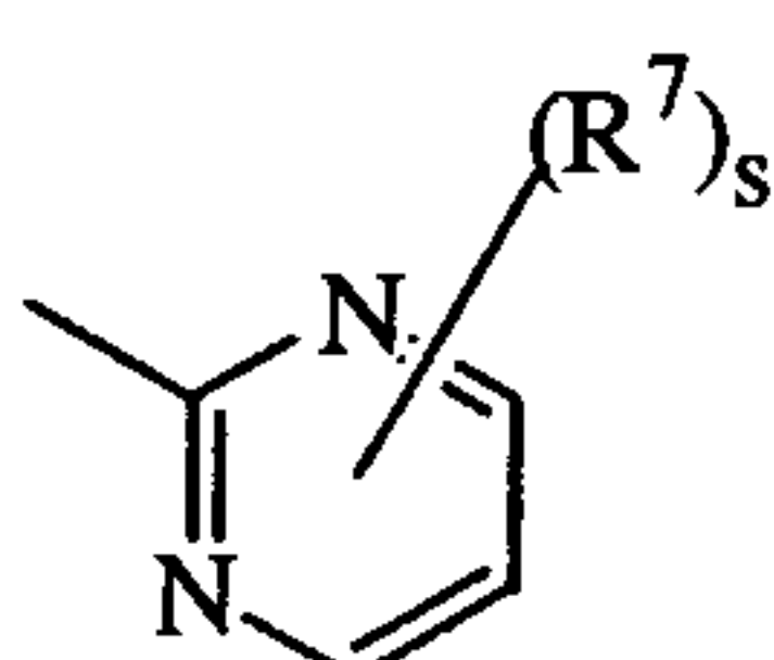
(a-5)
