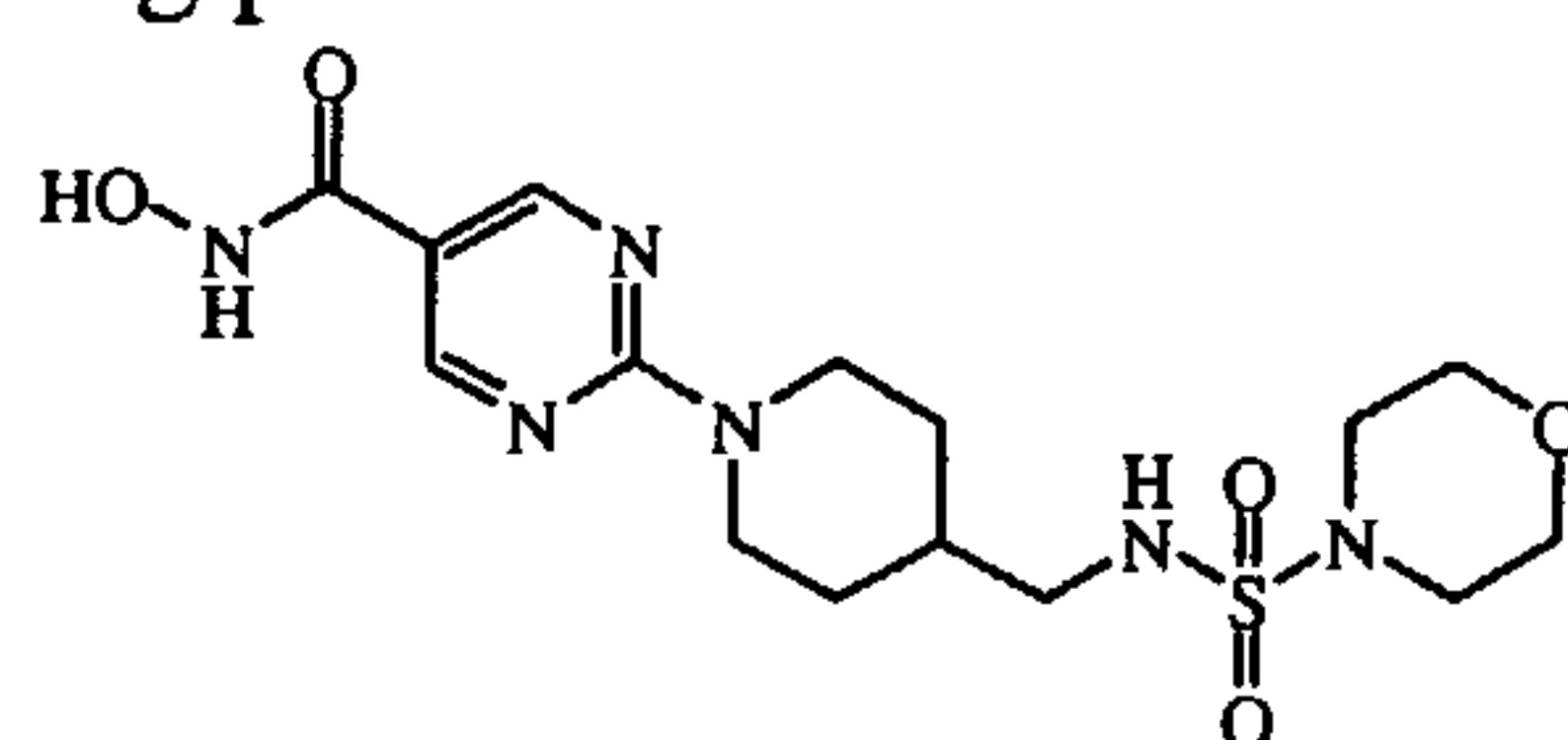
compound 28
