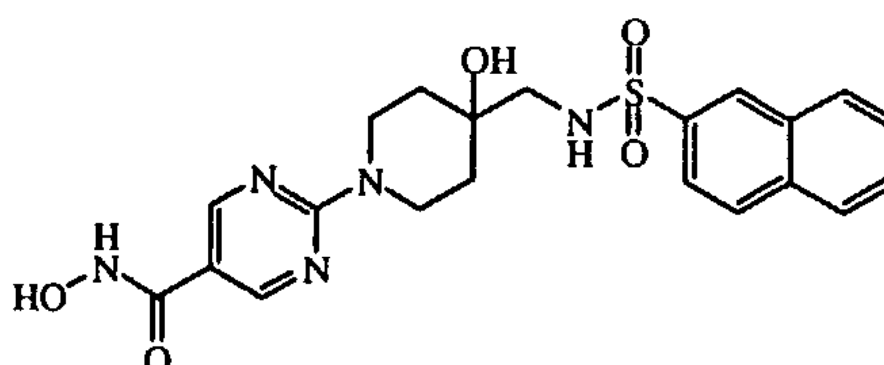
compound 9
