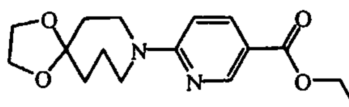
intermediate 22
