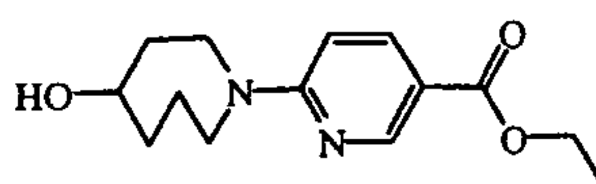
intermediate 24
