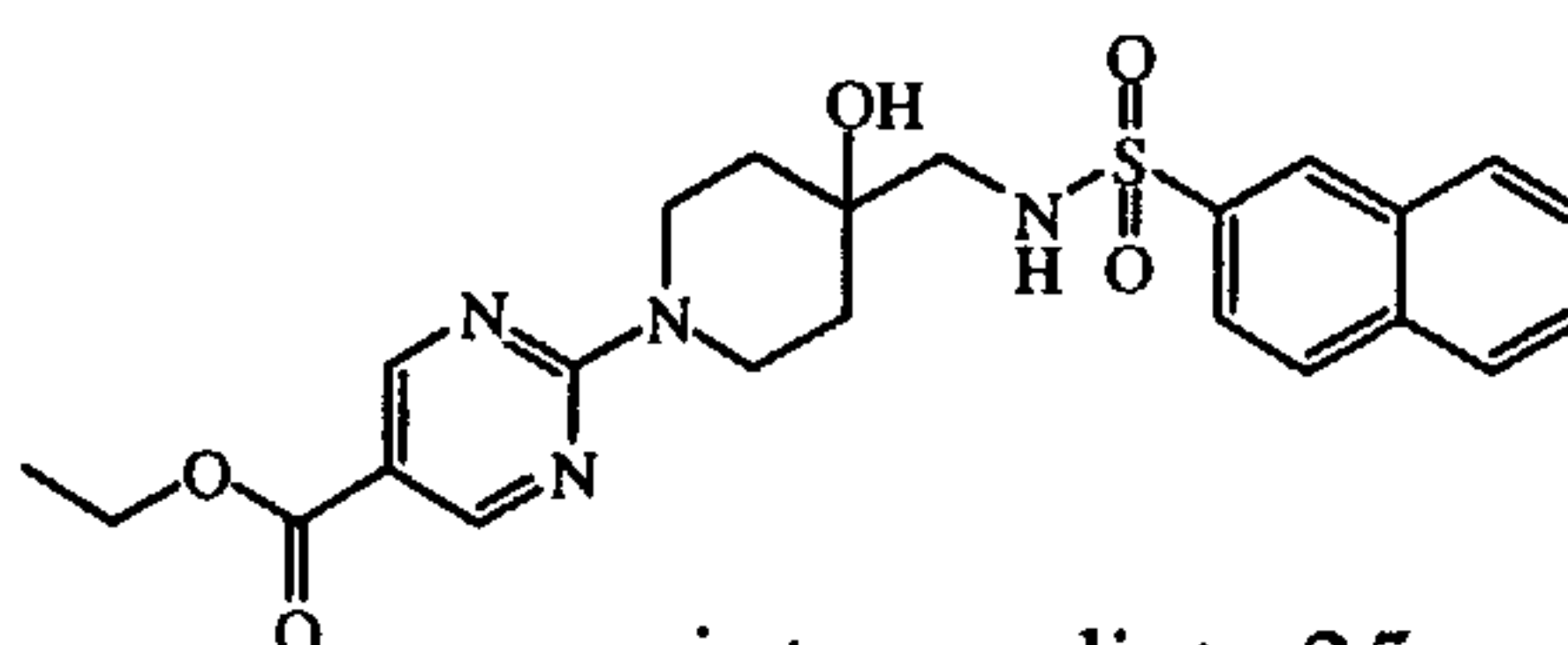
intermediate 35
