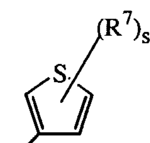
(a-10)
