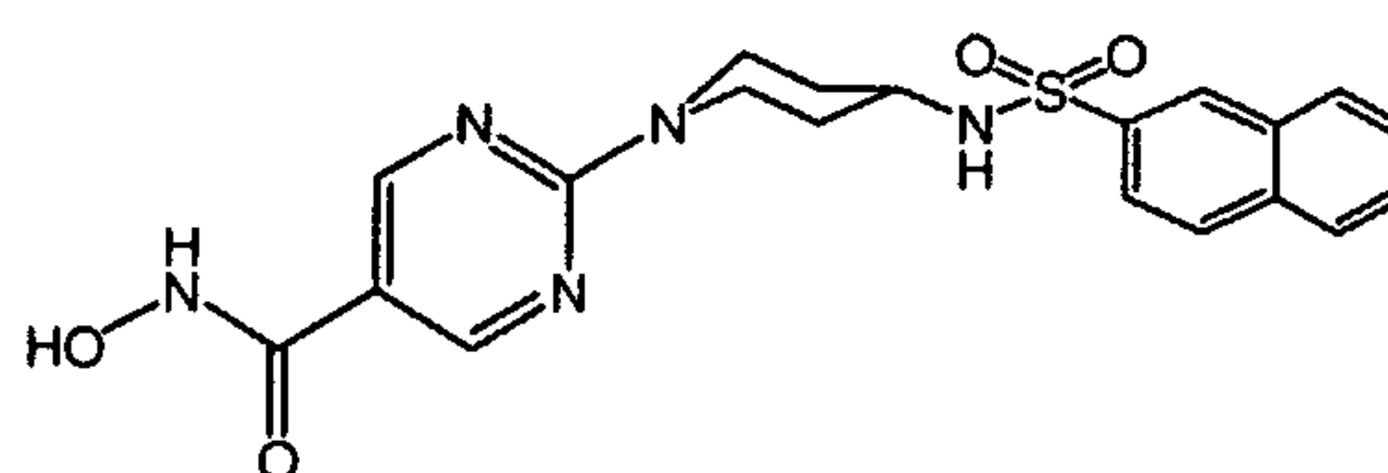
compound 2
