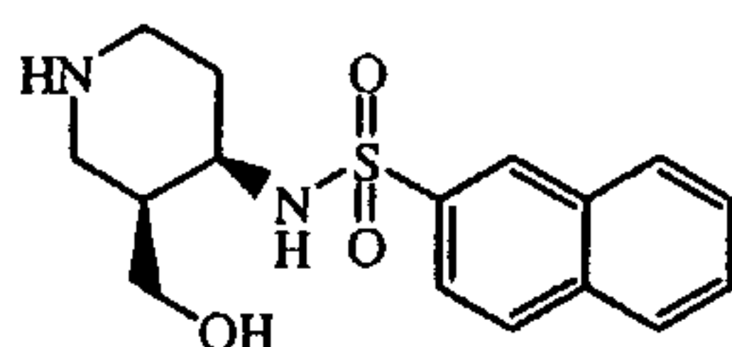
CIS intermediate 17
