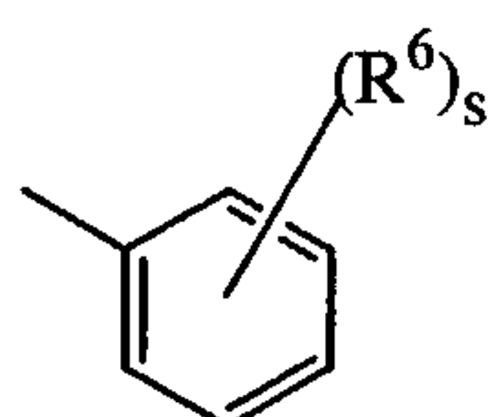
(a-1)
