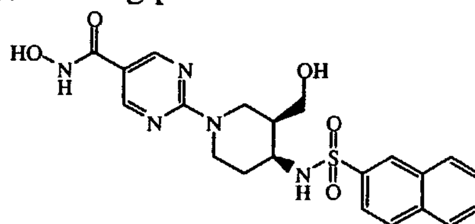
(CIS) compound 7
