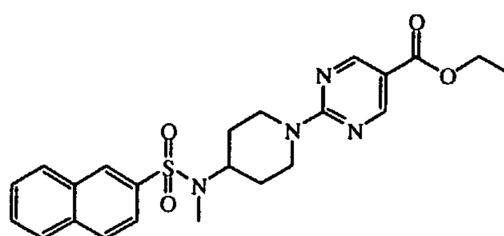
intermediate 56
