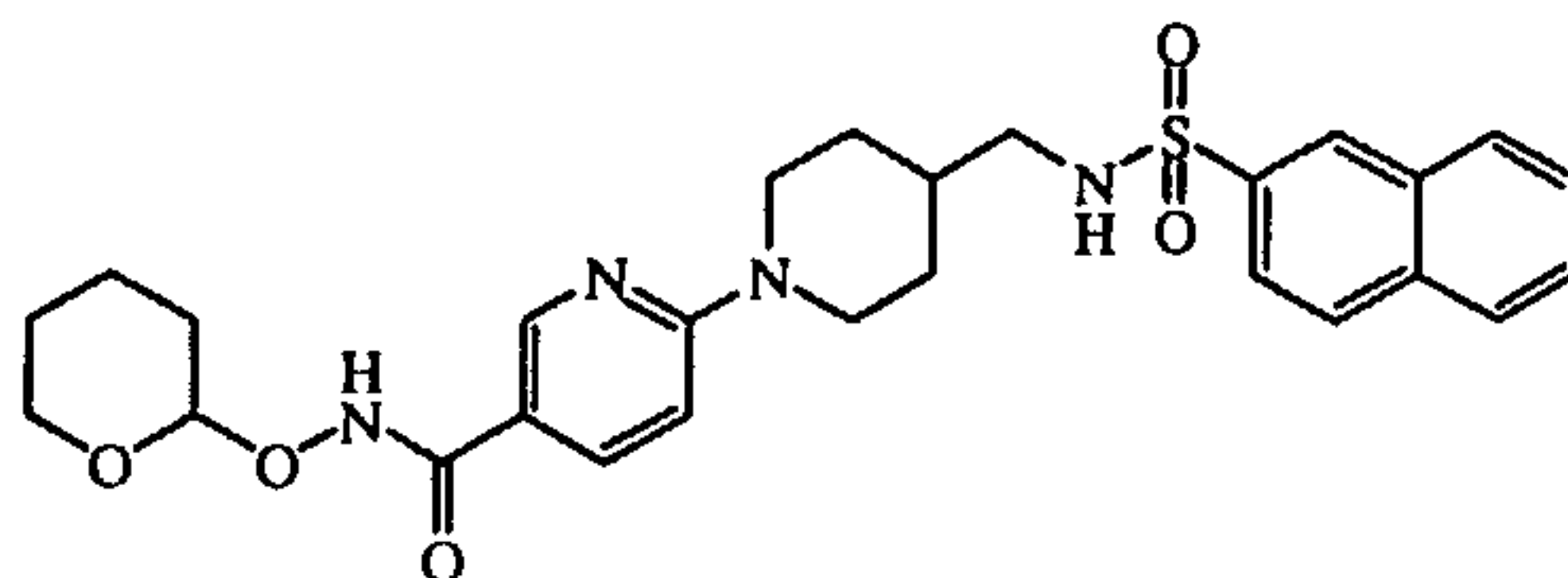
intermediate 30
