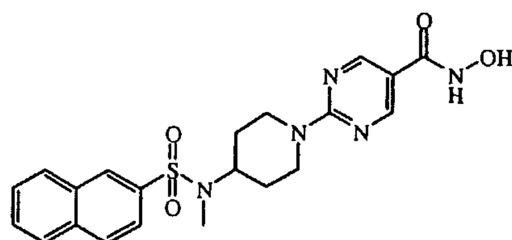
compound 29
