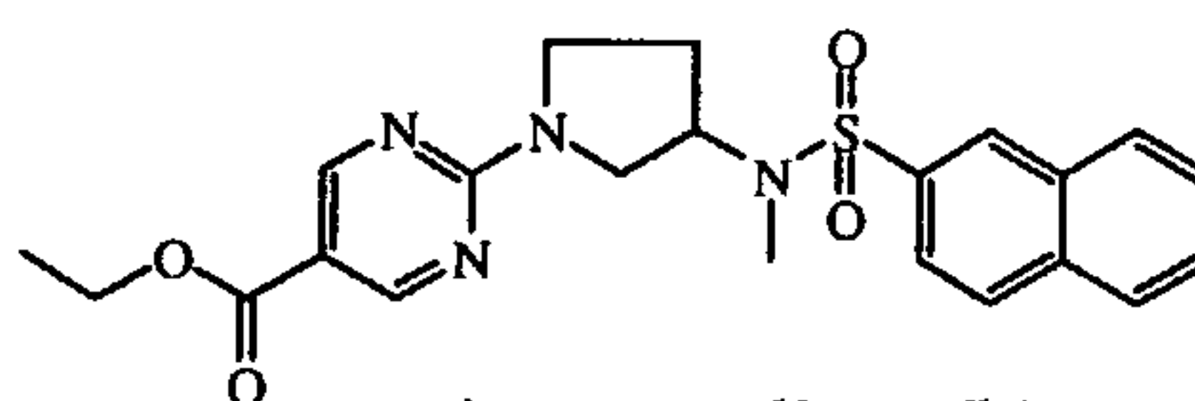
intermediate 54
