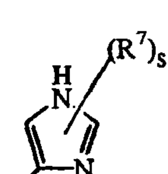
(a-14)
