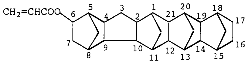
(157) pentacyclo[4.7.0.1 2,5 .0 8,13 .1 9,12 ]pentadecyl-3-methacrylate
