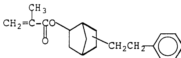
(219) 5(or 6)-tolyl-bicyclo[2.2.1]heptyl-2-methacrylate
