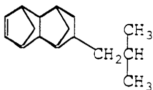
(420) 8-hexyltetracyclo[4.4.0.12,5.17,10]-3-dodecene
