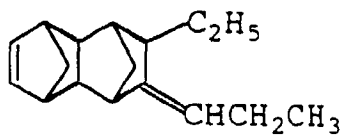
(443) 8-n-propylidene-9-isopropyltetracyclo[4.4.0.12.5.17,10]-3-dodecene
