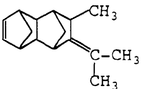
(447) 8-isopropylidene-9-ethyltetracyclo[4.4.0.12.5.17,10]-3-dodecene
