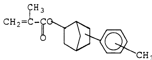
(220) 5(or 6)-(ethylphenyl)-bicyclo[2.2.1]heptyl-2-methacrylate
