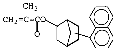
(226) 5(or 6)-(anthracenyl)-bicyclo[2.2.1]heptyl-2-methacrylate
