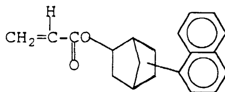
(212) 5(or 6)-(anthracenyl)-bicyclo[2.2.1]heptyl-2-acrylate
