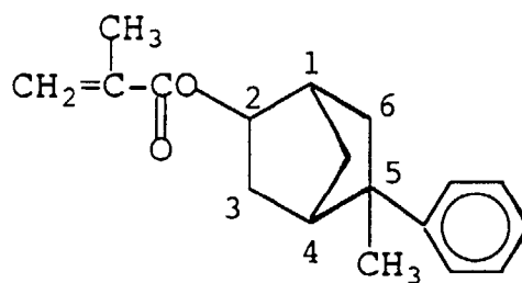
(217) 5(or 6)-benzyl-bicyclo[2.2.1]heptyl-2-methacrylate
