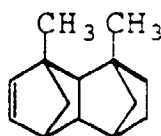
(425) 8,9-dimethyltetracyclo[4.4.0.1 2,5 .1 7,10 ]-3-dodecene
