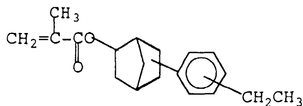
(221) 5(or 6)-(isopropylphenyl)-bicyclo[2.2.1]heptyl-2-methacrylate
