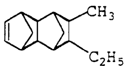
(427) 11,12-dimethyltetracyclo[4.4.0.1 2,5 .1 7,10 ]-3-dodecene
