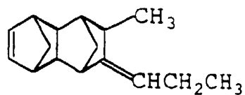
(442) 8-n-propylidene-9-ethyltetracyclo[4.4.0.12.5.17,10]-3-dodecene
