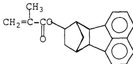
(225) 5(or 6)-(α-naphthyl)-bicyclo[2.2.1]heptyl-2-methacrylate
