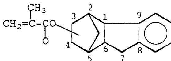
(223) 8,9-benzo-tricyclo[4.3.0.1 2,5 ]-undecyl-3-methacrylate
