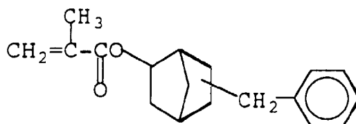
(218) 5(or 6)-(2-phenylethyl)-bicyclo[2.2.1]heptyl-2-methacrylate
