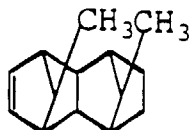
(428) 2,7,9-trimethyltetracyclo[4.4.0.1 2,5 .1 7,10 ]-3-dodecene
