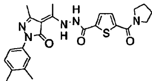
Synthetic Example 7
