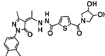
Synthetic Example 6
