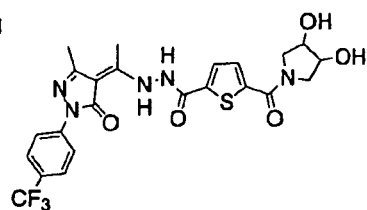
Synthetic Example 33
