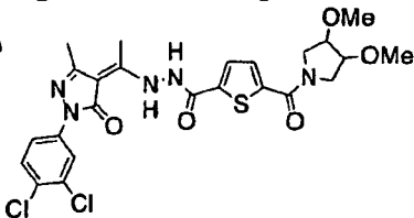
Synthetic Example 44
