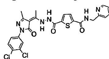
Synthetic Example 42
