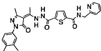
Synthetic Example 10
