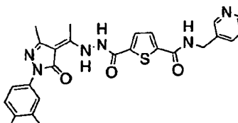
Synthetic Example 8
