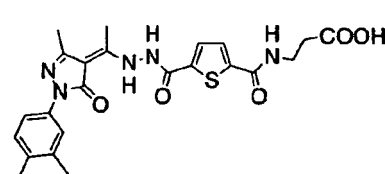
Synthetic Example 9
