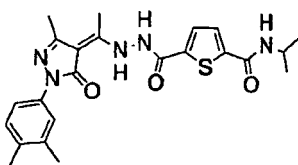
Synthetic Example 4
