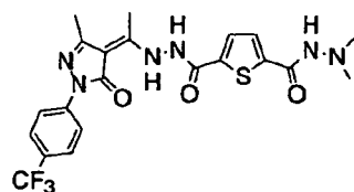
Synthetic Example 36
