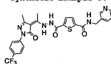
Synthetic Example 36
