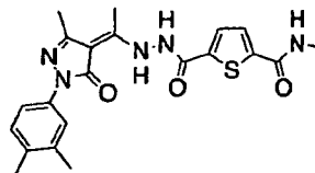
Synthetic Example 10
