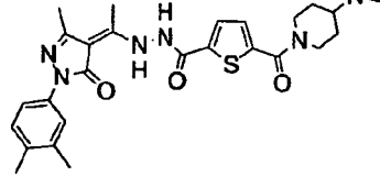
Synthetic Example 9
