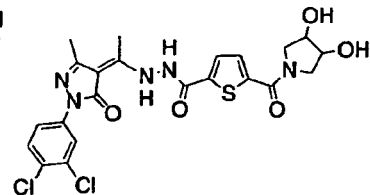
Synthetic Example 42
