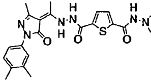
Synthetic Example 8
