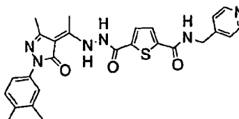
Synthetic Example 5
