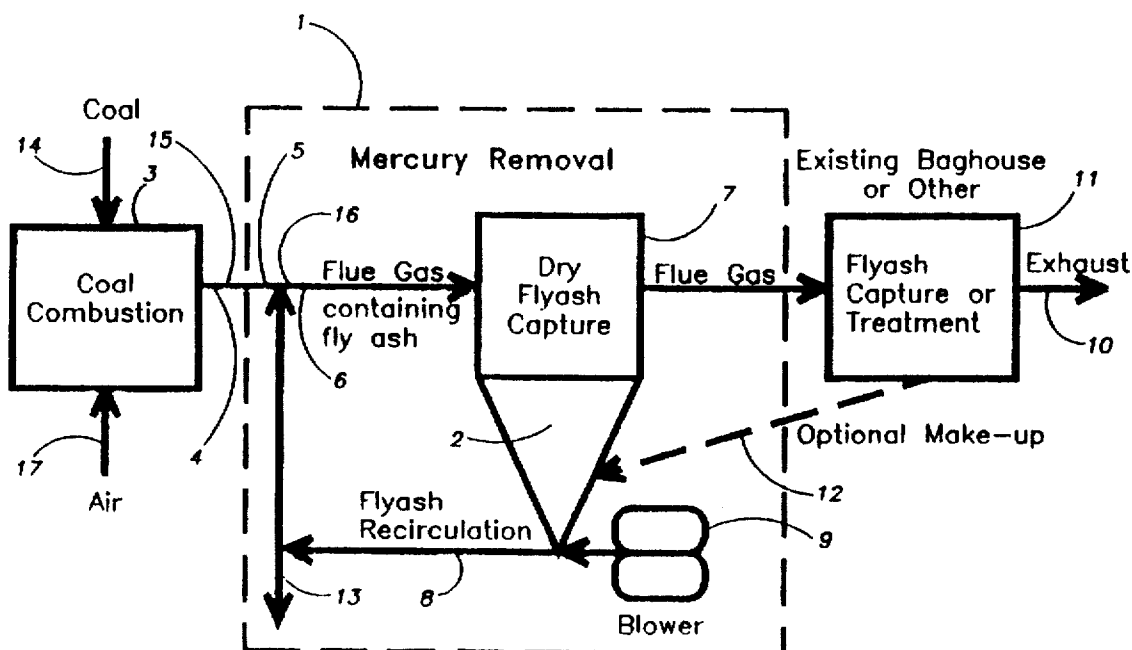
Flyash Recirculation for Mercury Sorption
