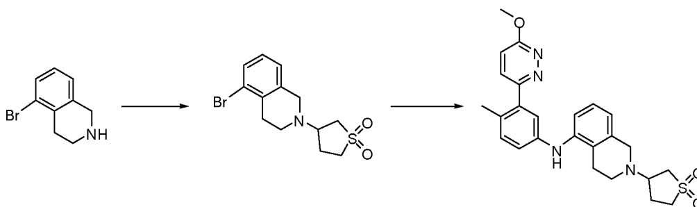
Scheme 7
