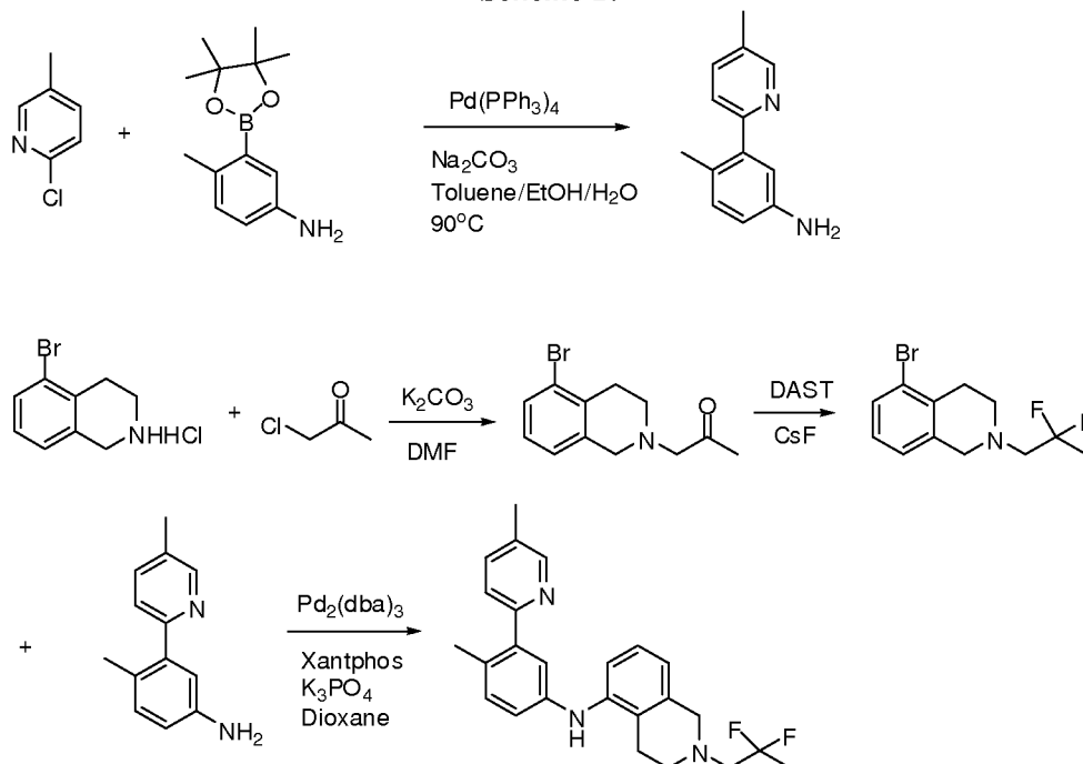
Scheme 2:
