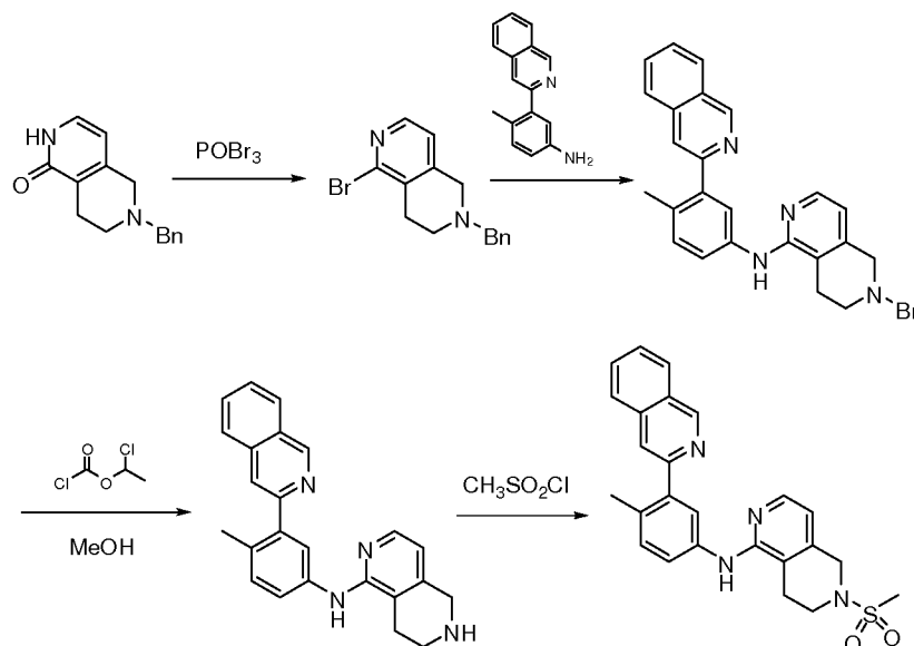
Scheme 9
