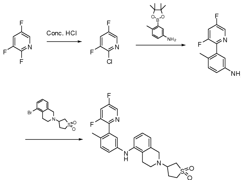
Scheme 8
