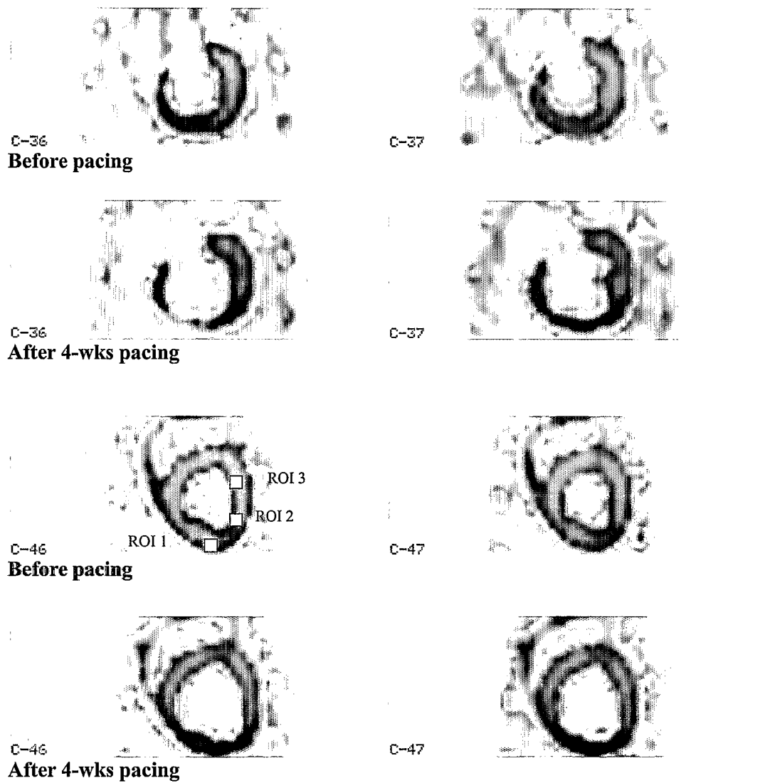
Figure 18: A decrease in F-18-FBnTp uptake in the inferior wall following pacing-induced heart failure.
