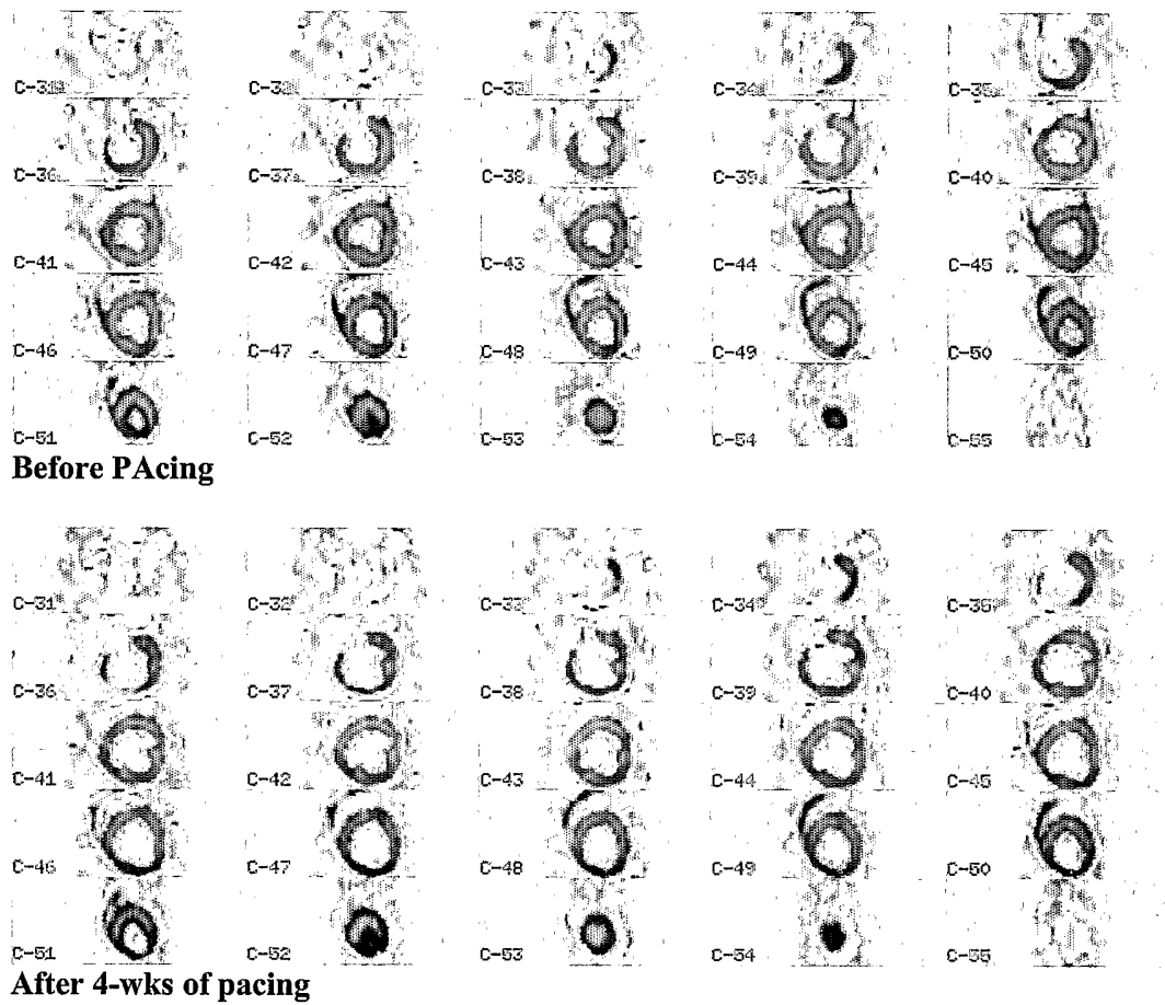
Figure 17: F-18-FBNTP PET short-axis images of the myocardium before and after pacing
