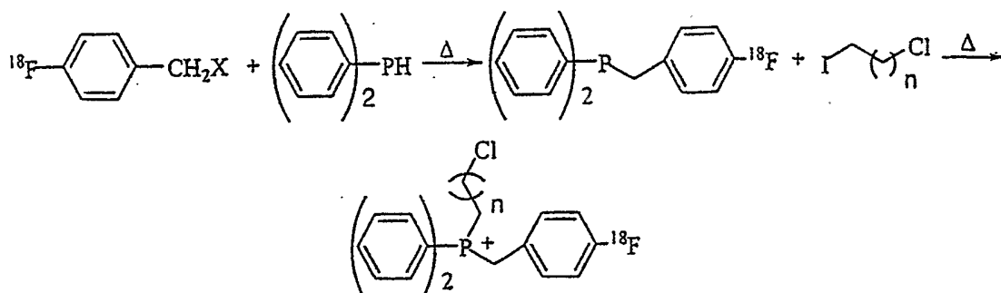
Scheme 3: synthesis of the [ 18 F]-benzyl-chloroalkyl phosphonium ion.
