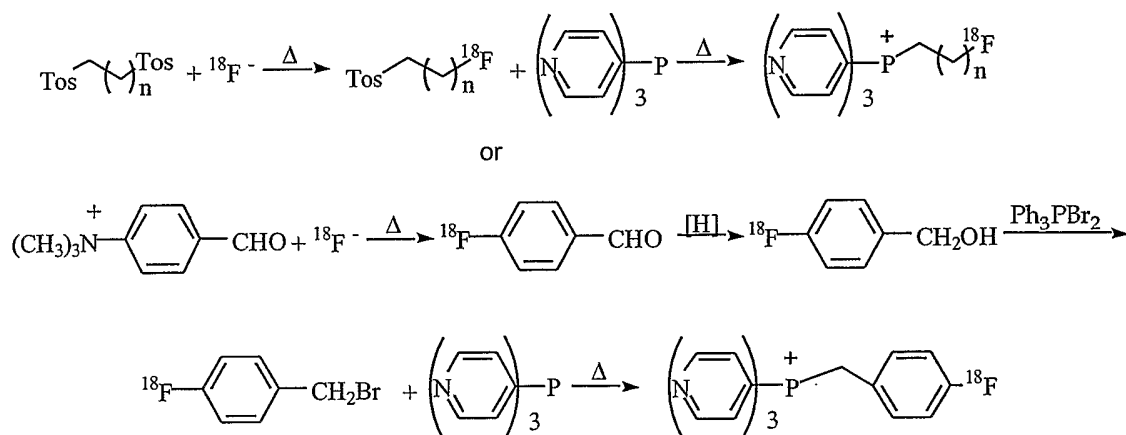
Scheme 4: synthesis of [ 18 F]-alkyl or aryl tripyridylphosphonium ion
