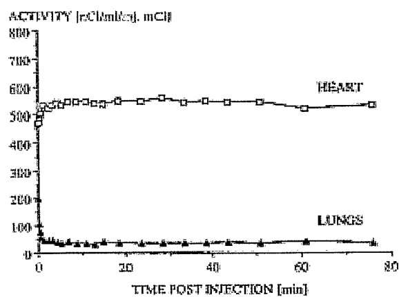
Figure 10: C-11TPMP myocardial uptake
