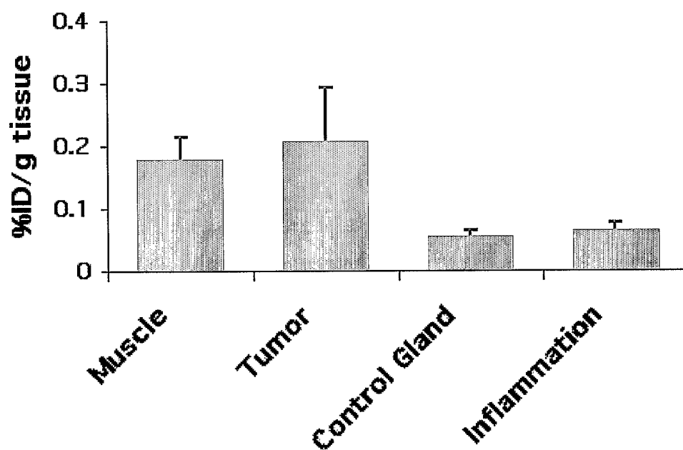
Figure 4. Accumulation of ^{18}\text{F} -FBnTP in malignant (Tumor) and healthy (control) mammary gland and in healthy (Muscle) and inflammation muscle, in rats.
