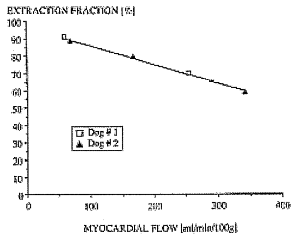
Figure 11: C-11-TPMP extraction fraction
