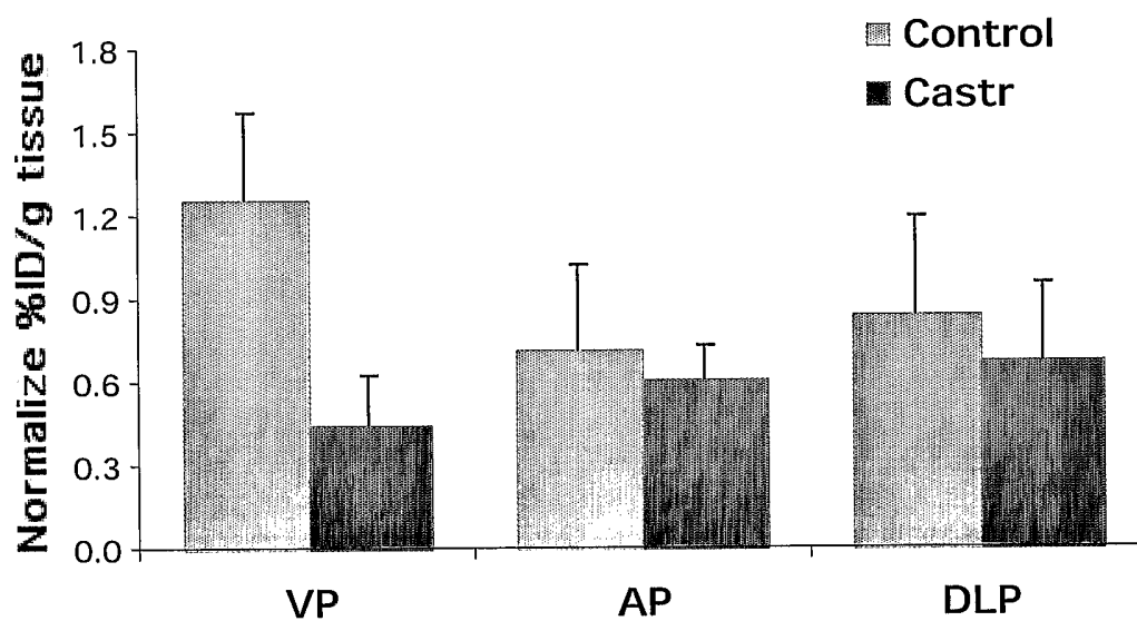
Figure 6: Accumulation of F-18-FBnTP in the prostate lobes 4 days after castration. Castration-produced apoptosis induced significant lobe-specific decrease in the ventral aspect, compared to control
