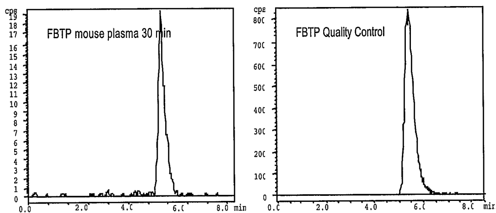
Figure 1 Radiochromatograms of ^{18}\text{F} -FBnTP (quality control) and plasma 30 min p.i. of the tracer into mice.
