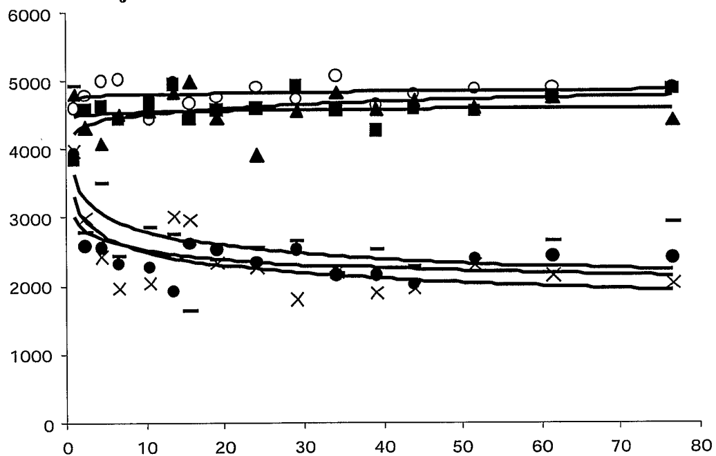
Figure 14: F-18-FBnTP accumulation kinetics in the left and right ventricles in 3 consecutive axial slices (8 to 10). Each trace is the mean of ROIs as above demonstrated. This figure is a good example for the rapid fact kinetics of FBnTP and uniform distribution in the myocardium.
