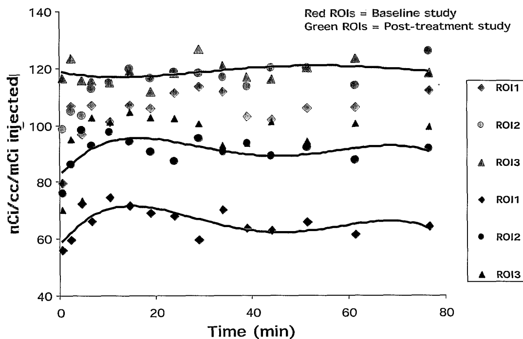
Figure 19: Time-activity course of [^{18}\text{F}]\text{FBnTP} myocardial uptake before (red) and after 4 weeks of pacing. Each data point represents the mean activity of four slices (slice 46 to 49). Positioning of region of interest (ROI) is shown in the left upper cardiac image. The same ROIs template was used to retrieve data in all cardiac sections.
