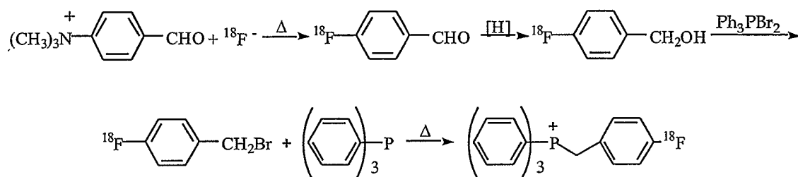
10 Scheme 2: Synthesis of [ ^{18}\text{F} ]aryl phosphonium ions.
