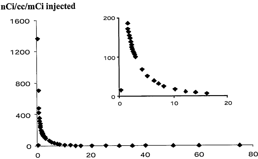
Figure 13: F-18-FBnTP rapid clearance from blood
