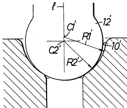
FIG. 4 PRIOR ART
