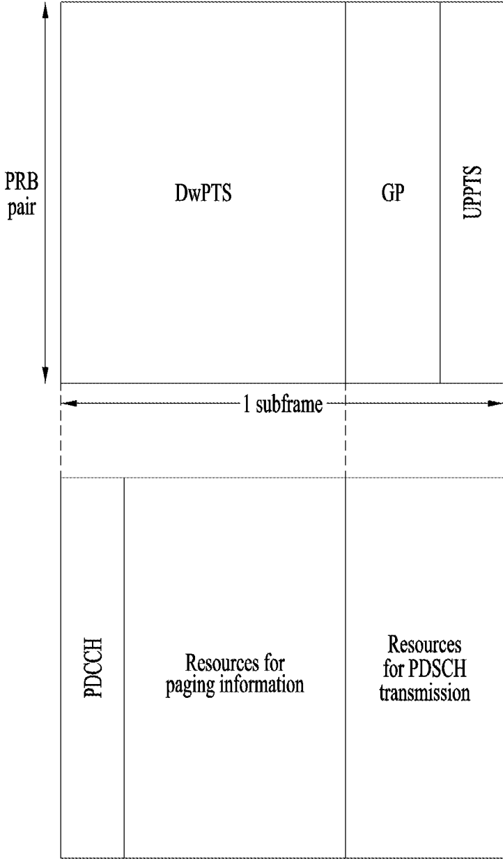
Resources usage for advanced UE in SD subframe
