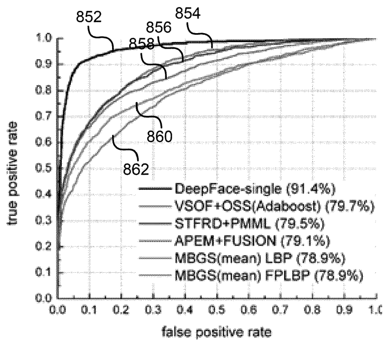
Figure 4. The ROC curves on the YTF dataset.
