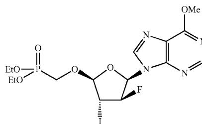
55 (2'R,3'S,4'R,5'R)-6-Methoxy-9-[tetrahydro 4-iodo-3-fluoro-5-(diethoxyphosphinyl)methoxy-2-furanyl]purine (6)
