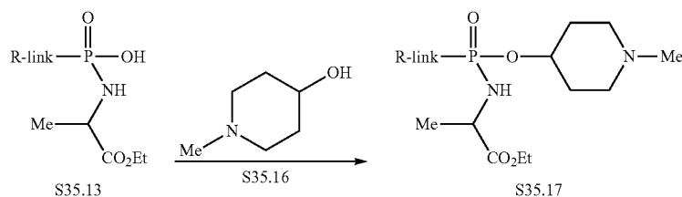
Scheme 35 Example 4
