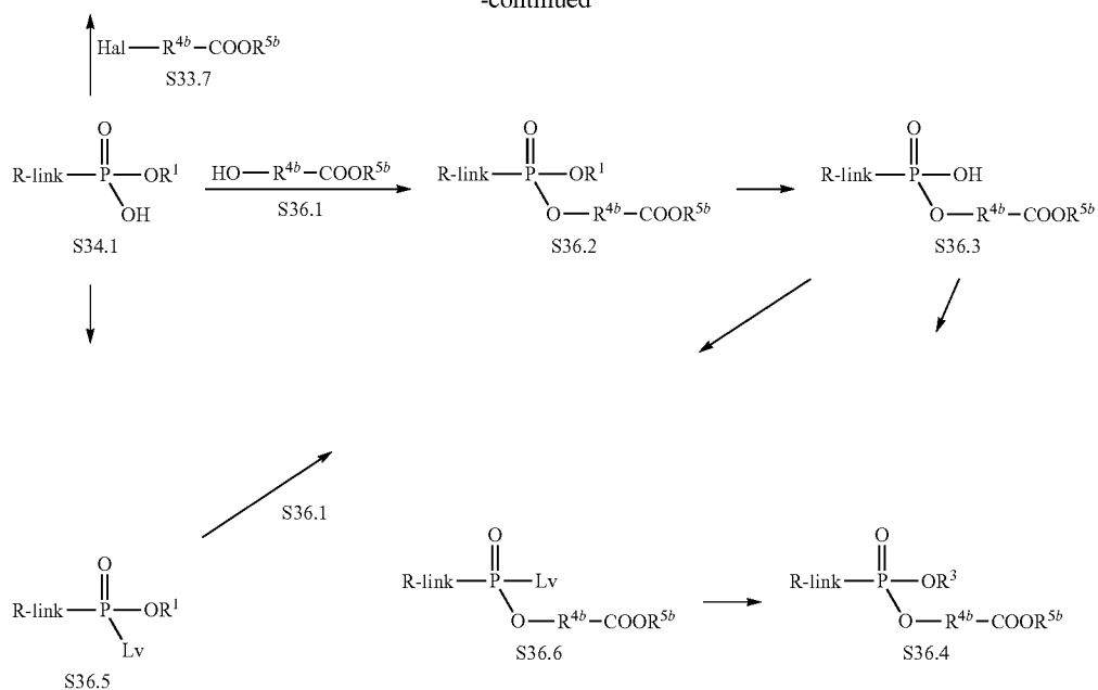
Scheme 36 Example 1
