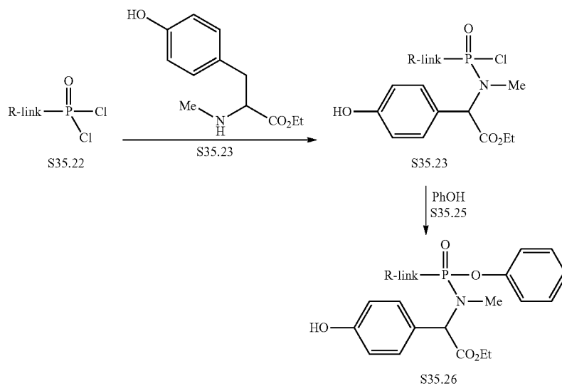
Scheme 35 Example 5
