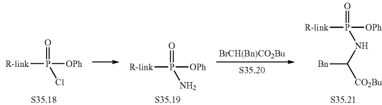
Scheme 35 Example 5
