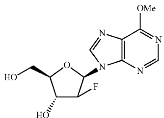
2-deoxy-2-fluoro-β-D-arabinofuranosyl-6-methoxyadenine (4)
