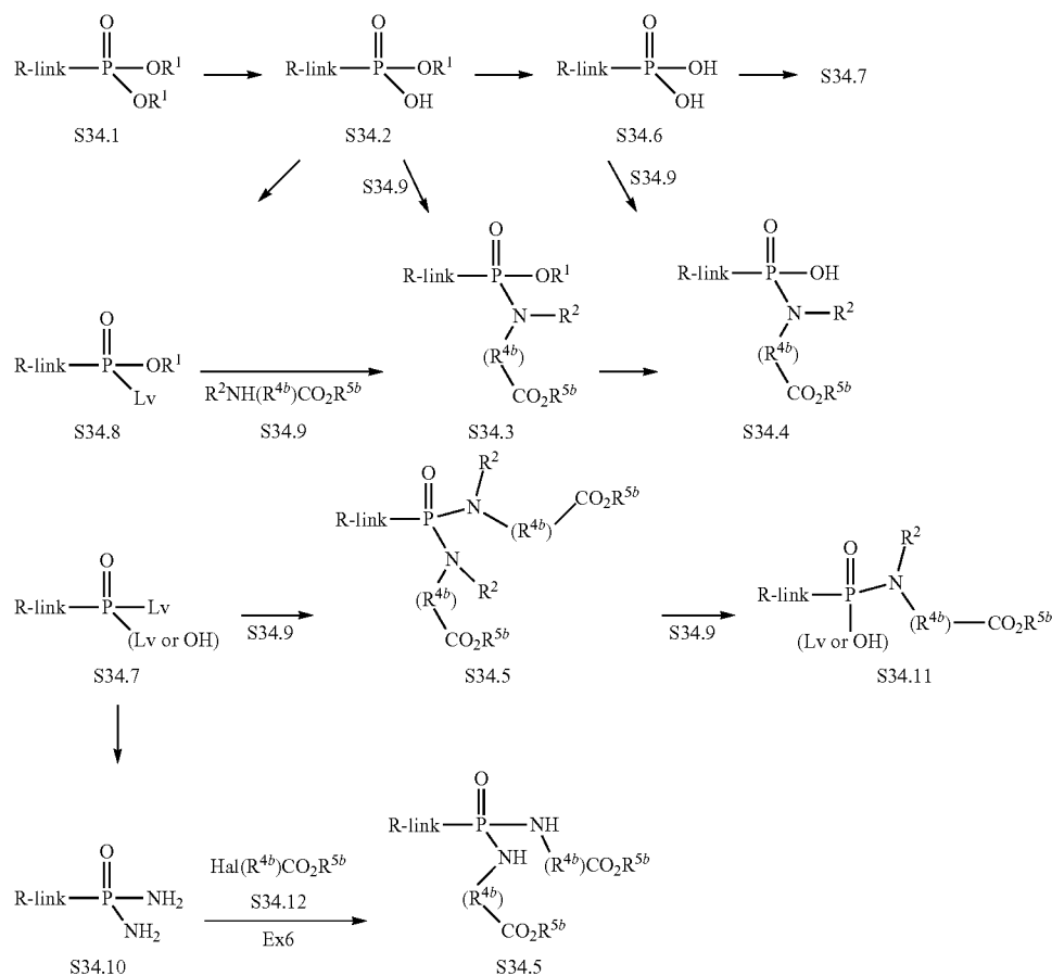
Scheme 34
