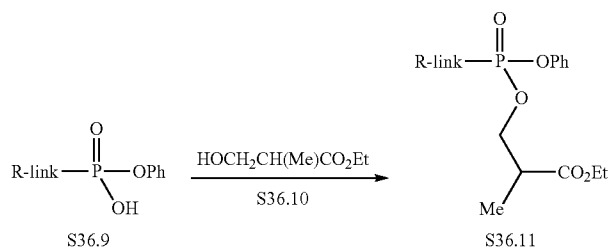
Scheme 36 Example 1
