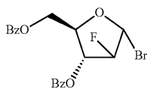
2-deoxy-2-fluoro-3,5-di-O-benzoyl-α-D-arabinofuranosylbromide (2)
