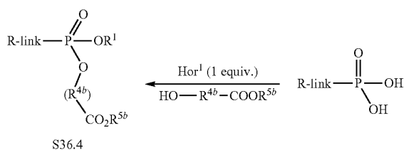
Scheme 36
