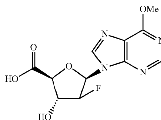
2-deoxy-2-fluoro-5-carboxy-β-D-arabinofuranosyl-6-methoxyadenine (5)
