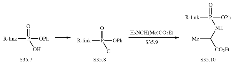
Scheme 35 Example 2
