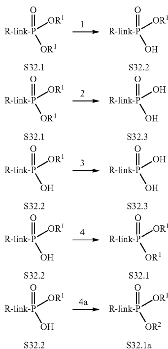
Scheme 32
