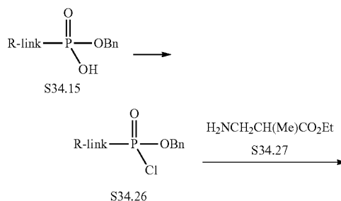
Scheme 34 Example 4
