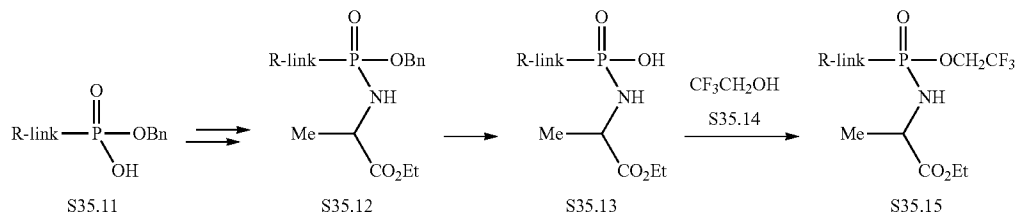
Scheme 35 Example 3
