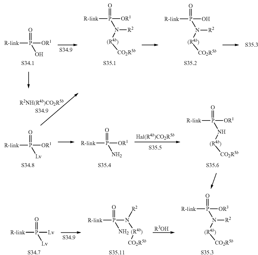
Scheme 35
