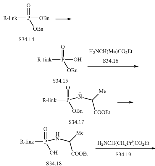
Scheme 34 Example 1
