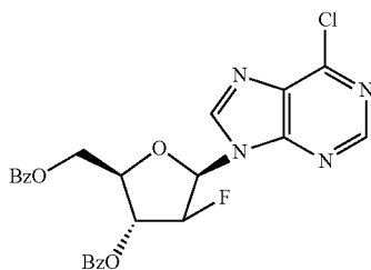
2-deoxy-2-fluoro-3,5-di-O-benzoyl-β-D-arabinofuranosyl-9H-6-chloropurine (3)
