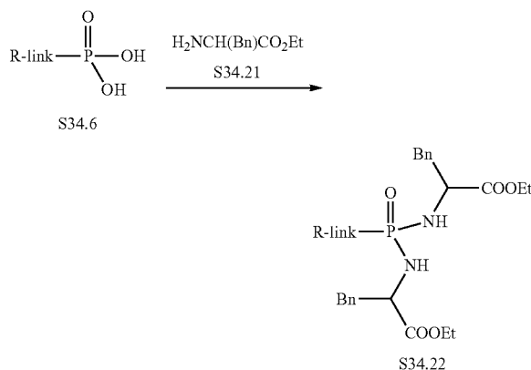
Scheme 34 Example 3
