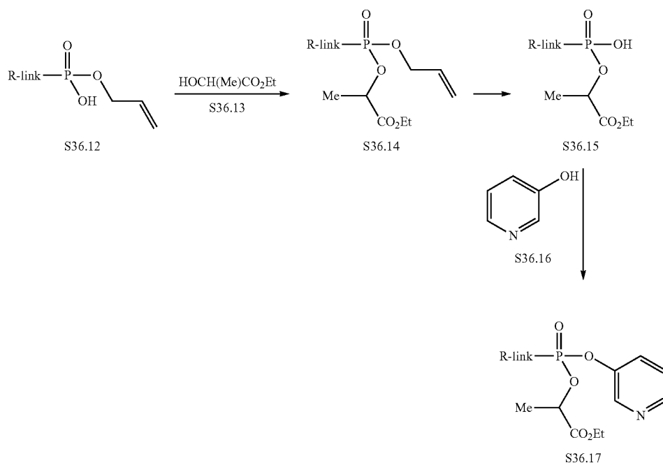
Scheme 36 Example 2
