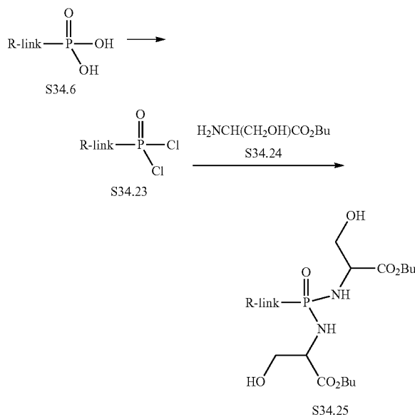
Scheme 34 Example 4
