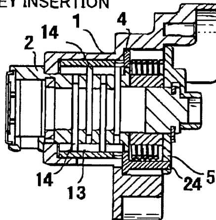
FIG. 4A BEFORE KEY INSERTION
