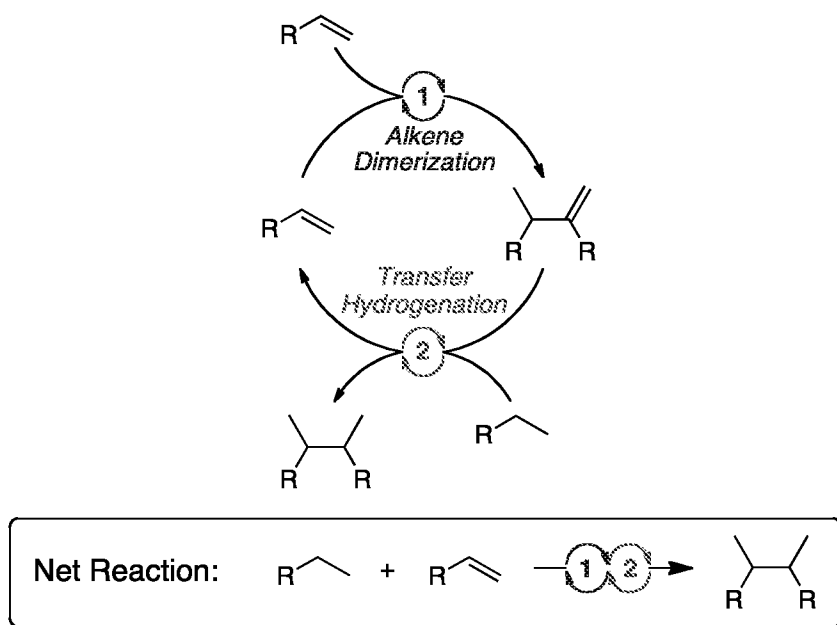
Scheme I: Idealized Tandem Catalytic Approach toward Alkane / Alkene Upgrading
