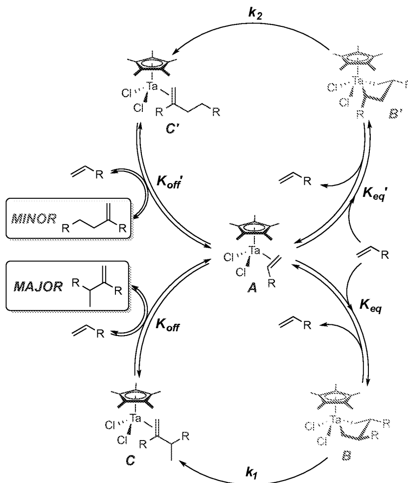
Scheme V: Postulated Catalytic Cycles for the Dimerization of 1-Alkenes into Two Regioisomers Catalyzed by 1
