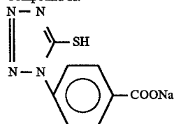
Compound-X:
