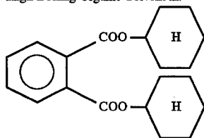
Compound-IX:
