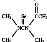
Selenium Compound-V:
