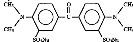
Dye-V:
