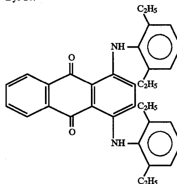
Dye-V:
