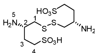
Compound I
