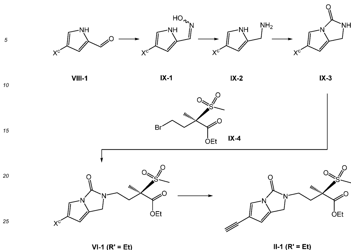
Scheme 9
