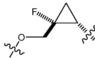
M C
