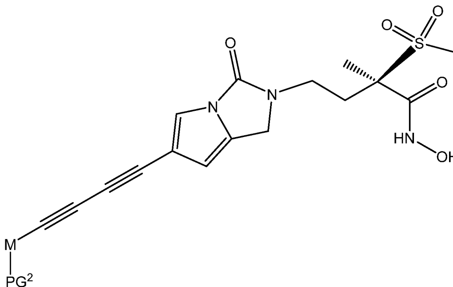
III
