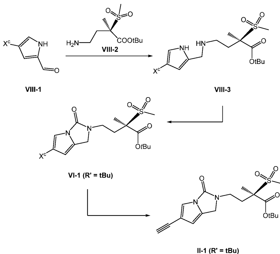
Scheme 8
