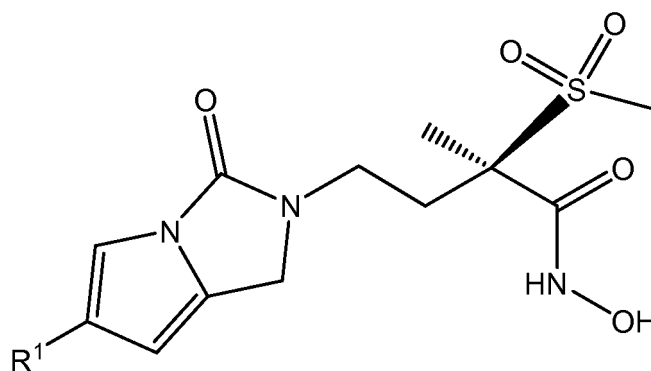
(A3)
