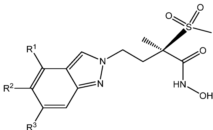
(A1)
