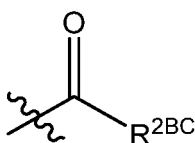
L^{2BC}
