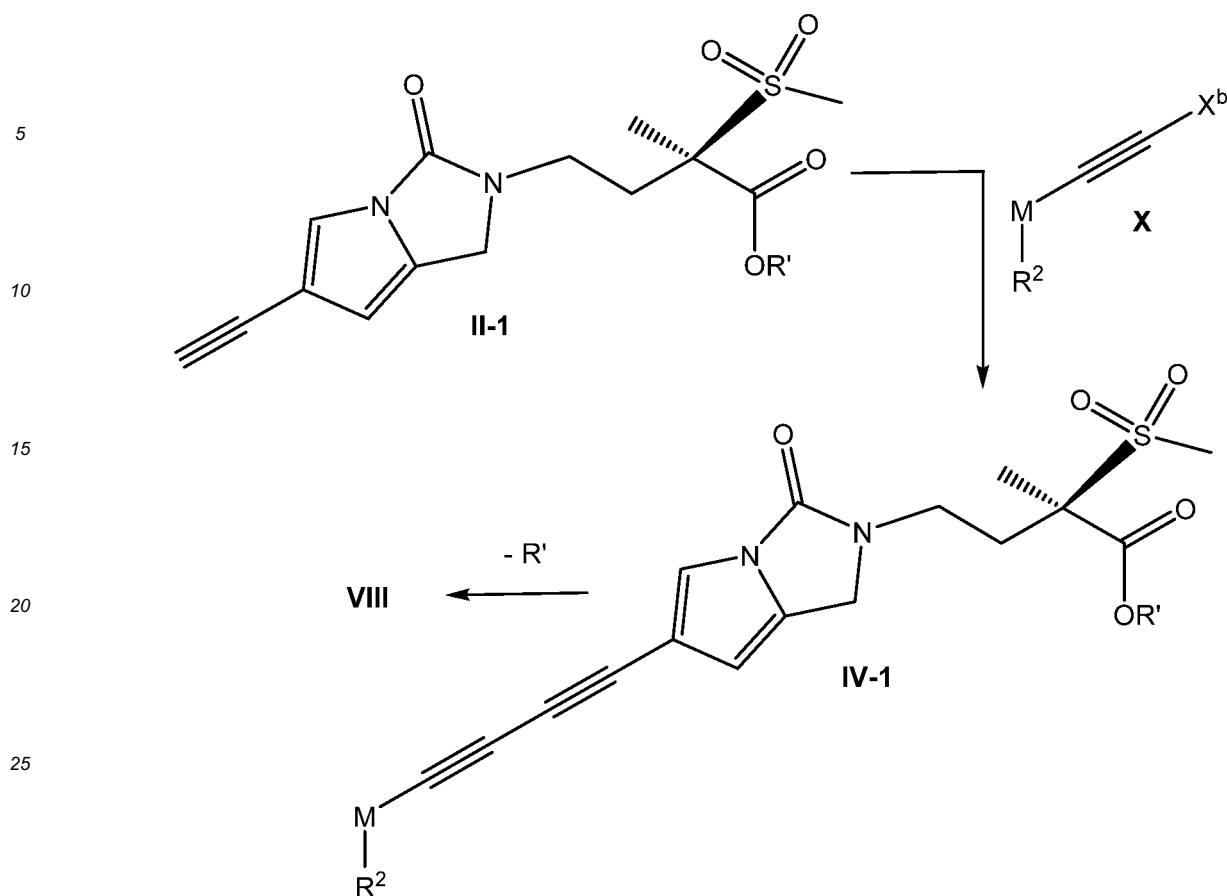
Scheme 4
