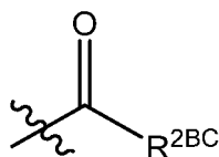
L^{2BC}
