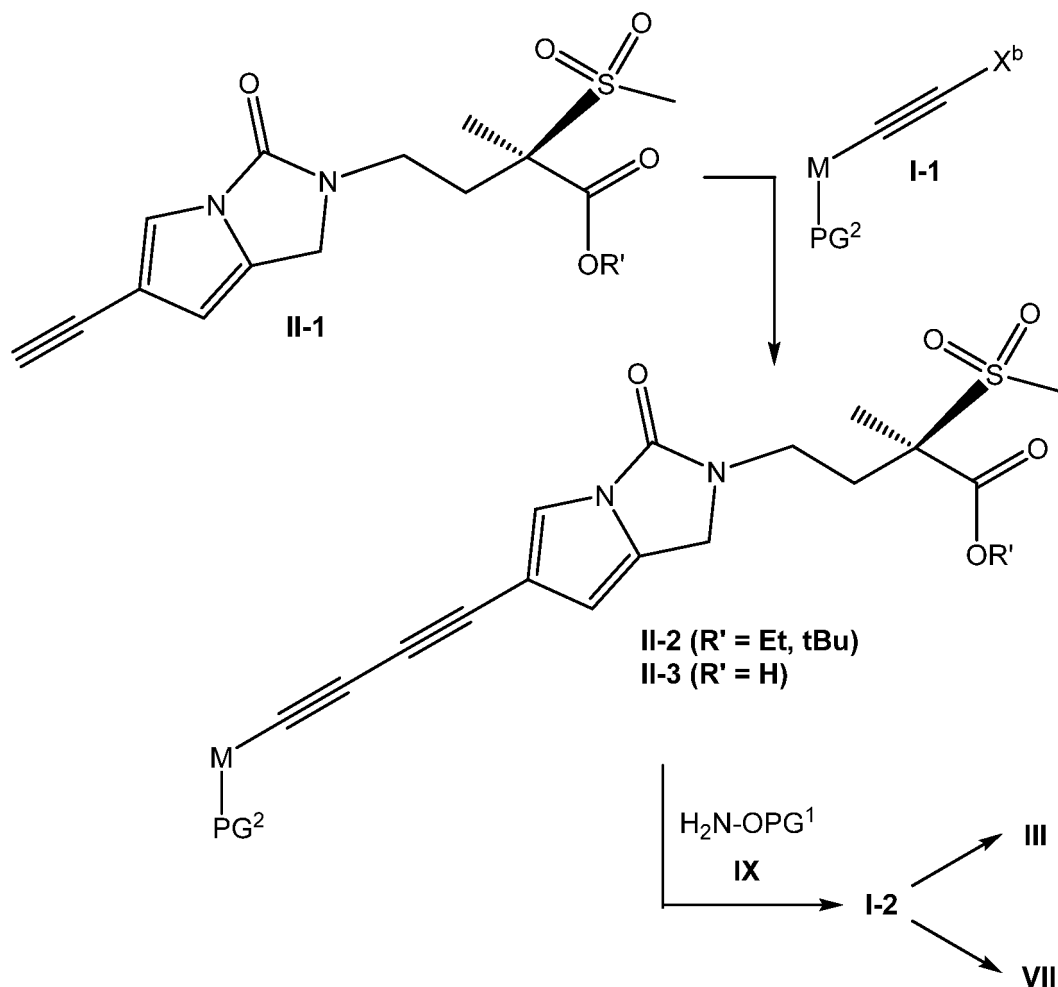
Scheme 2
