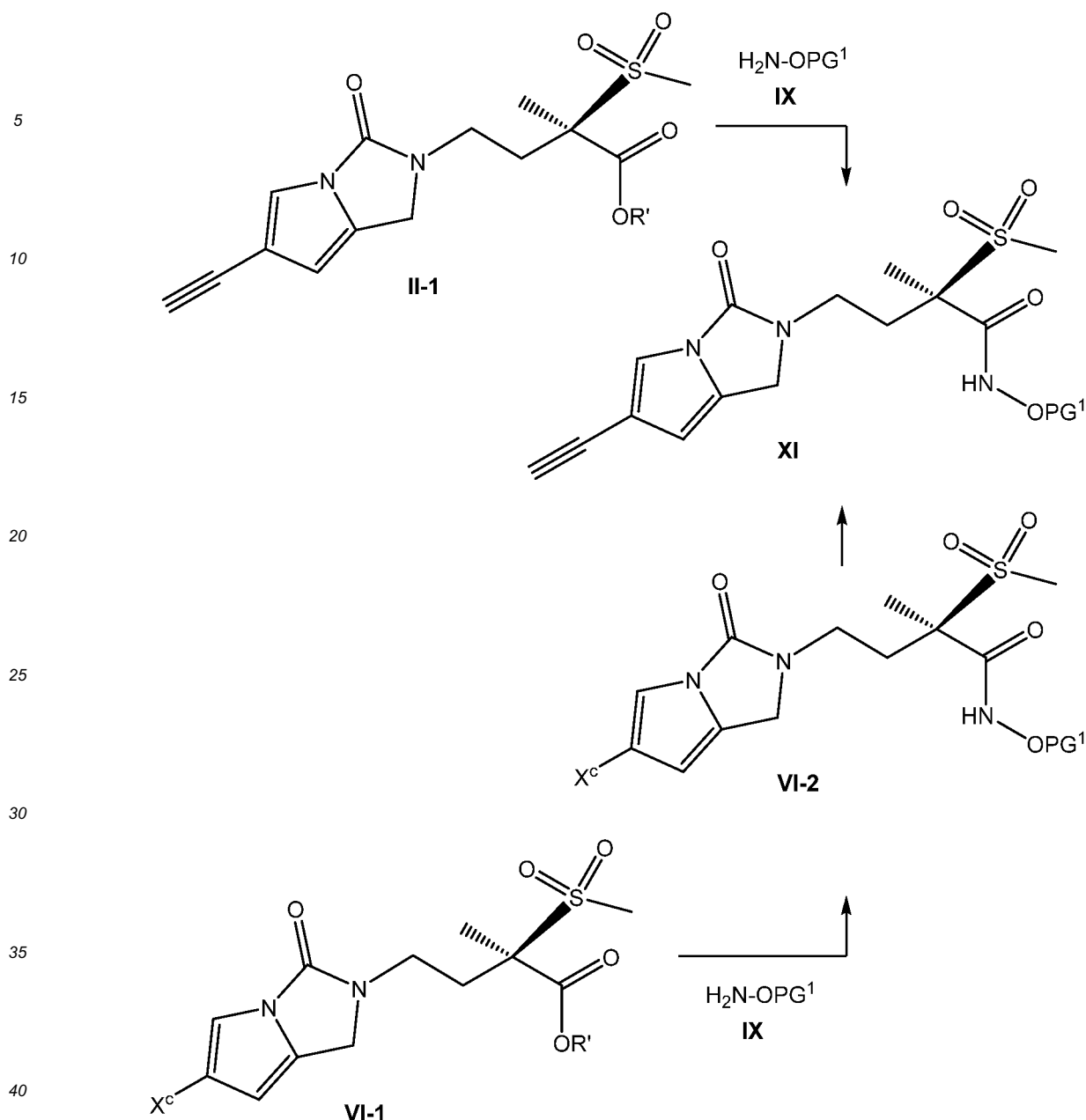
Scheme 6
