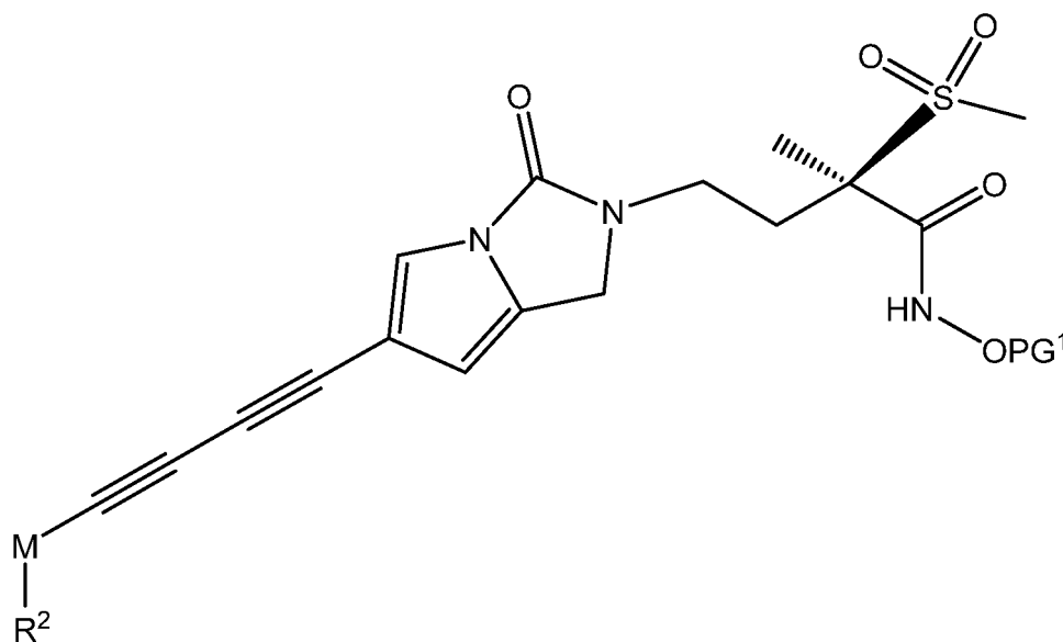
II
