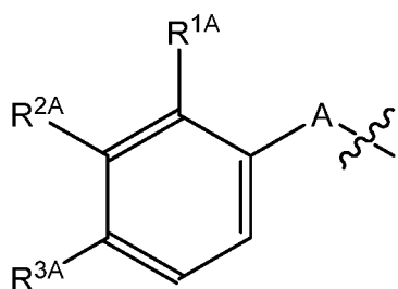
M A
