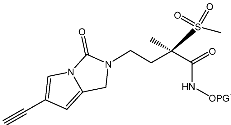
XI
