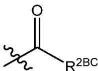
L^{2BC}
