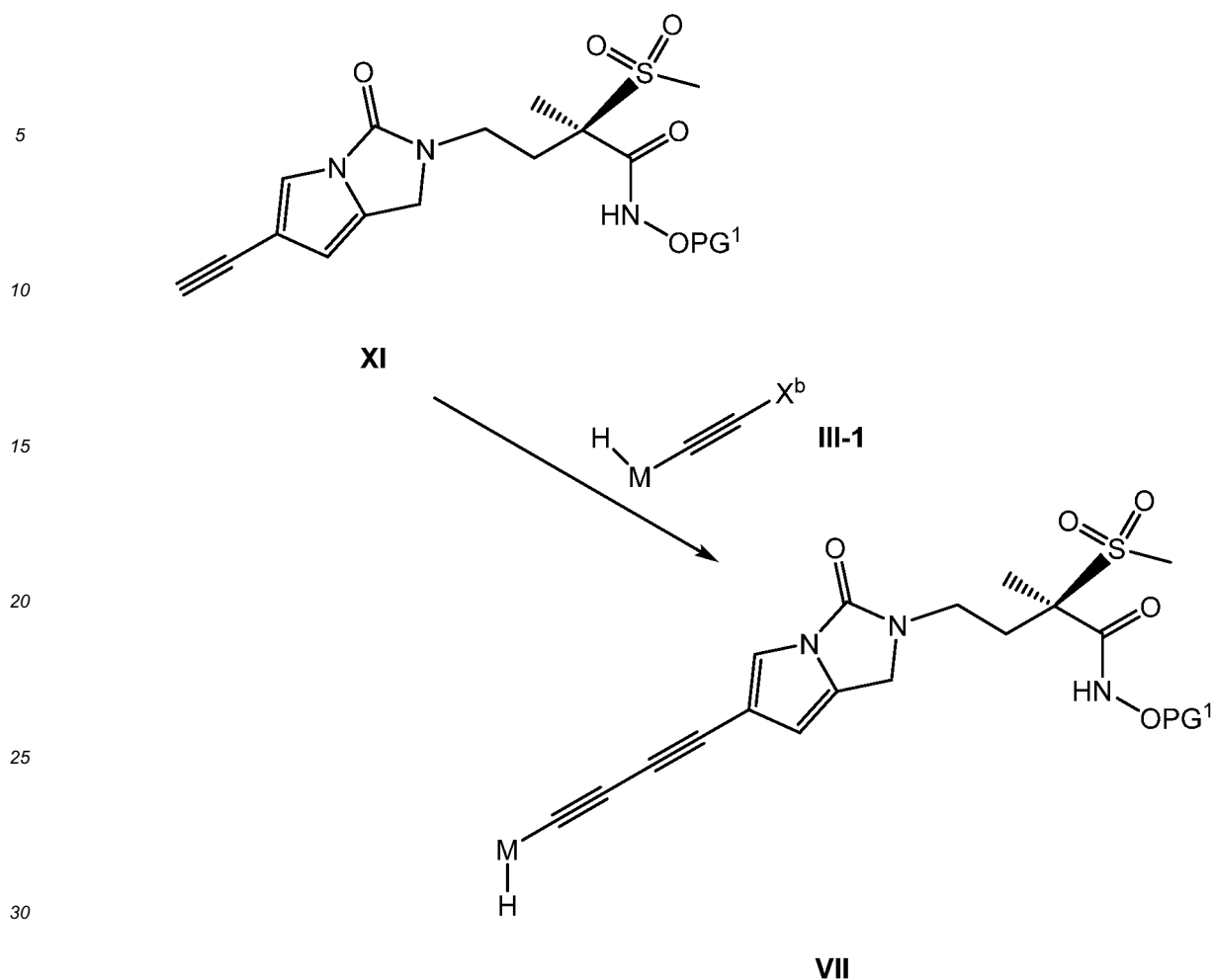
Scheme 3
