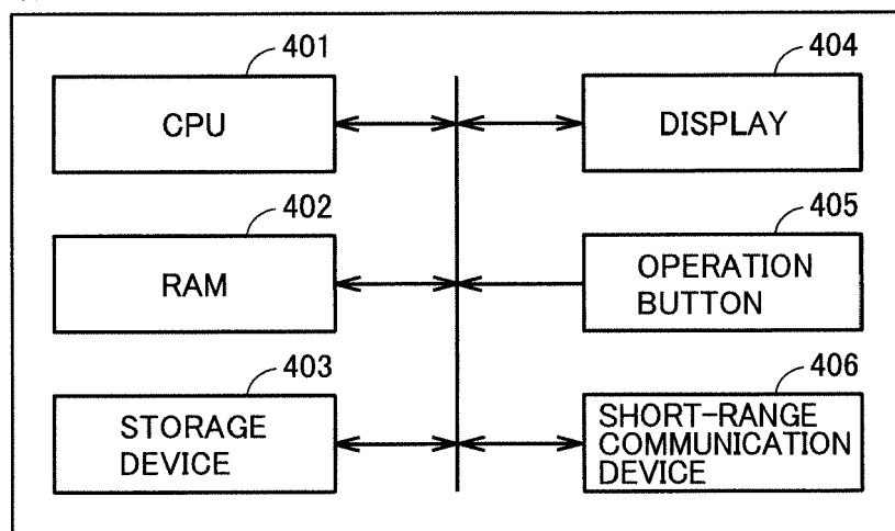
400 MOBILE TERMINAL
