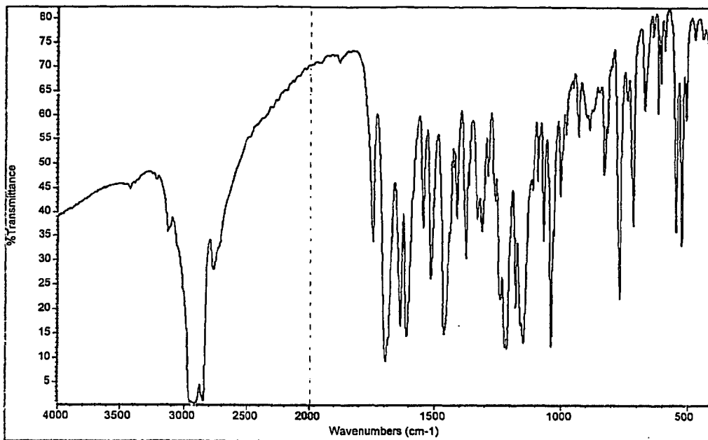
Figure 1 Infrared spectrum of the Mesylate Form I
