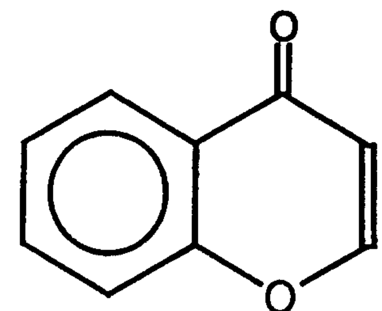
7-Methylcoumarin
