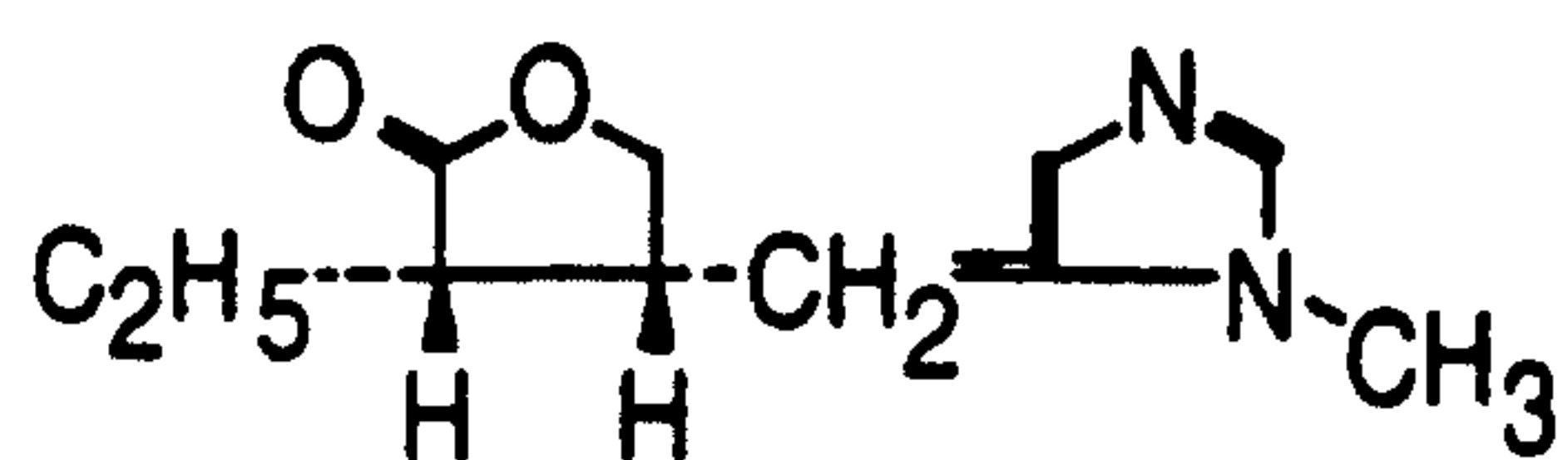
Pilocarpine
