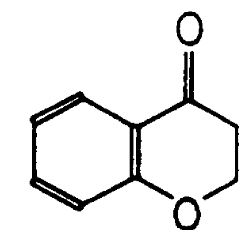
4-Chromanone
