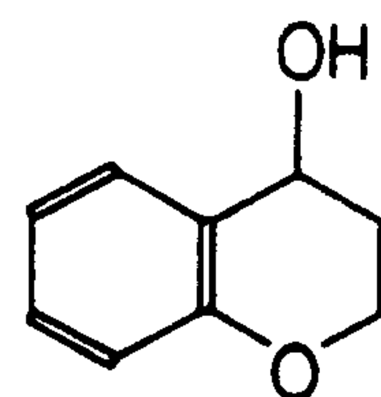
4-Chromanol
