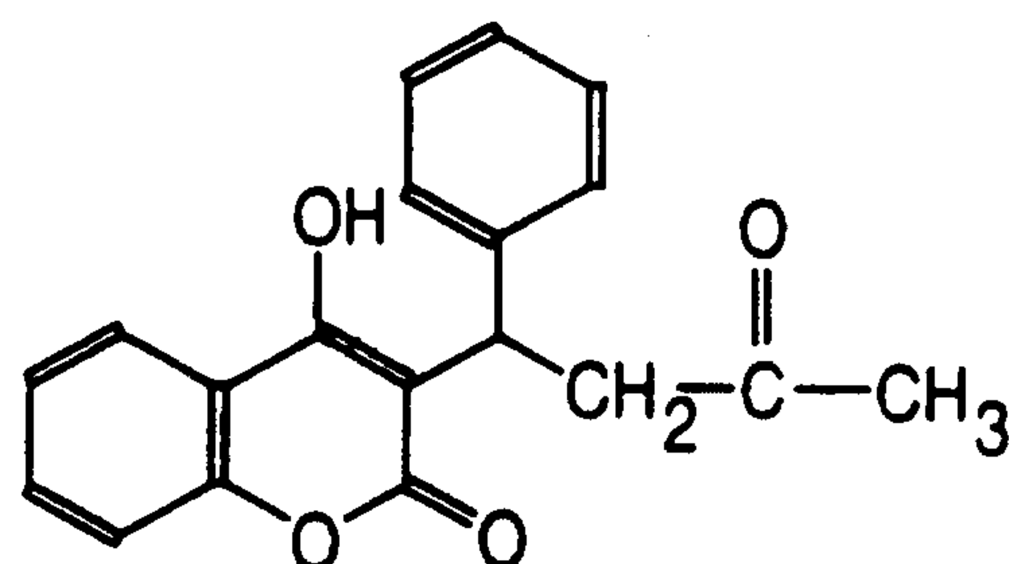
Warfarin
