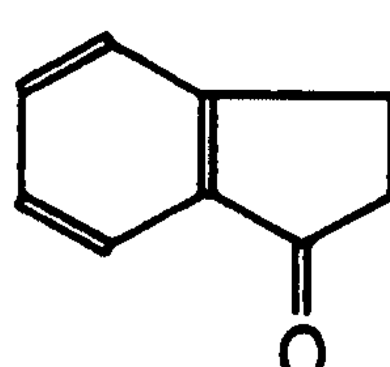
1-Indanone
