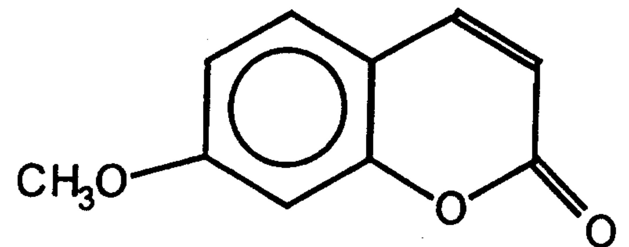
7-Methoxycoumarin
