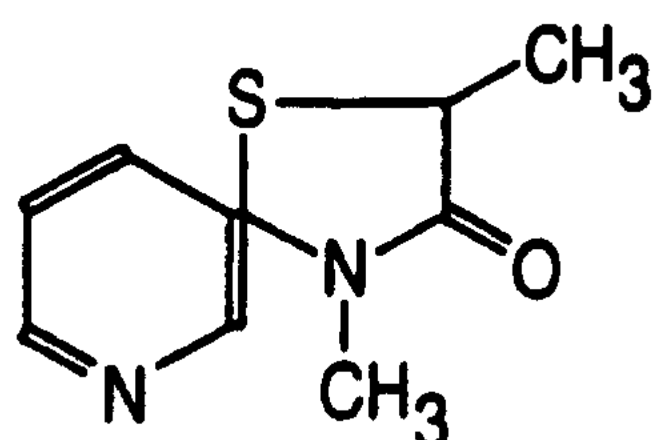
SM-12502
