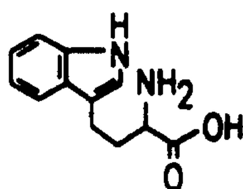
Tryptophan
