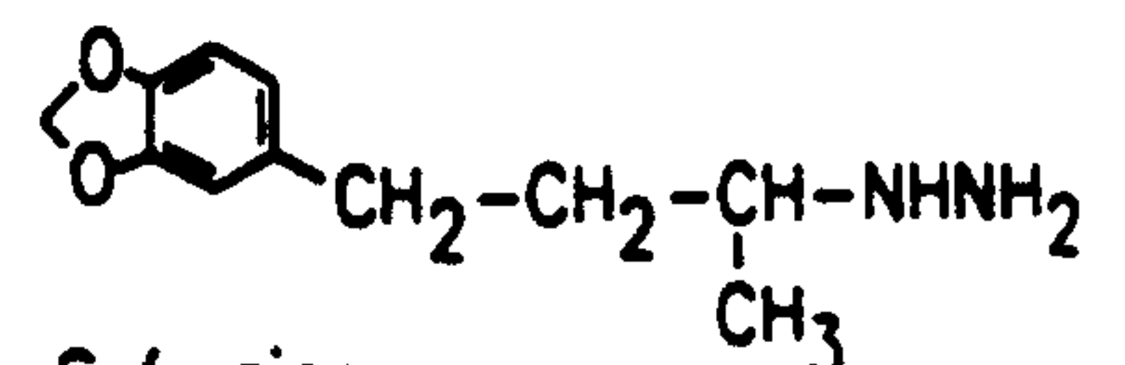
Safrozine
