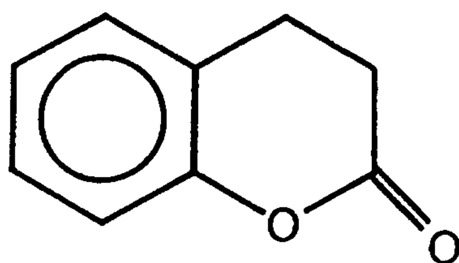
Dihydrocoumarin
