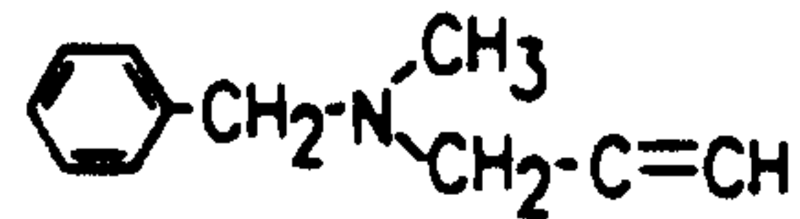
Pargyline
