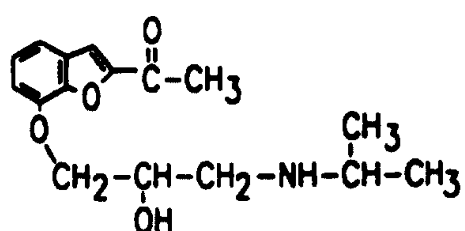
Betunoil
