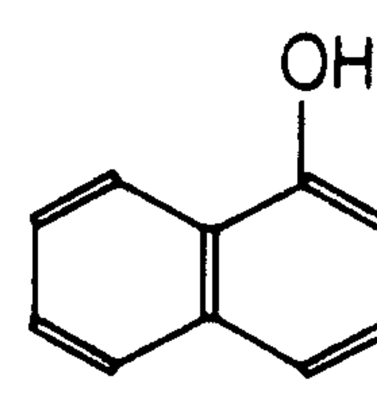
1-Naphthol
