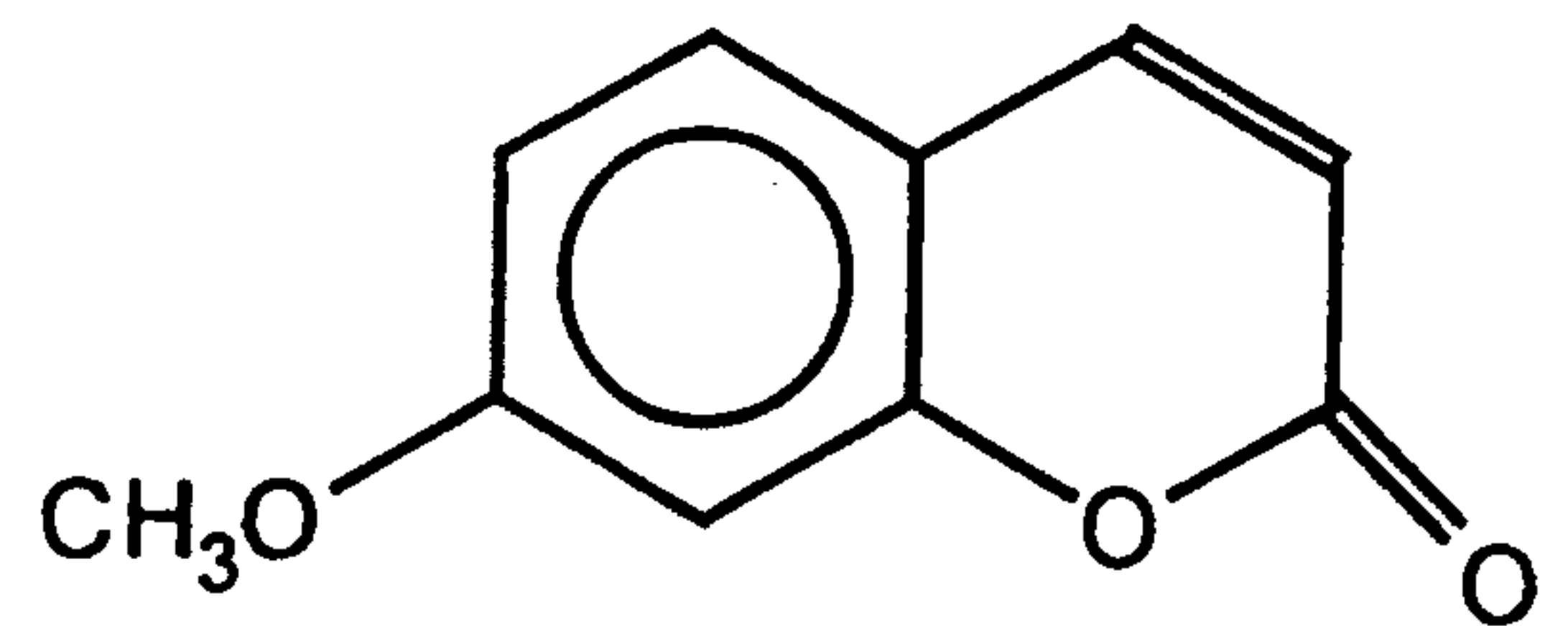
7-Methylcoumarin
