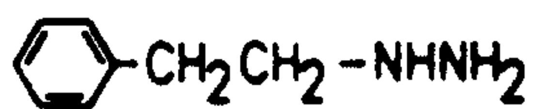
Phenelzine
