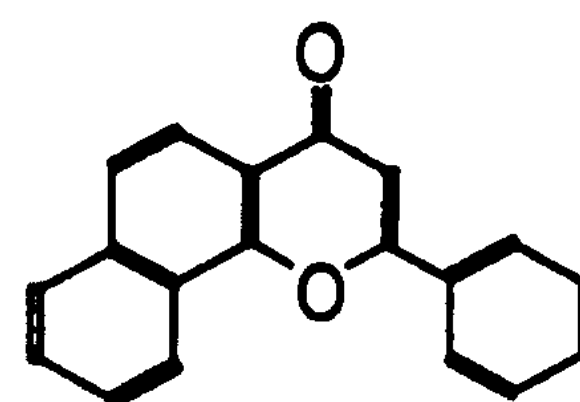
6-Aminochrysene
