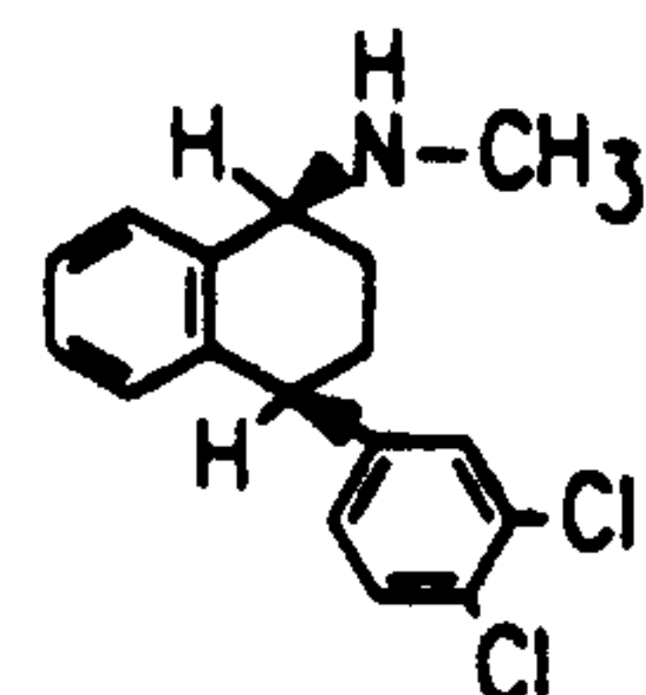
Sertraline
