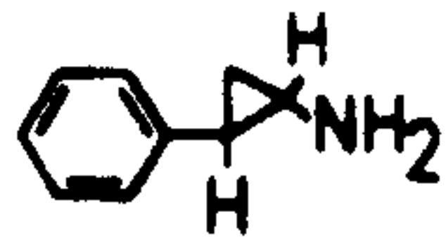
Tranylcypromine
