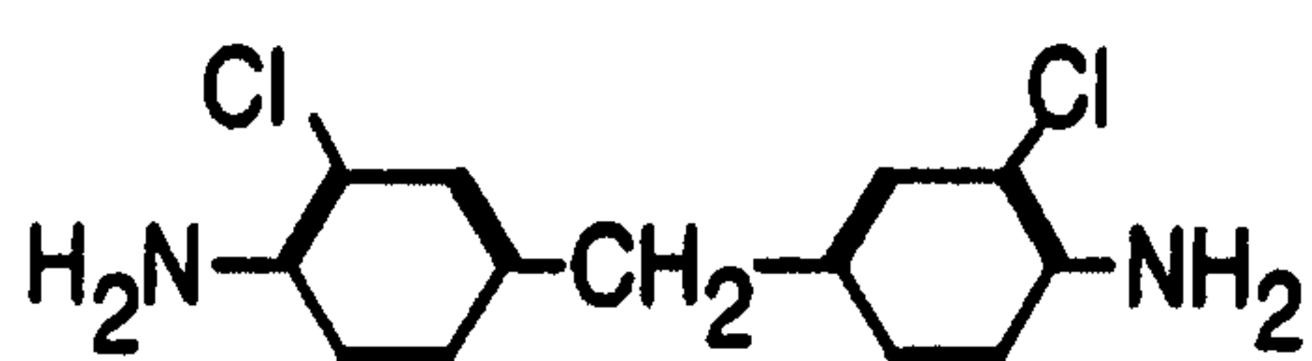
4,4'-Methylene bis[2-chloroaniline
