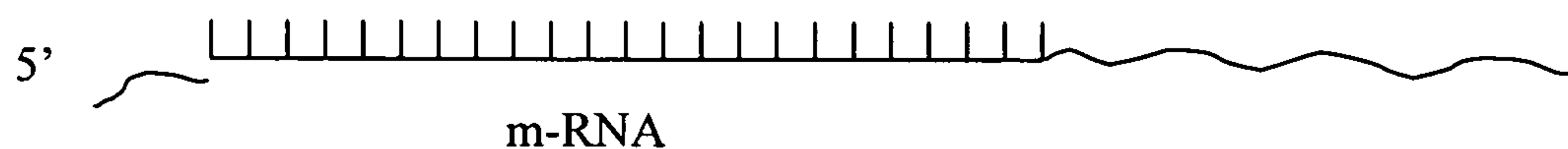
Diagram (2). (m-RNA Complementary to antisense strand)
