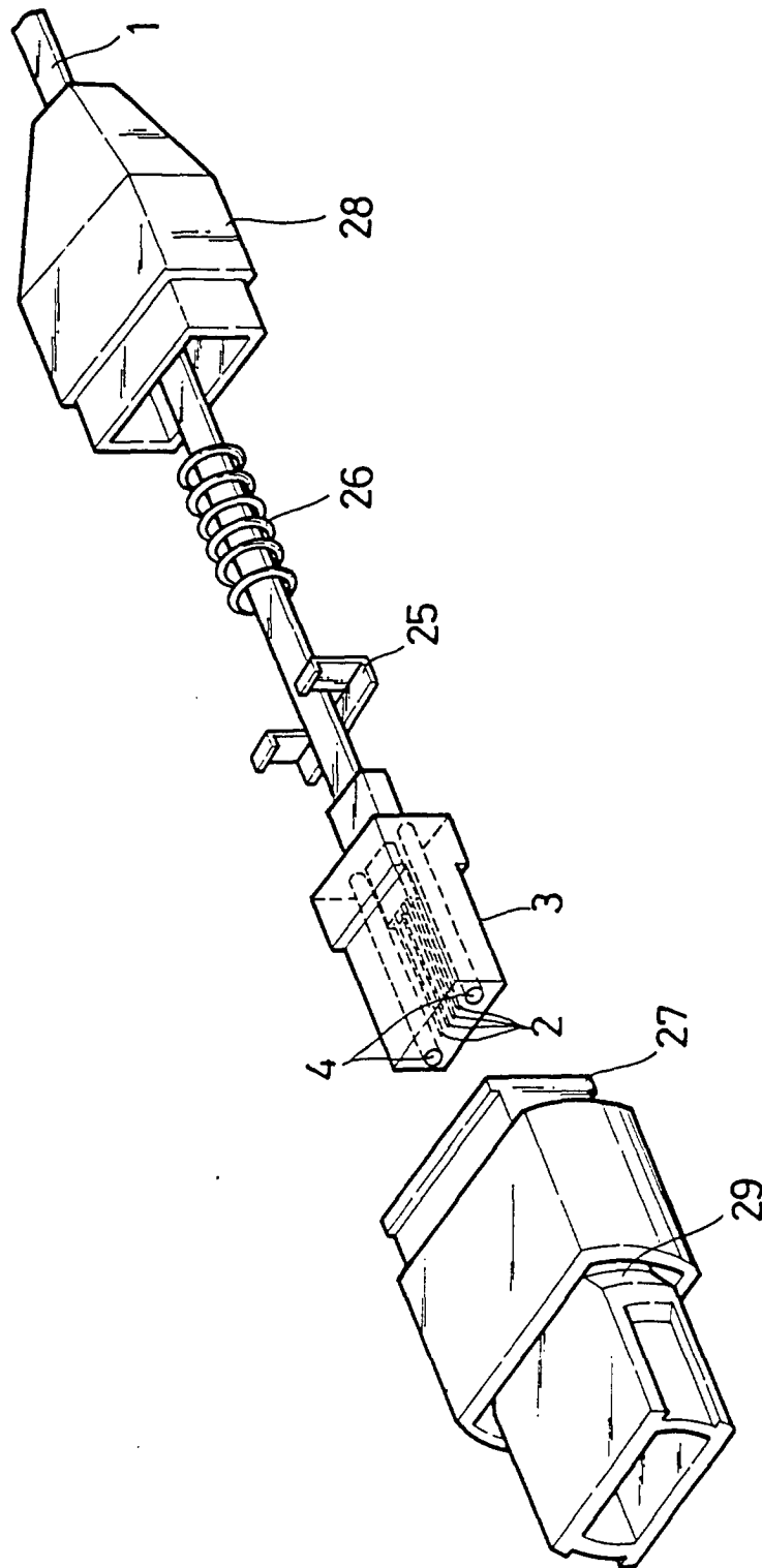
FIG. 10 PRIOR ART
