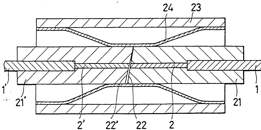
FIG. 8 PRIOR ART
