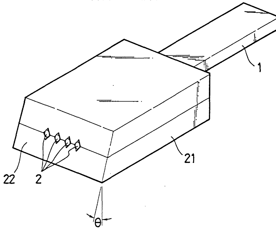
FIG. 7 PRIOR ART
