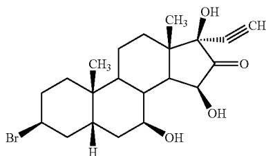
subgroup 12-1, compound 4.2.2.3,
