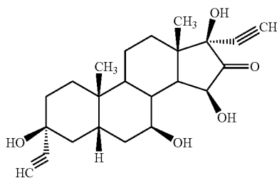
subgroup 13-1, compound 4.2.2.3,
