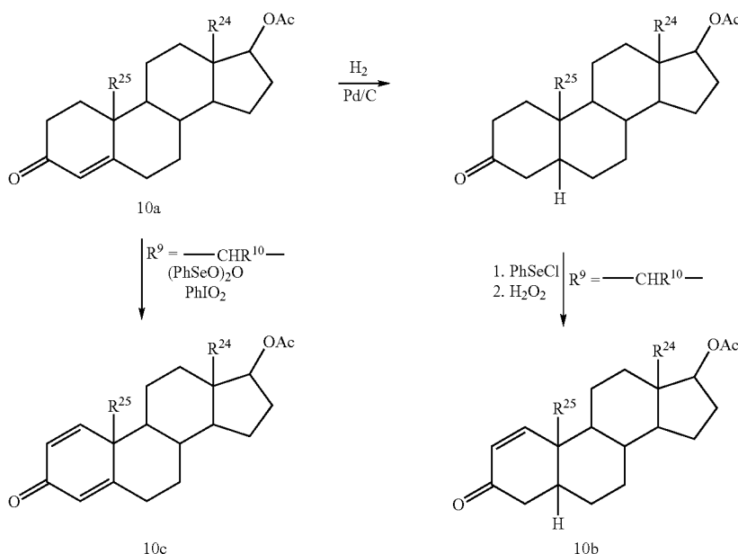
Scheme 10
