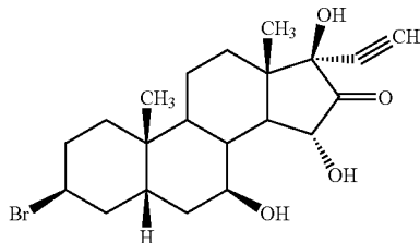
subgroup 12-2, compound 4.2.2.3.
