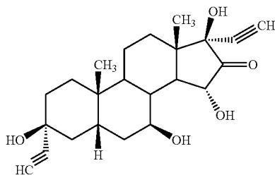
subgroup 13-2, compound 4.2.2.3.
