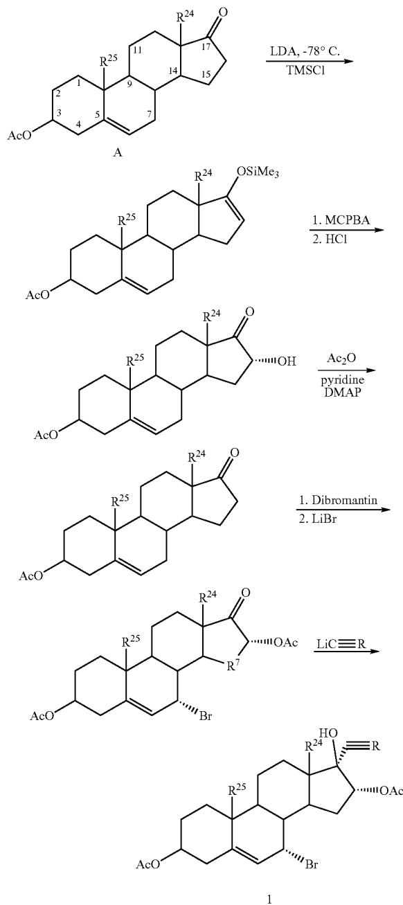
Scheme 1
