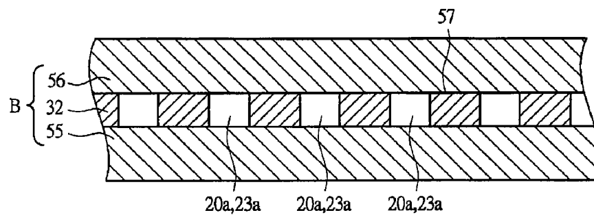
FIG. 11C Second slurry application step: Electrode B
