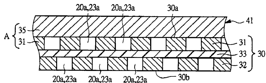
FIG. 6B First slurry application step: Electrode B
