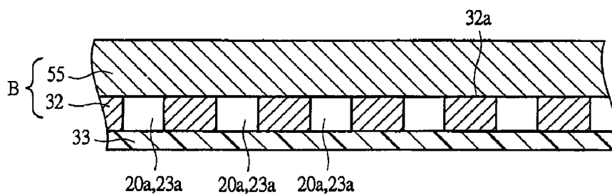
FIG. 11A First slurry application step: Electrode B
