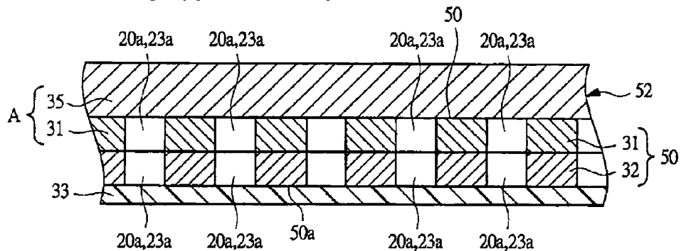
FIG. 10A First slurry application step: Electrode A
