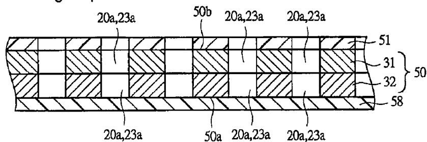
FIG. 12D Etching step
