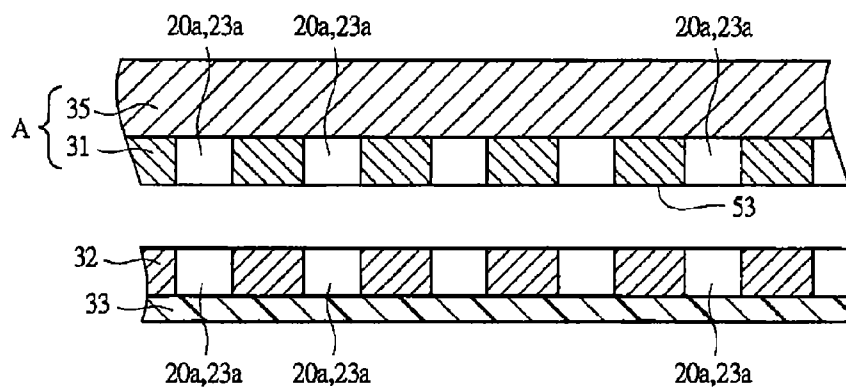
FIG. 10B Current collector separating step
