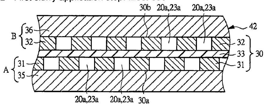
FIG. 6C Current collector separating step
