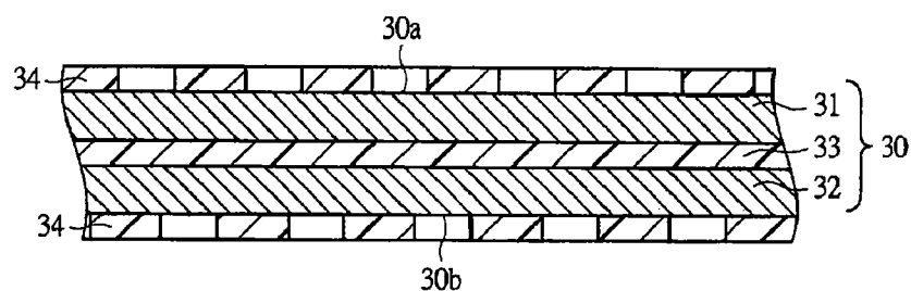
FIG. 5C Etching step
