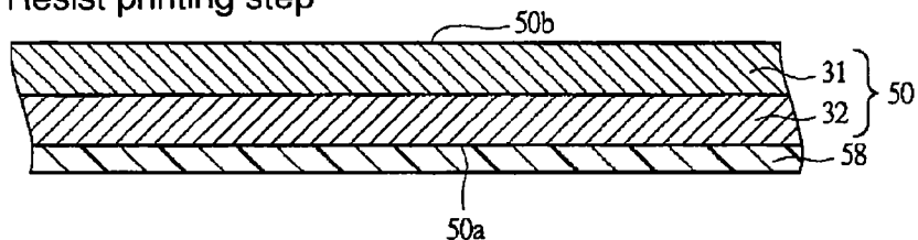
FIG. 12C Resist printing step
