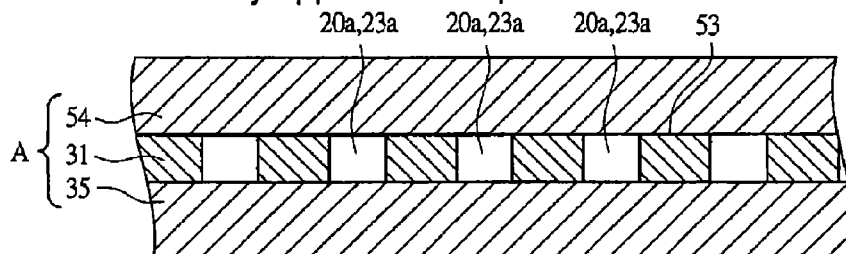
FIG. 10C Second slurry application step: Electrode A
