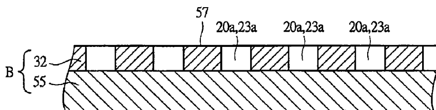
FIG. 11B Film separating step
