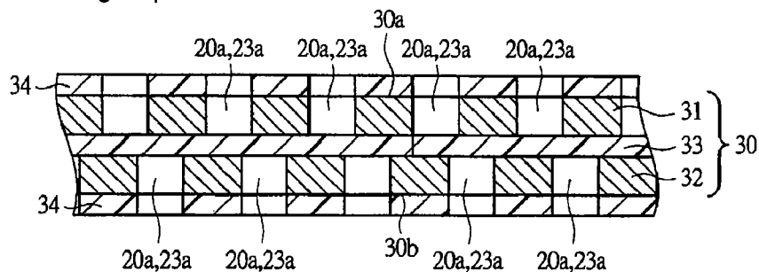
FIG. 5C Etching step
