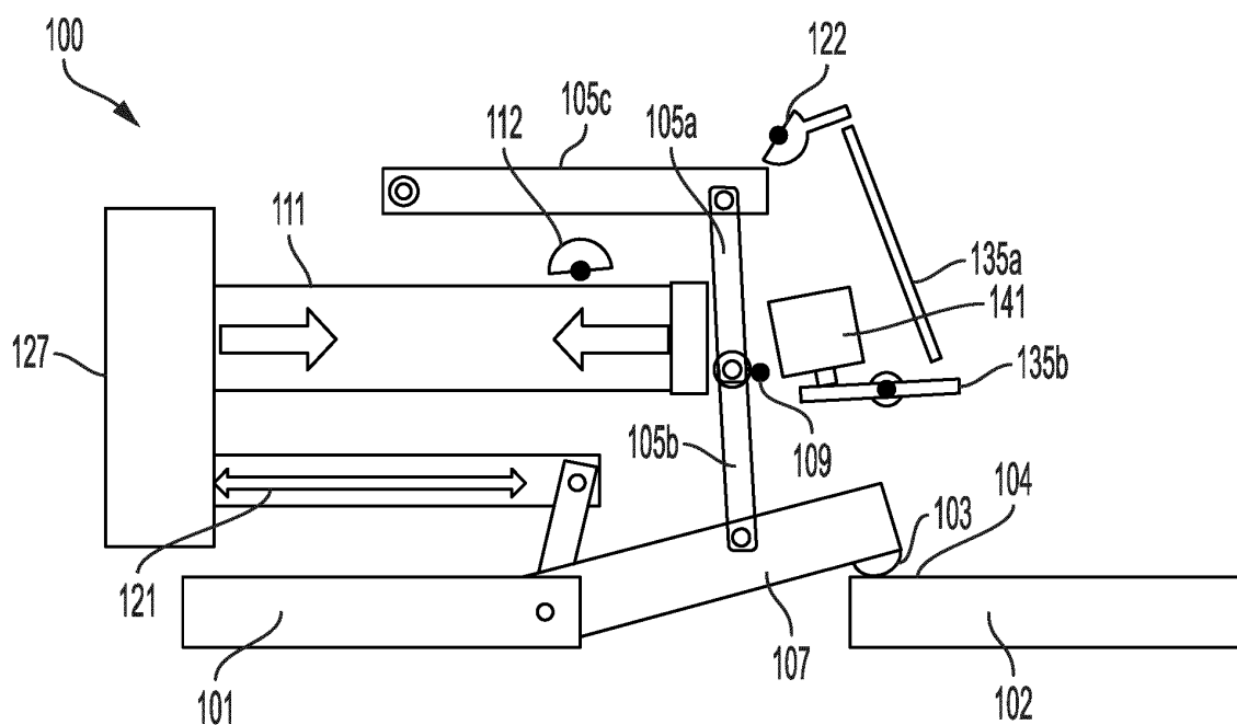
FIG. 1C PRIOR ART
