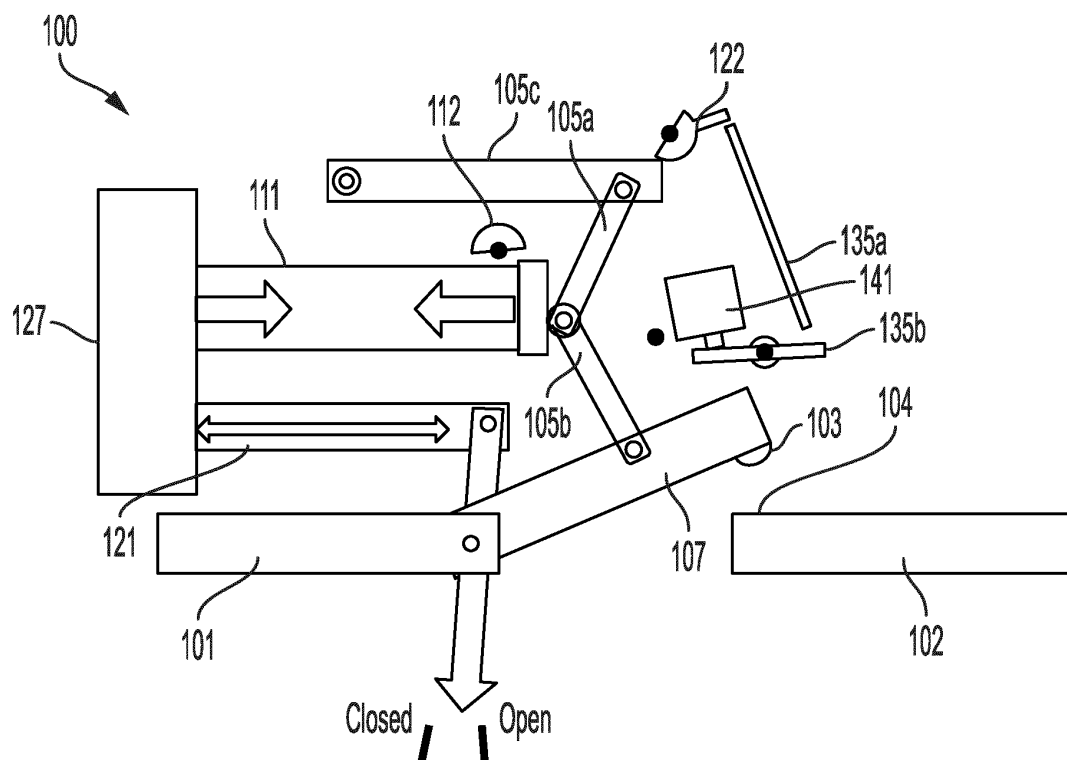
FIG. 1C PRIOR ART
