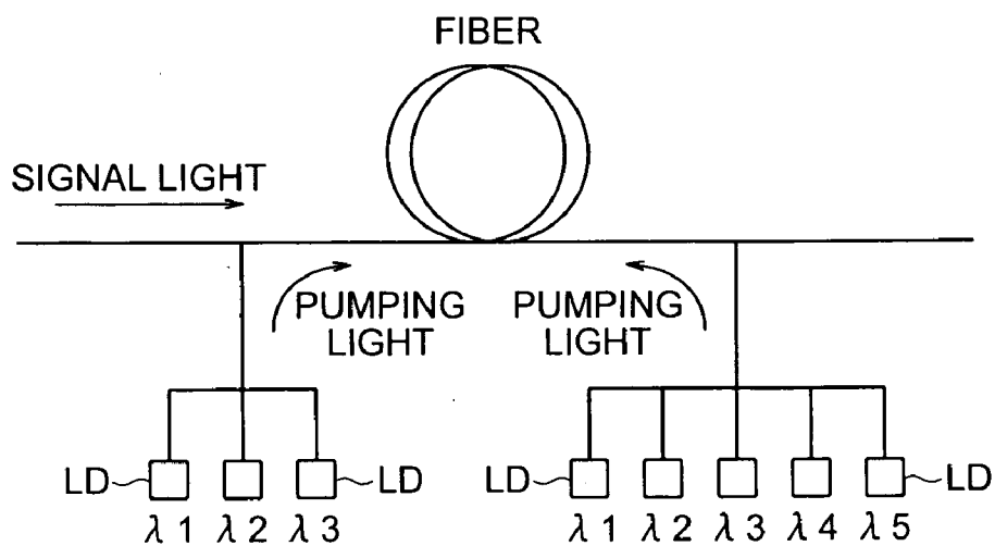
STRUCTURAL DIAGRAM OF BIDIRECTIONAL PUMPING
