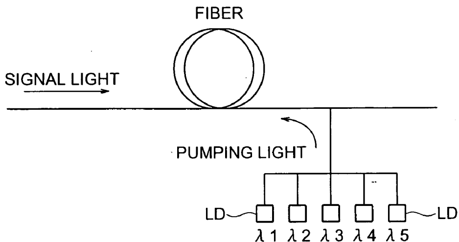
STRUCTURAL DIAGRAM OF BACKWARD PUMPING
