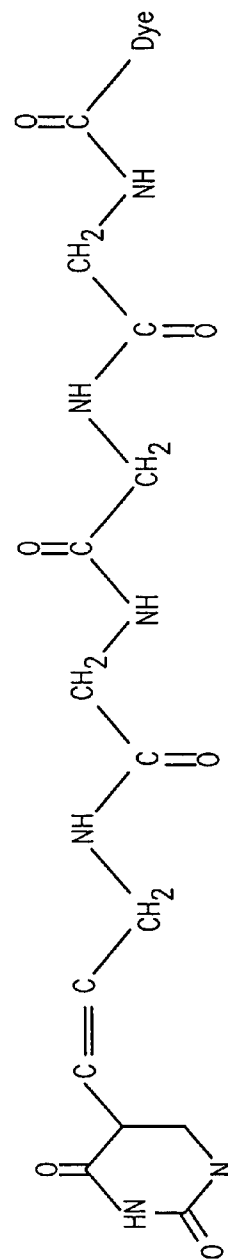
Tetraglycinyl linker
