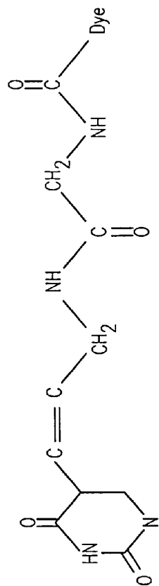
Diglycinyl linker
