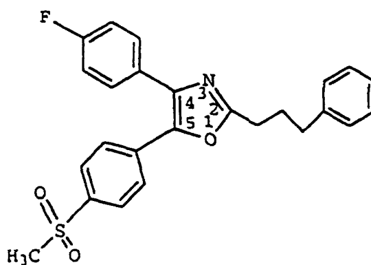
4-(4-Fluorophenyl)-5-[4-methylsulfonylphenyl]-2-(3-phenylpropyl)oxazole
