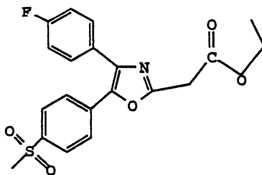
Ethyl 2-[4-(4-fluorophenyl)-5-(4- methylsulfonylphenyl)oxazol-2-yl]acetate
