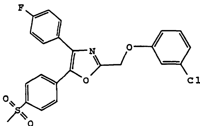
4 - ( 4 - Fluorophenyl ) - 2 - ( 3 - chlorophenoxy methyl ) - 5 - [ 4 - ( methylsulfonyl ) phenyl ] oxazole
