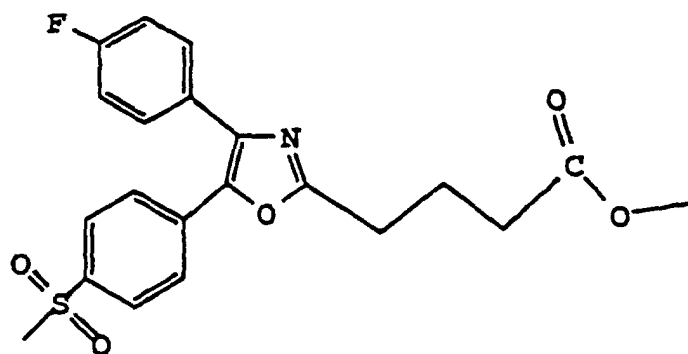
Methyl 4-[4-(4-fluorophenyl)-5-[4-methylsulfonylphenyl]oxazol-2-yl]butanoate
