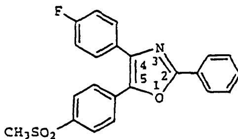
4-(4-Fluorophenyl)-5-[4-(methylsulfonyl)phenyl]-2-phenyloxazole
