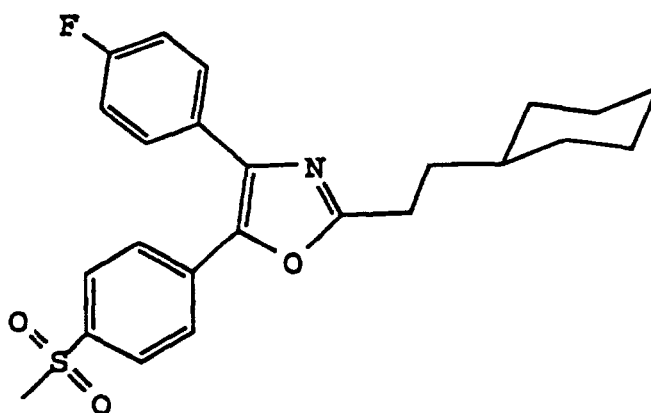
4 - ( 4 - Fluorophenyl ) - 2 - ( cyclohexylethyl ) - 5 - [ 4 - ( methylsulfonyl ) phenyl ] oxazole
