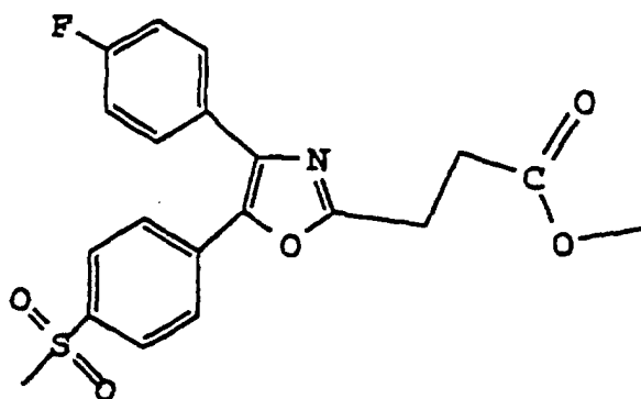
Methyl 3-[4-(4-fluorophenyl)-5-[4-methylsulfonylphenyl]oxazol-2-yl]propanoate
