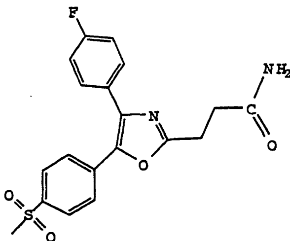
3 - [ 4 - ( 4 - Fluorophenyl ) - 5 - ( 4 - ( methylsulfonyl ) phenyl ) oxazol - 2 - yl ] propanamide
