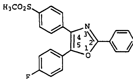
5 - ( 4 - Fluorophenyl ) - 2 - phenyl - 4 - [ 4 - ( methylsulfonyl ) phenyl ] oxazole
