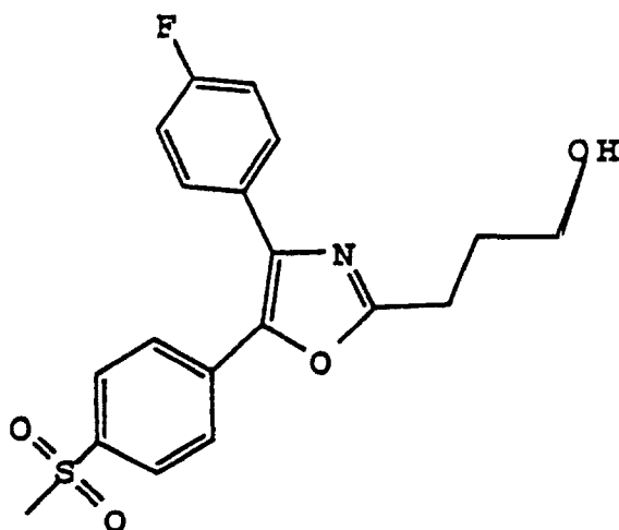
4 - ( 4 - Fluorophenyl ) - 2 - ( 3 - hydroxypropyl ) - 5 - [ 4 - ( methylsulfonyl ) phenyl ] oxazole
