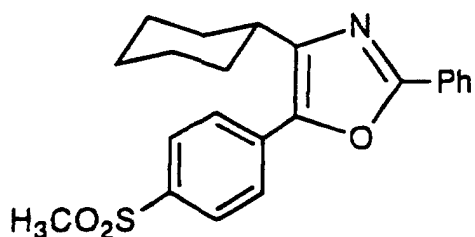
2-Phenyl-4-(cyclohexyl)-5-[4-(methylsulfonyl)phenyl]oxazole
