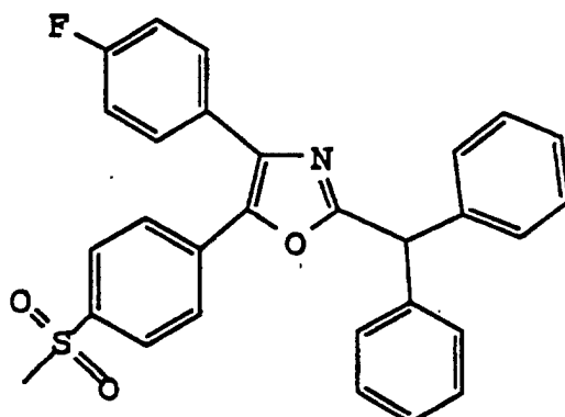
2-Diphenylmethyl-4-(4-fluorophenyl)- 5-[4-methylsulfonylphenyl]oxazole
