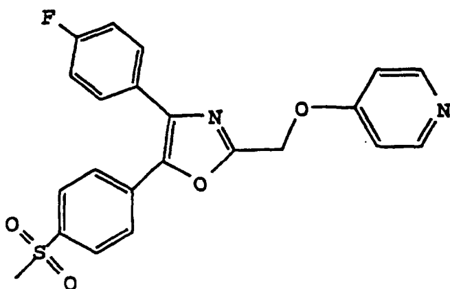
4 - ( 4 - Fluorophenyl ) - 2 - ( pyridyloxymethyl ) - 5 - [ 4 - ( methylsulfonyl ) phenyl ] oxazole
