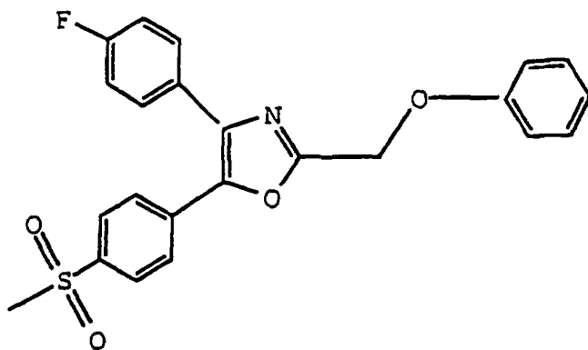
4 - ( 4 - Fluorophenyl ) - 5 - [ 4 - ( methylsulfonyl ) phenyl ] - 2 - phenoxymethyloxazole
