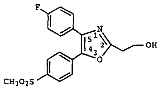
4 - ( 4 - Fluorophenyl ) - 2 - ( 2 - hydroxyethyl ) - 5 - [ 4 - ( methylsulfonyl ) phenyl ] oxazole
