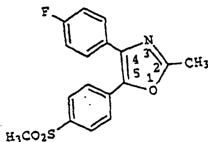
4-(4-Fluorophenyl)-2-methyl-5-[4-(methylsulfonyl)phenyl]oxazole
