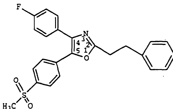
4 - ( 4 - Fluorophenyl ) - 2 - ( 2 - phenylethyl ) - 5 - ( 4 - ( methylsulfonyl ) phenyl ) oxazole
