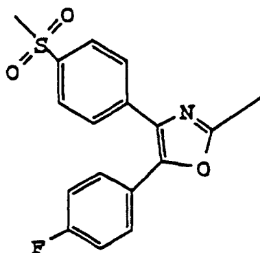
5-(4-Fluorophenyl)-2-methyl-4-[4-(methylsulfonyl)phenyl]oxazole
