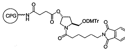
IV. Hydroxyproline-Amine Icaa CPG
