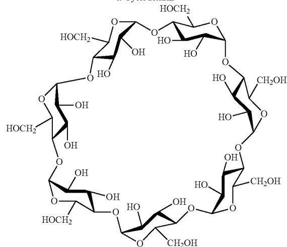
\beta -Cyclodextrin
