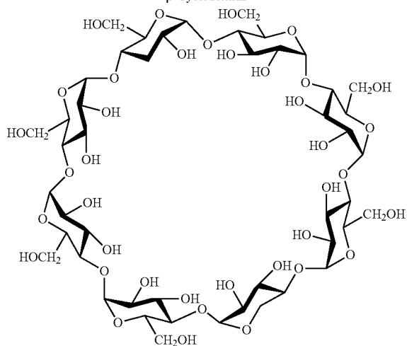
\gamma -Cyclodextrin
