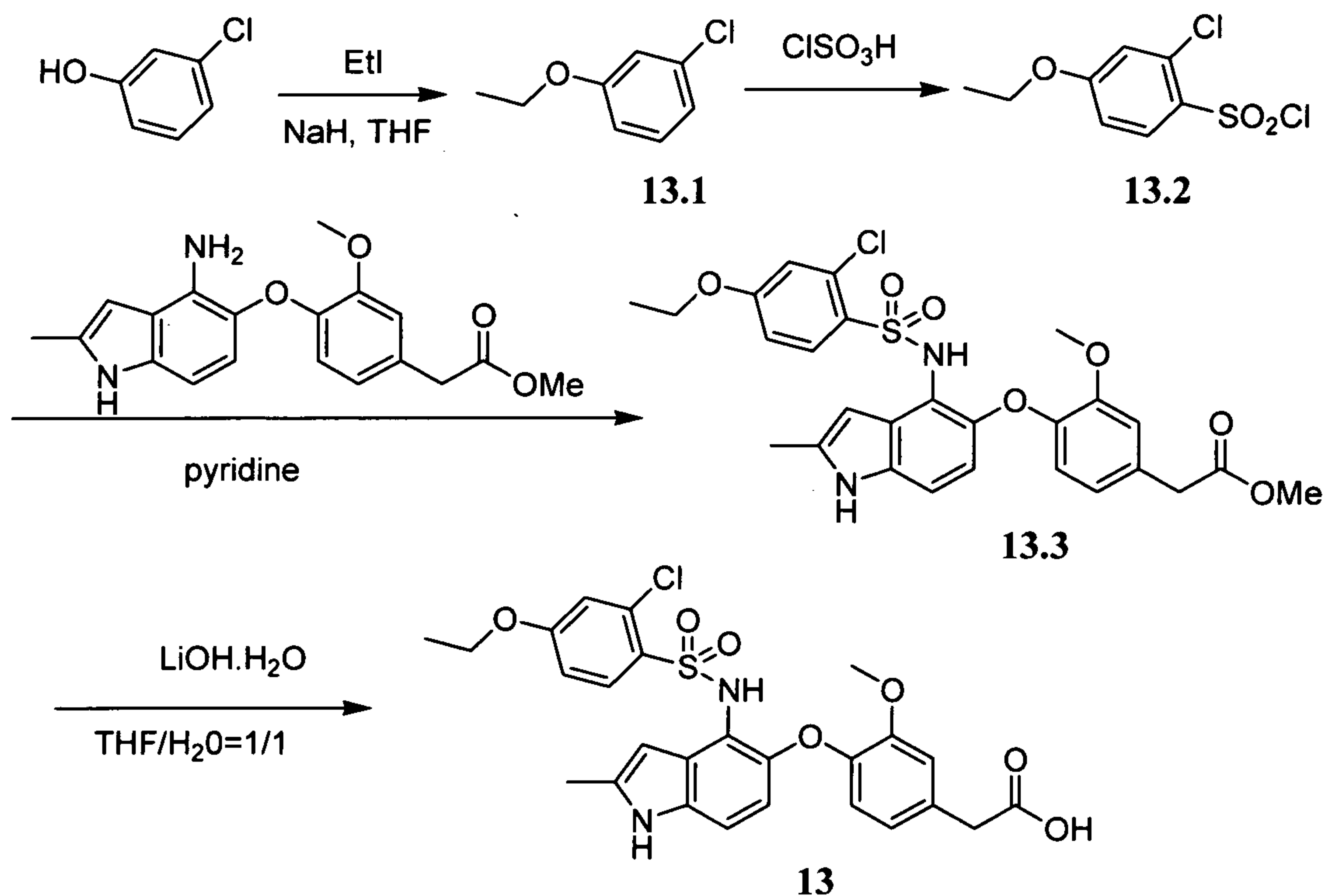
Scheme 13
