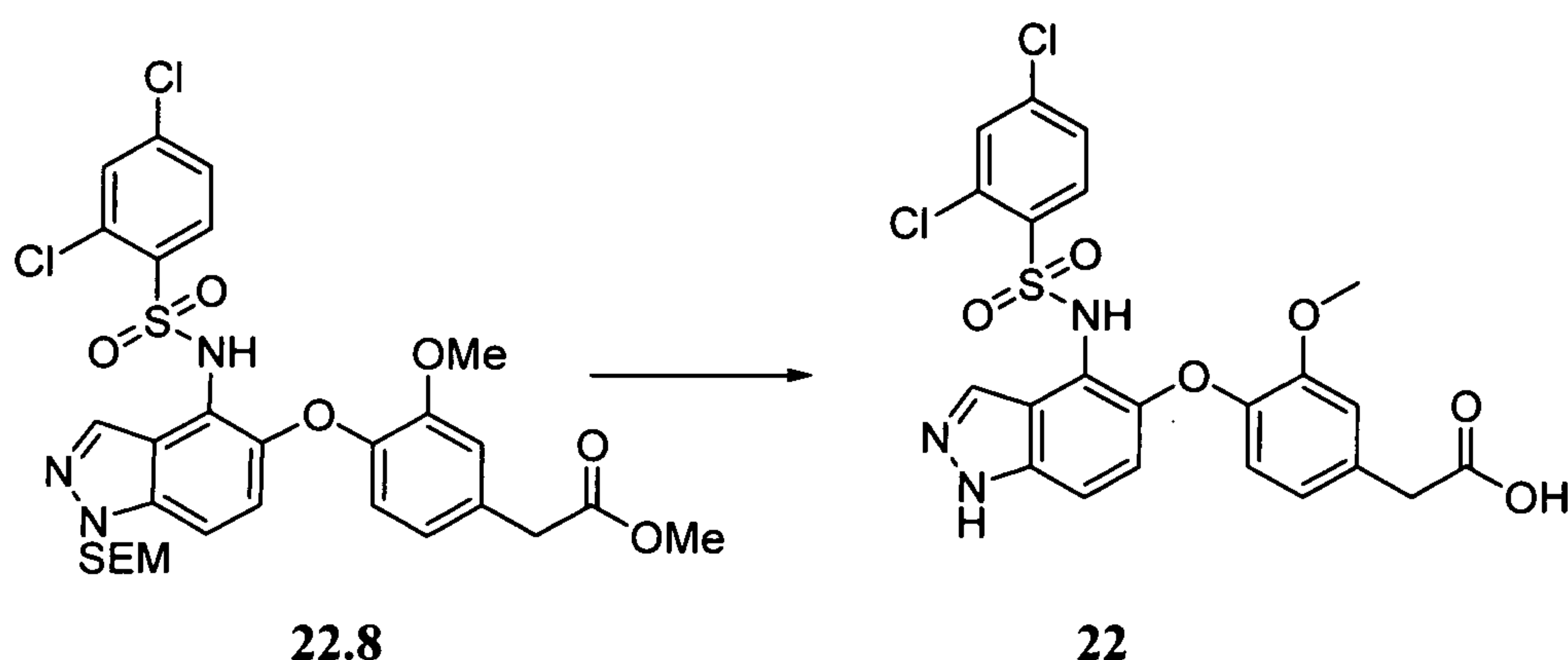
Scheme 22.9
