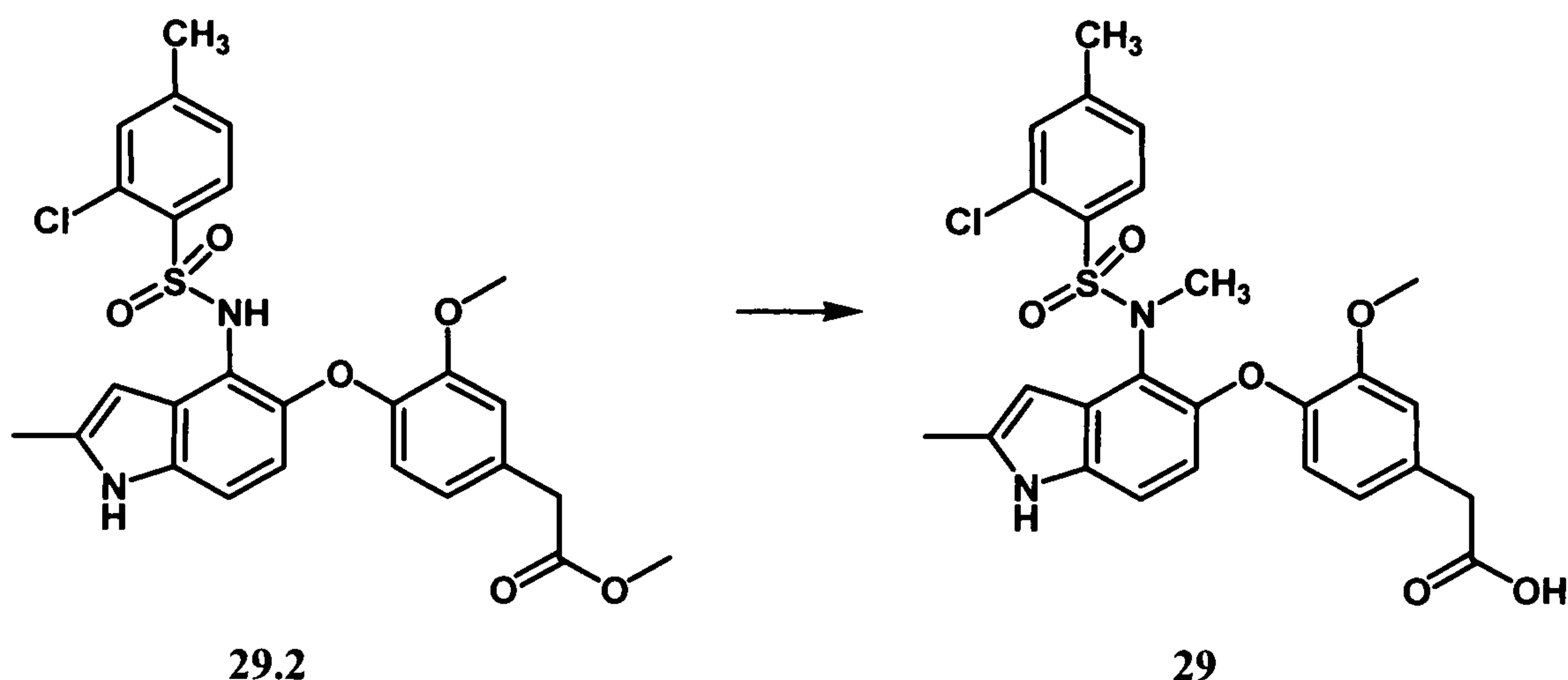
Scheme 29.3
