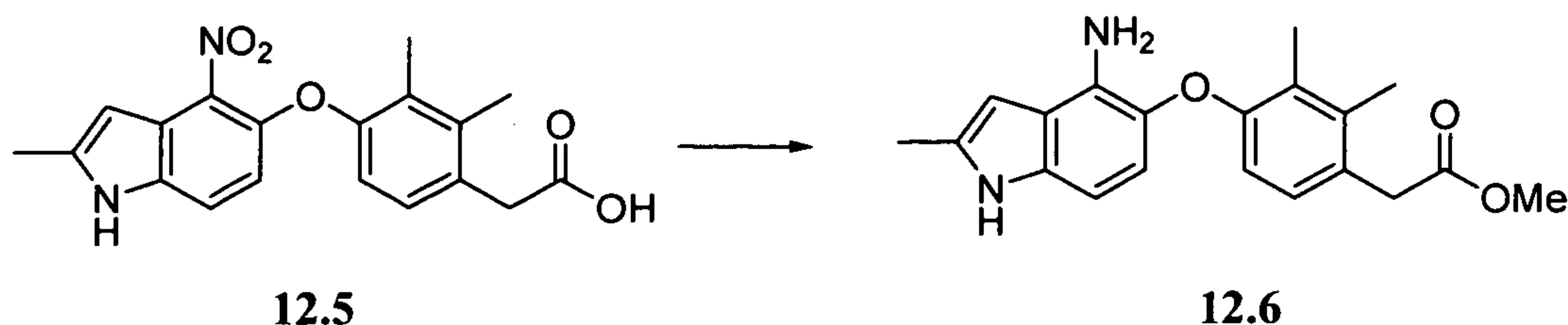
Scheme 12.6
