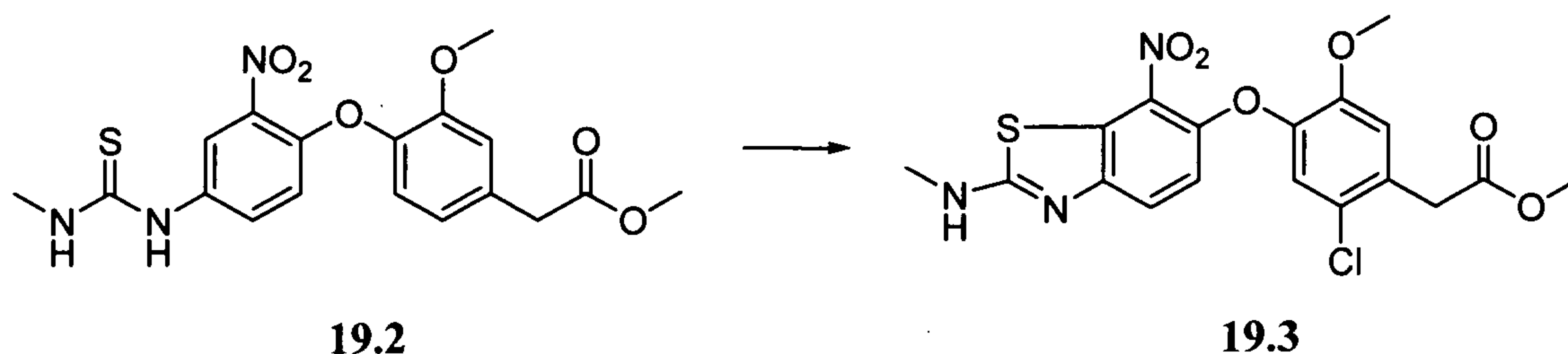
Scheme 19.2
