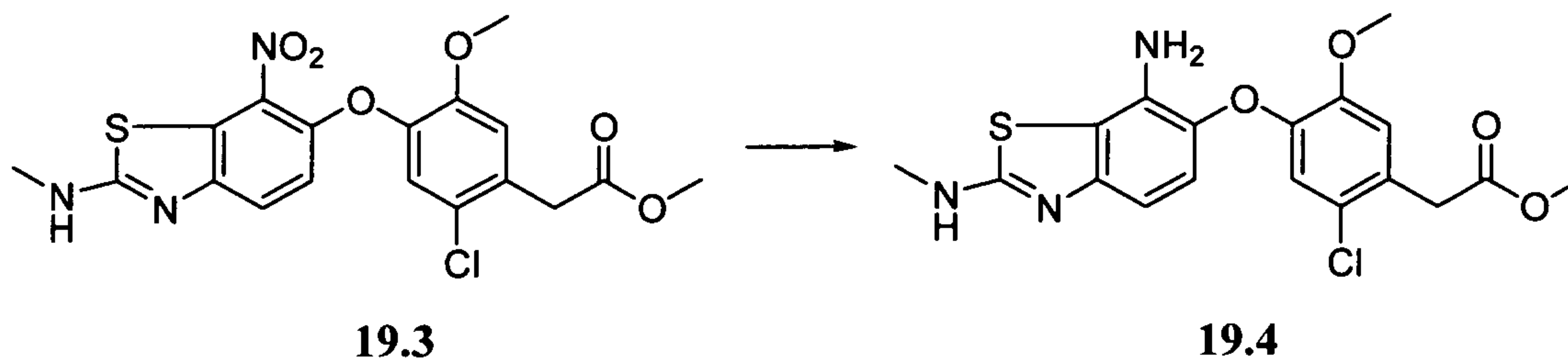
Scheme 19.3
