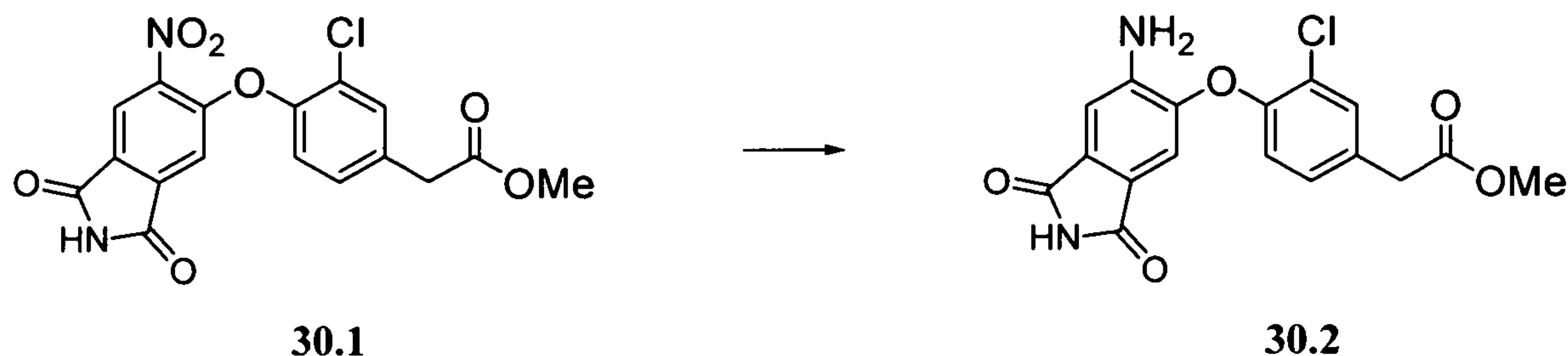
Scheme 30.2
