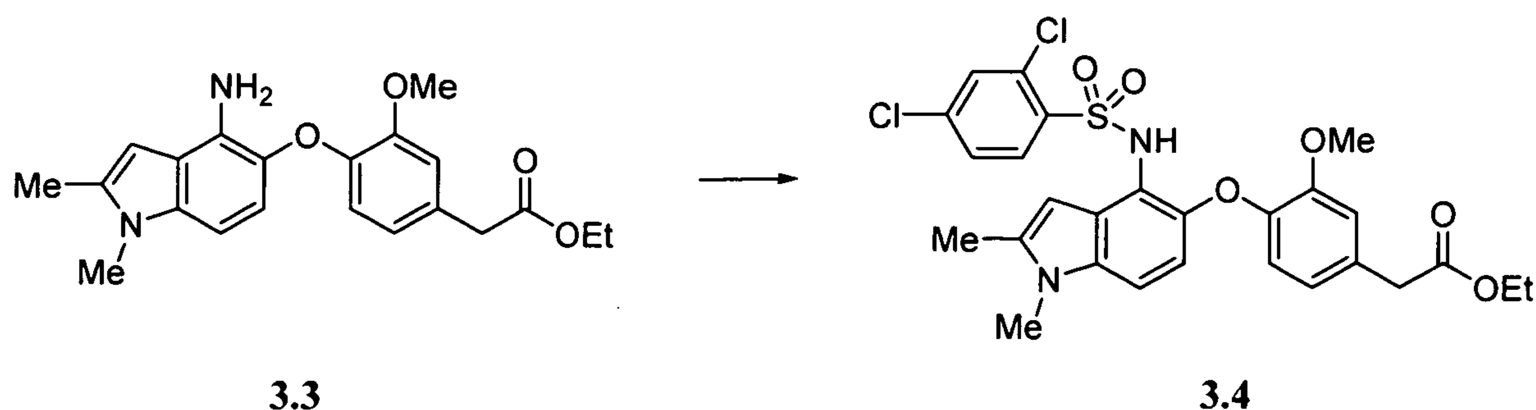
Scheme 3.4
