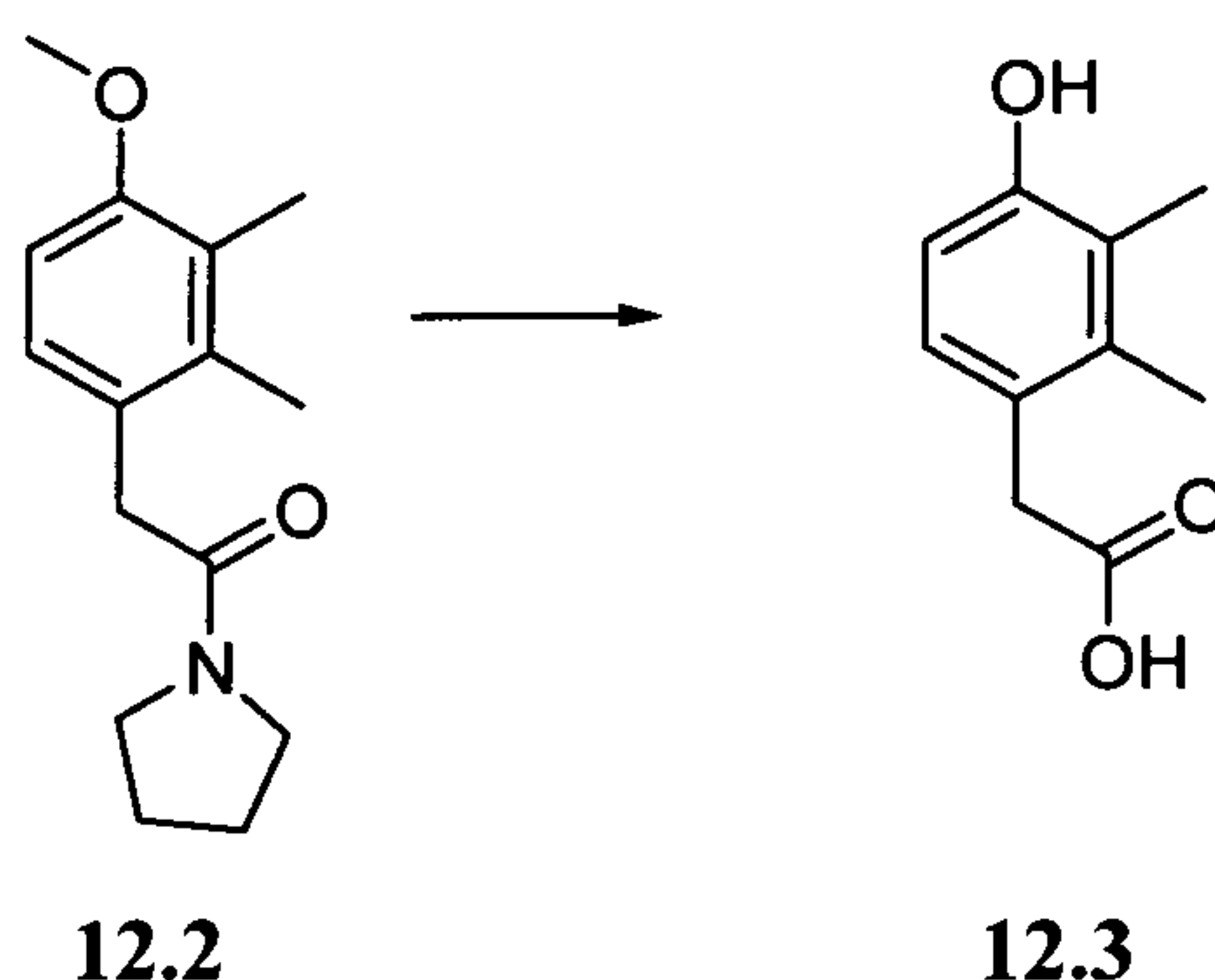
Scheme 12.3
