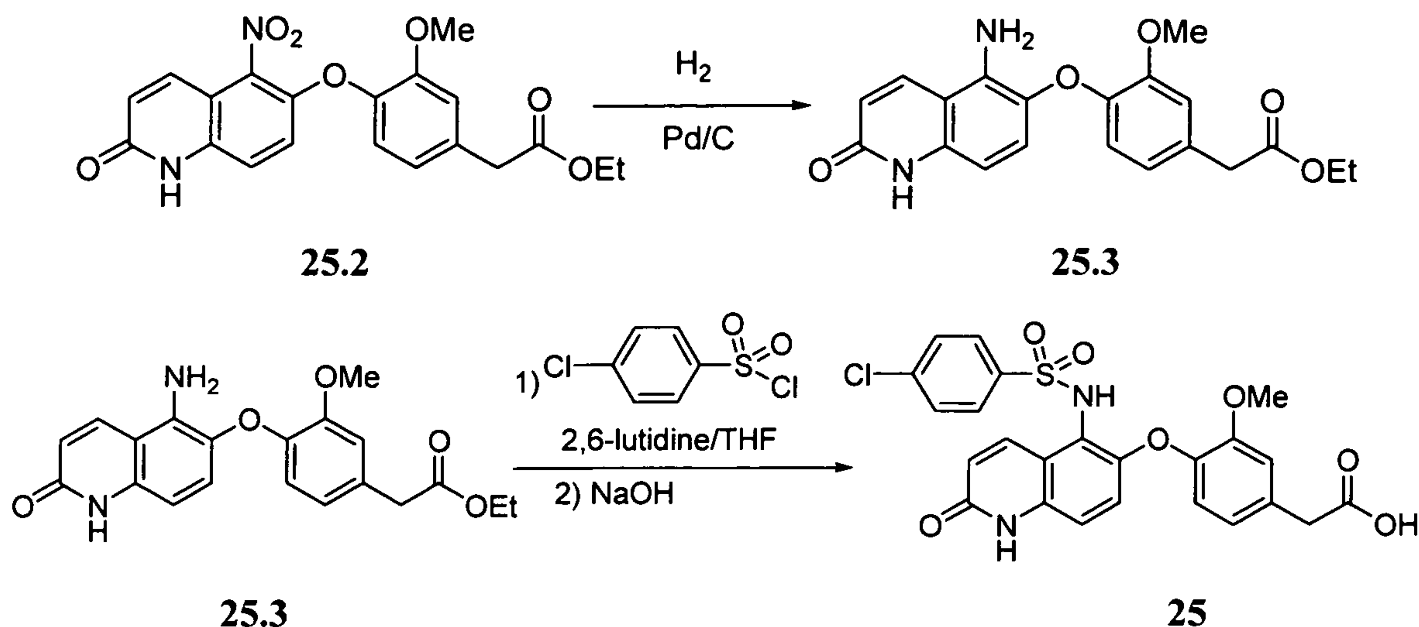
Scheme 25.2
