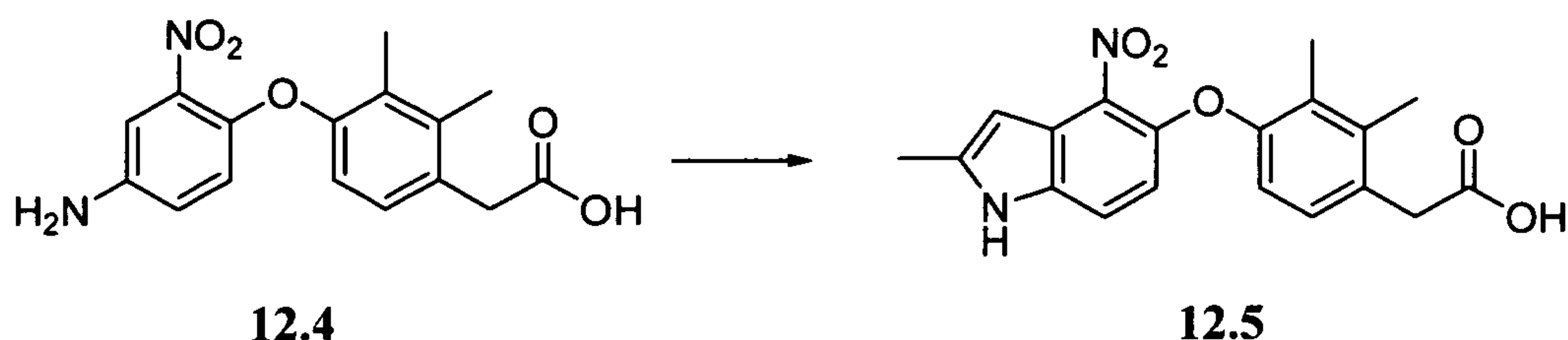
Scheme 12.5
