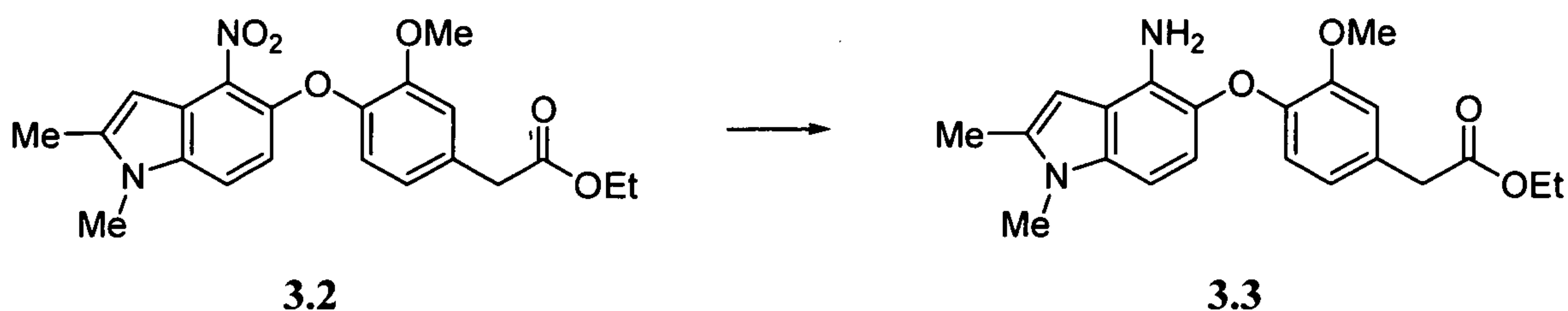
Scheme 3.3
