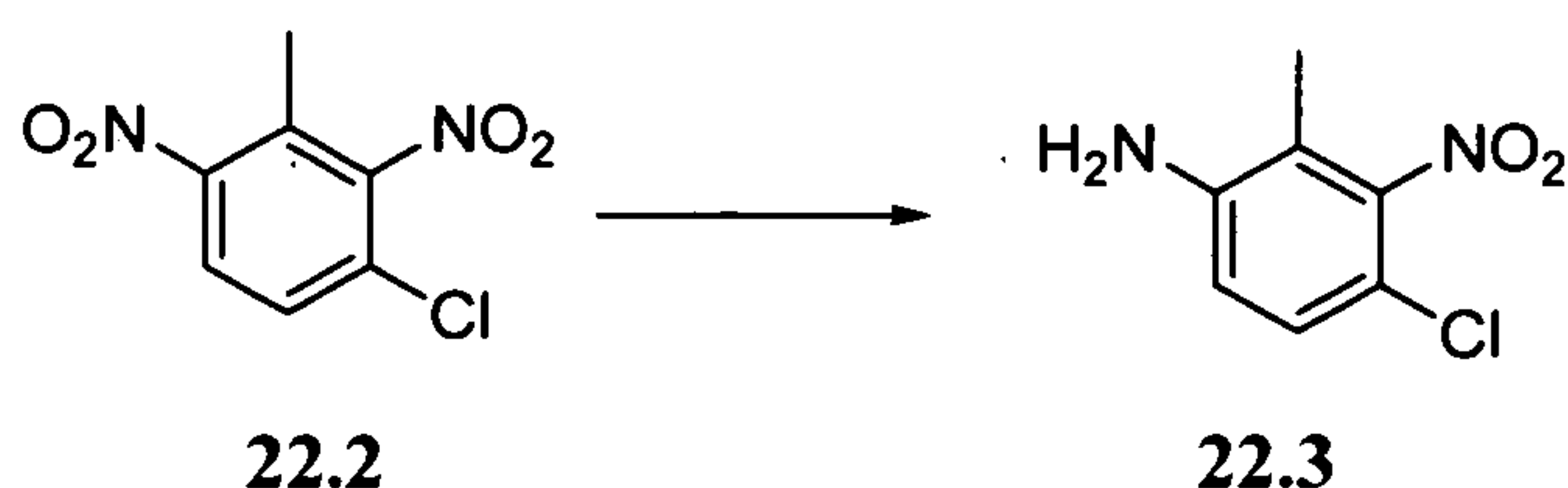
Scheme 22.3
