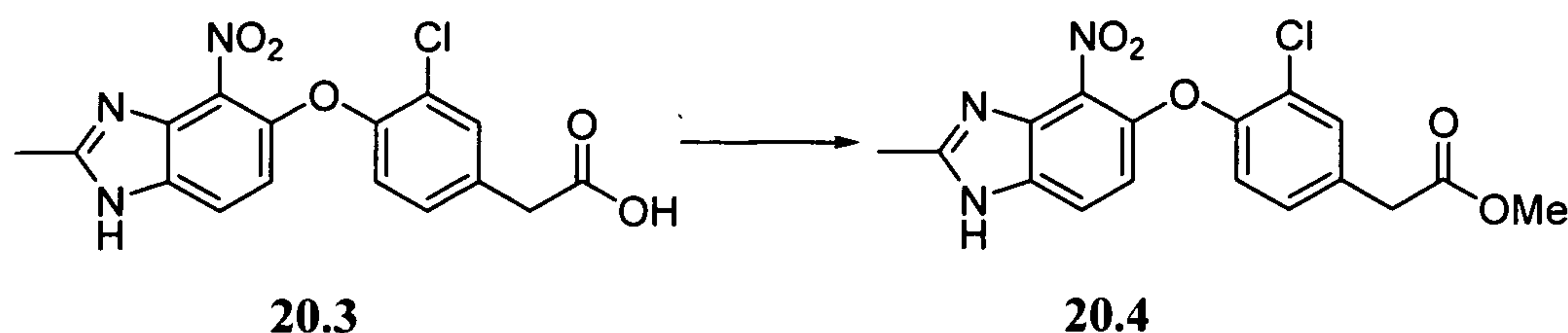
Scheme 20.4
