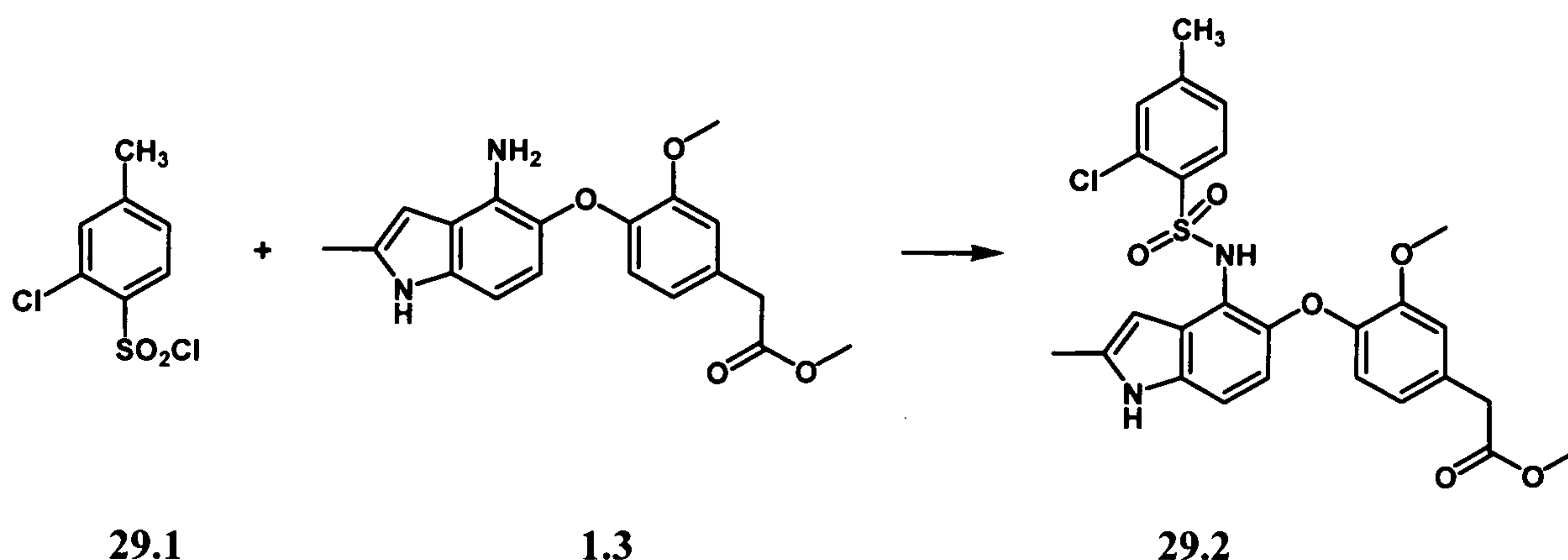
Scheme 29.2
