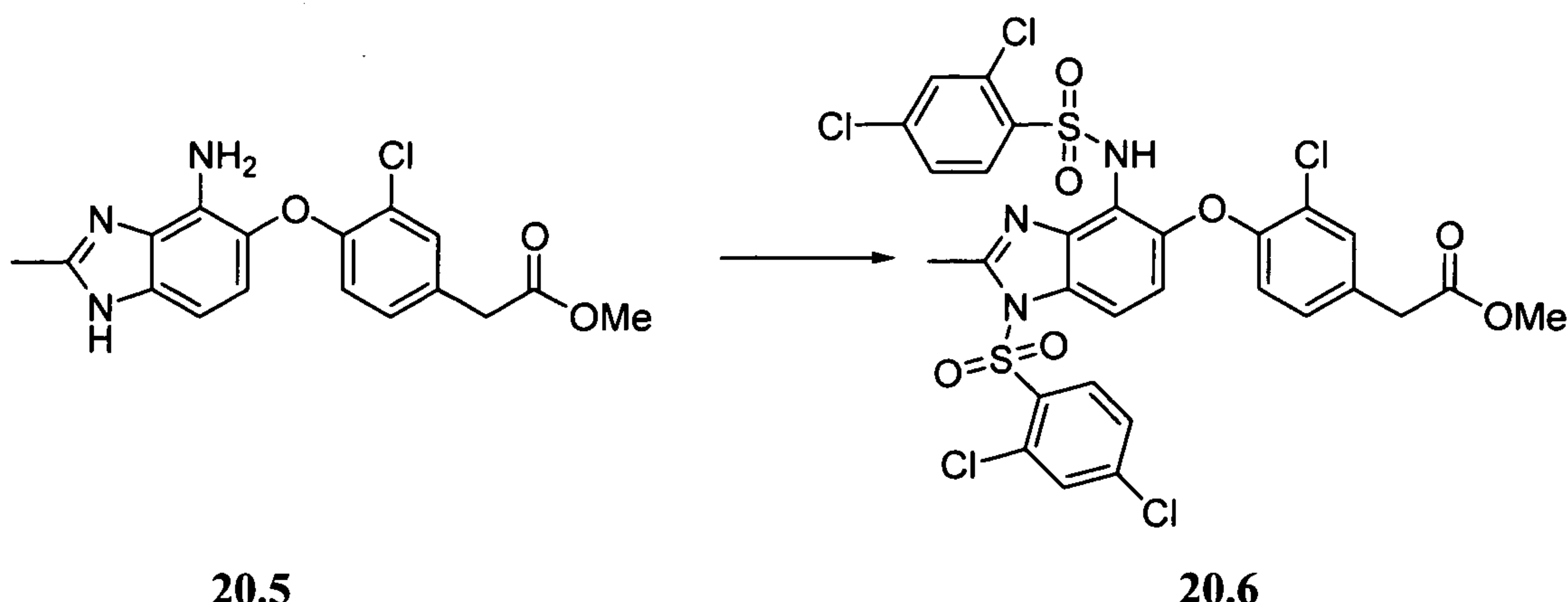
Scheme 20.6
