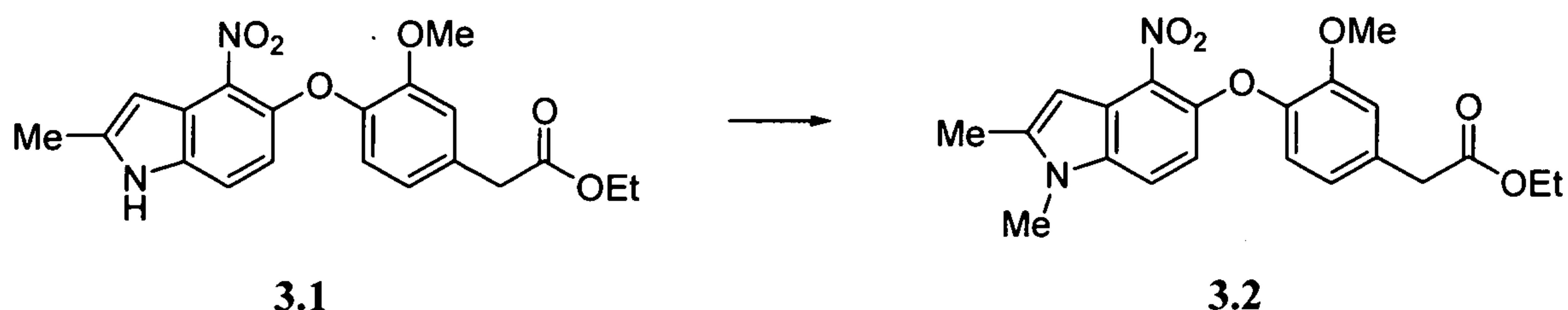
Scheme 3.2
