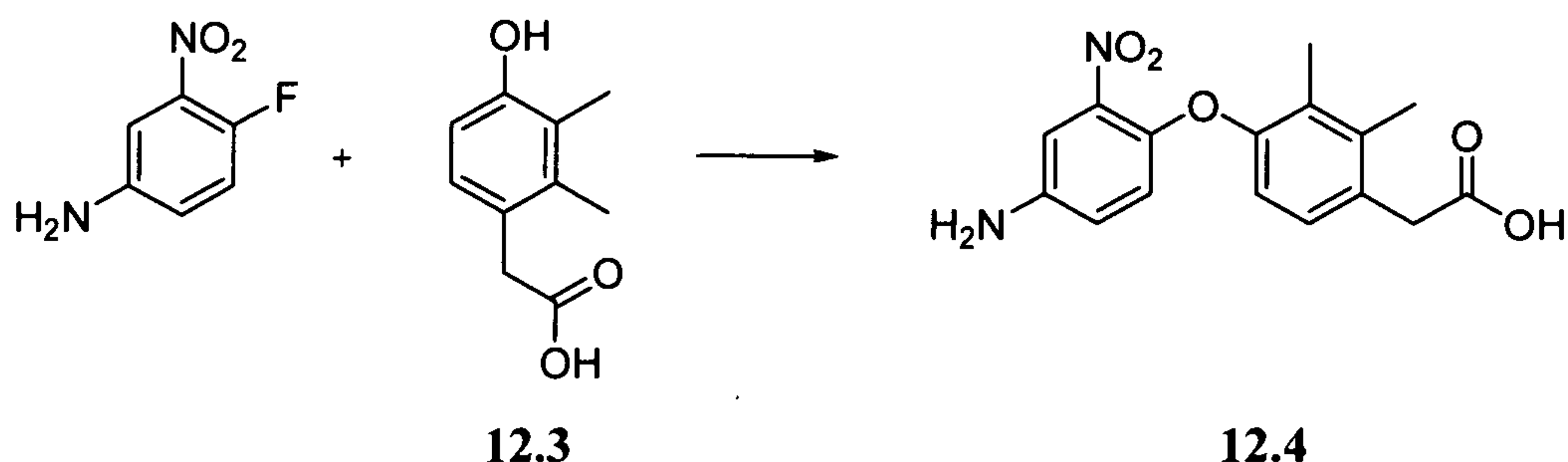
Scheme 12.4
