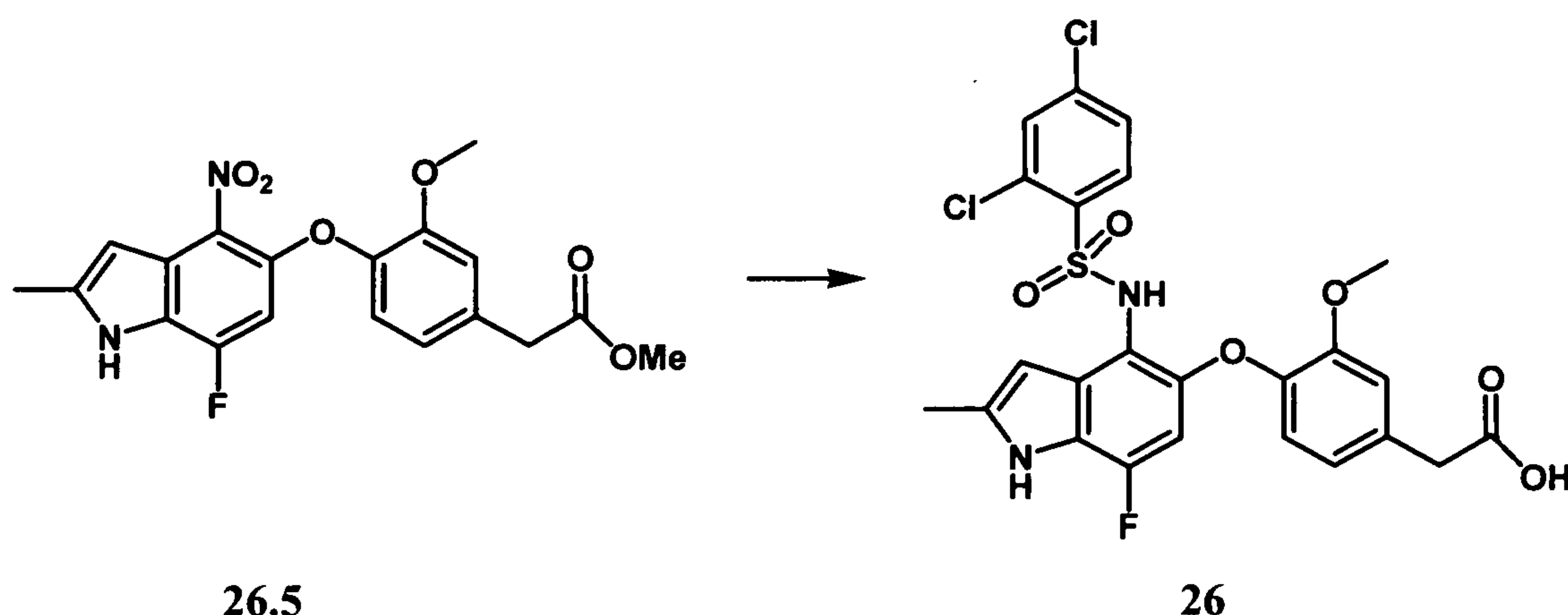
Scheme 26.4
