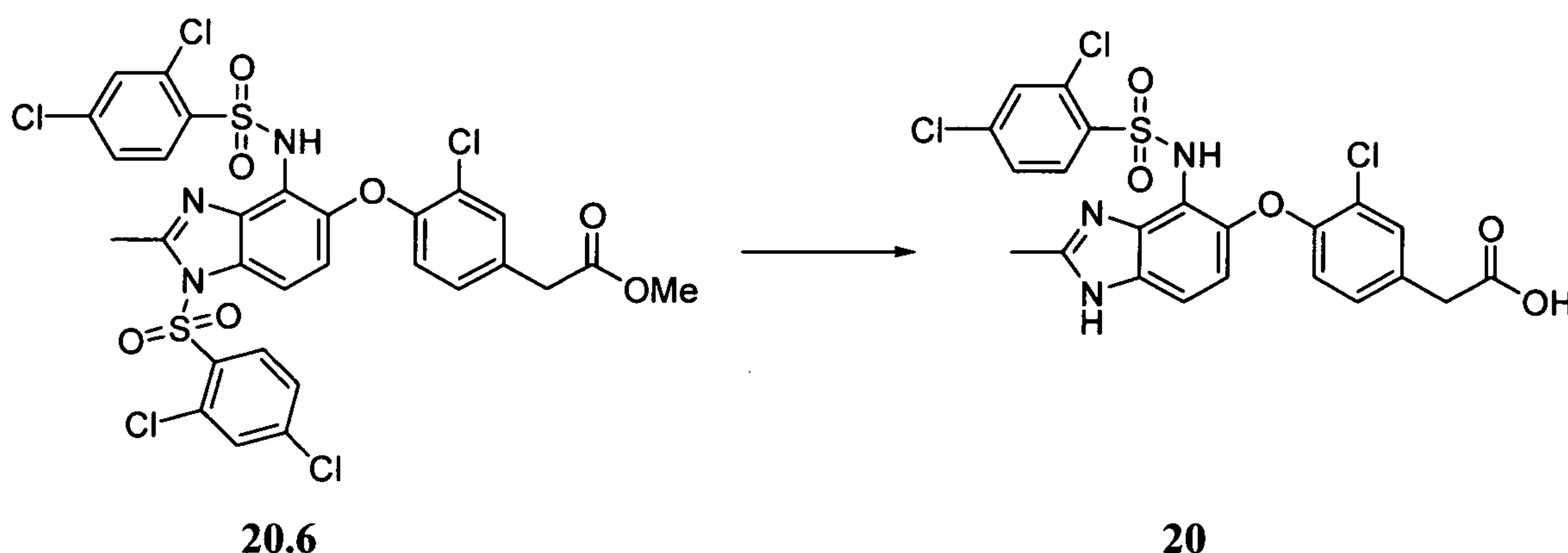
Scheme 20.7
