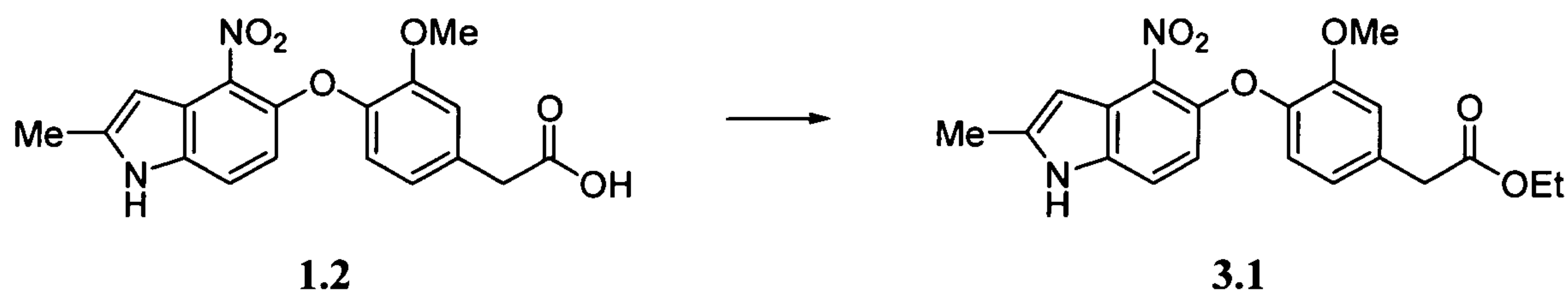
Scheme 3.1
