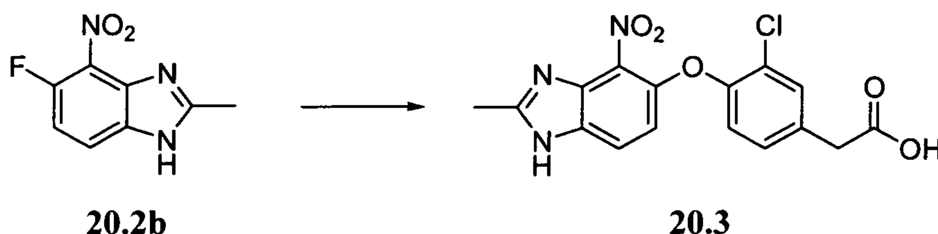
Scheme 20.3
