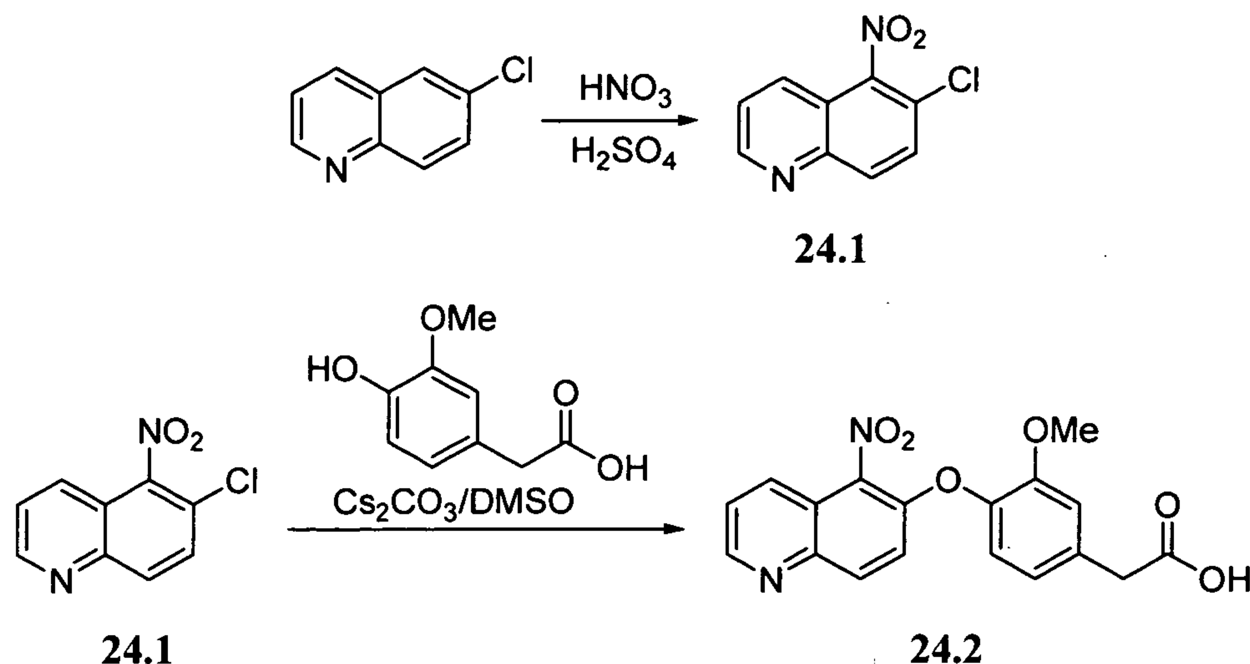
Scheme 24.1
