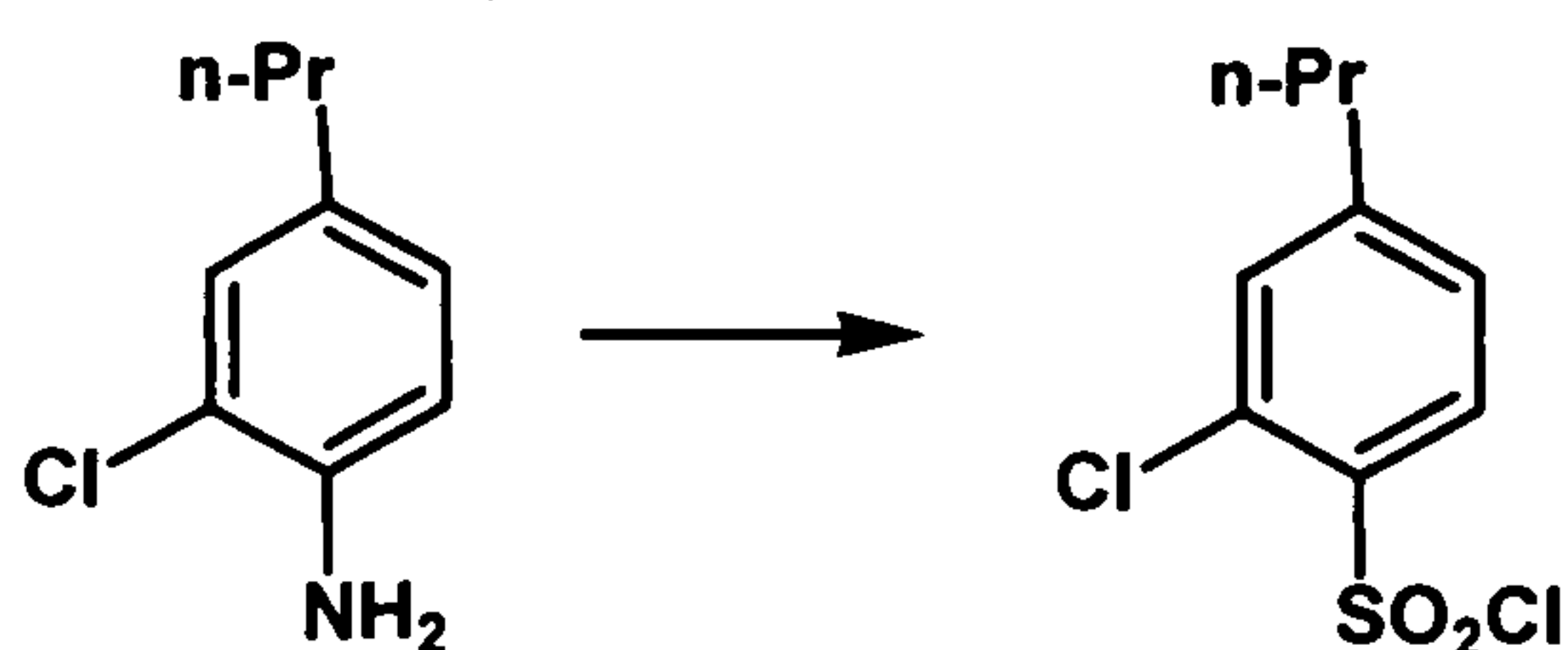
Scheme 10.2
