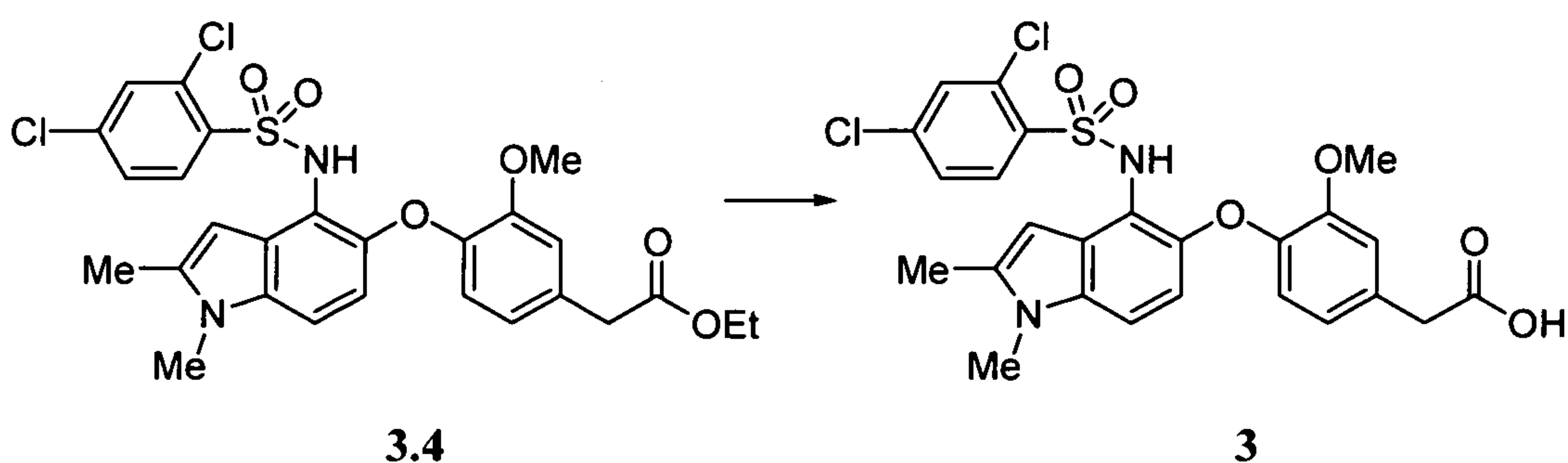
Scheme 3.5
