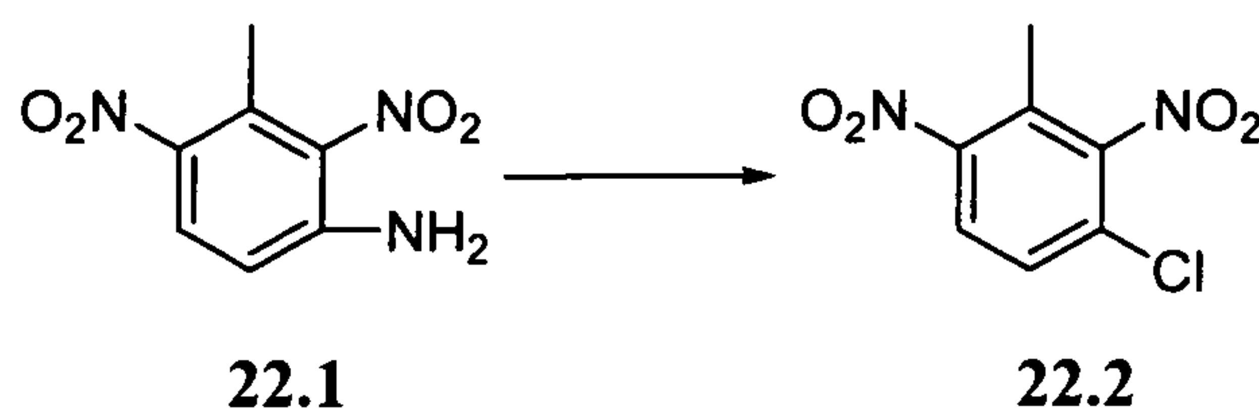
Scheme 22.2
