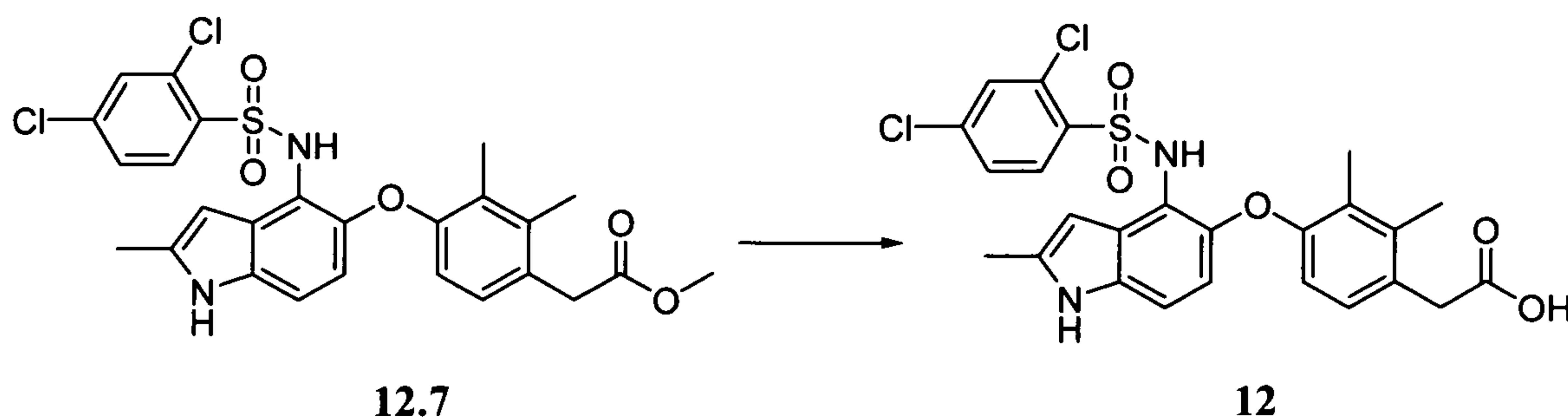
Scheme 12.8
