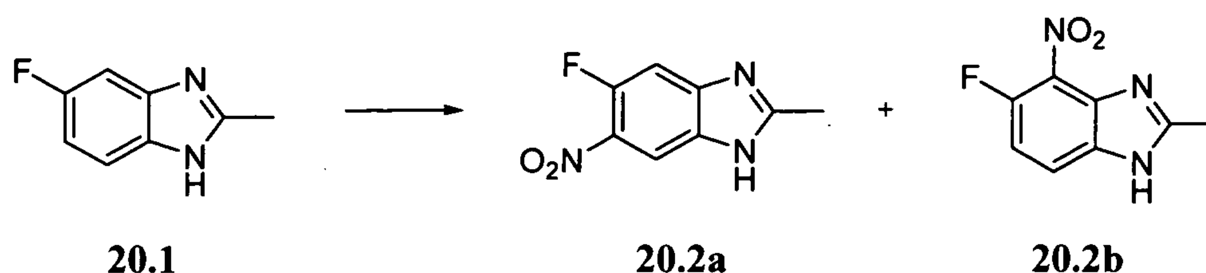
Scheme 20.2
