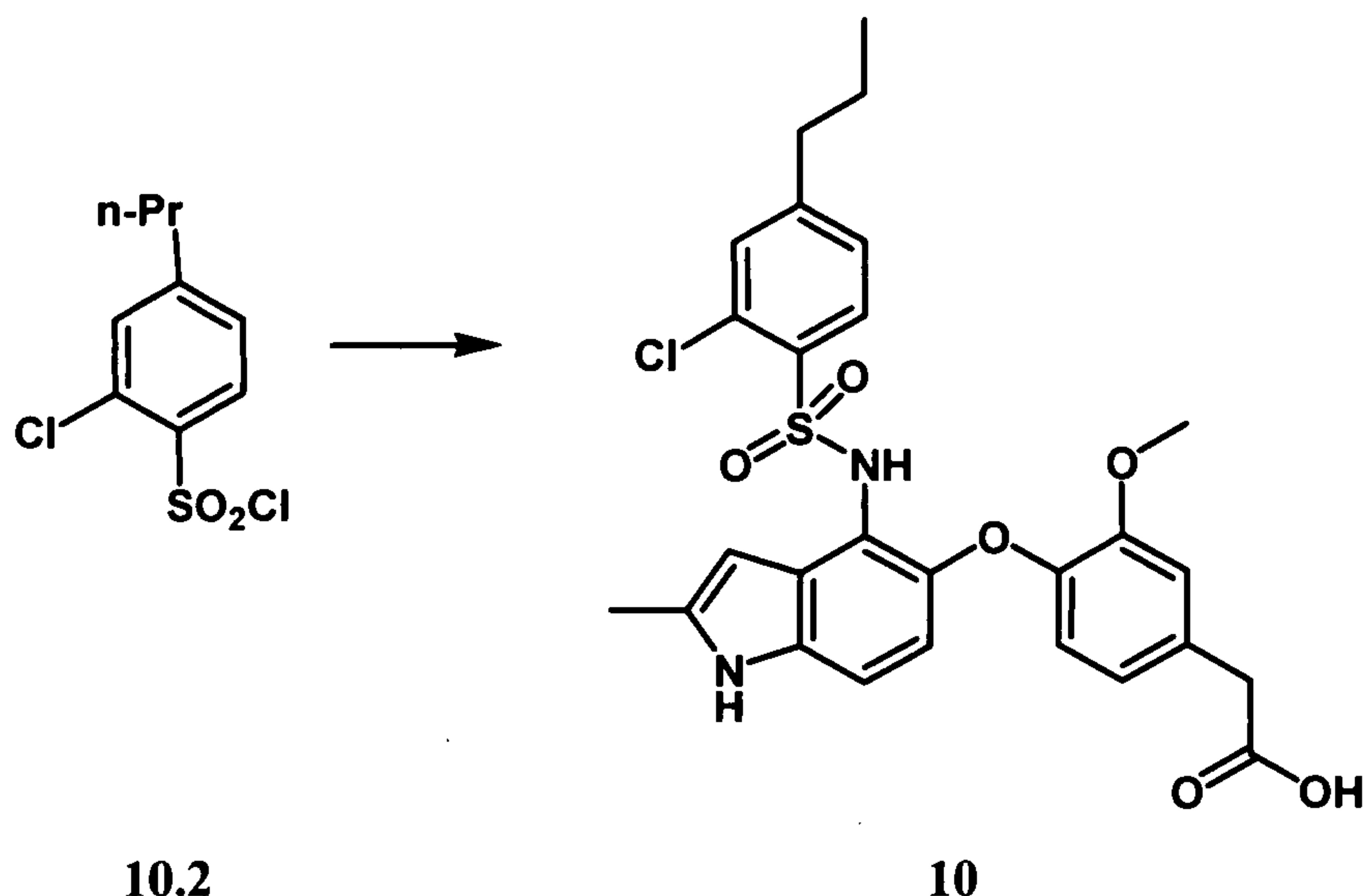
Scheme 10.3
