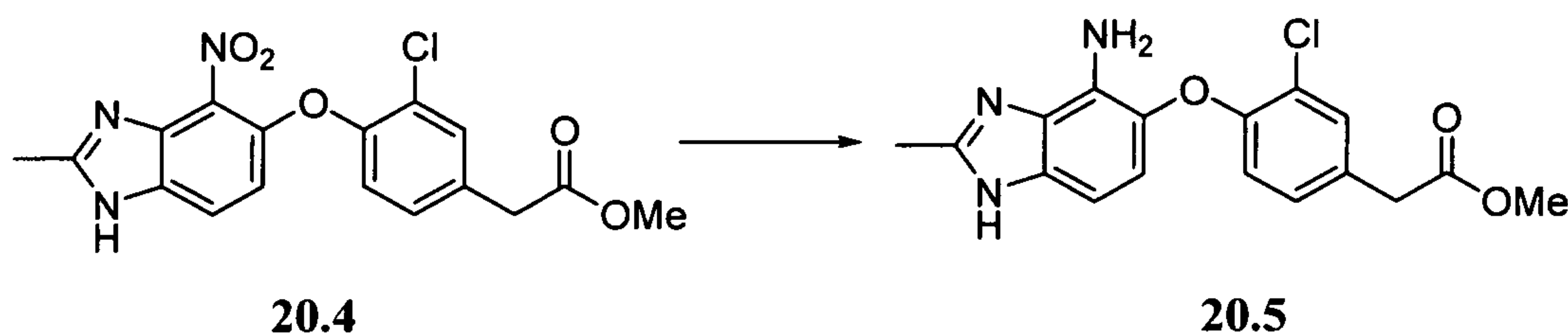
Scheme 20.5
