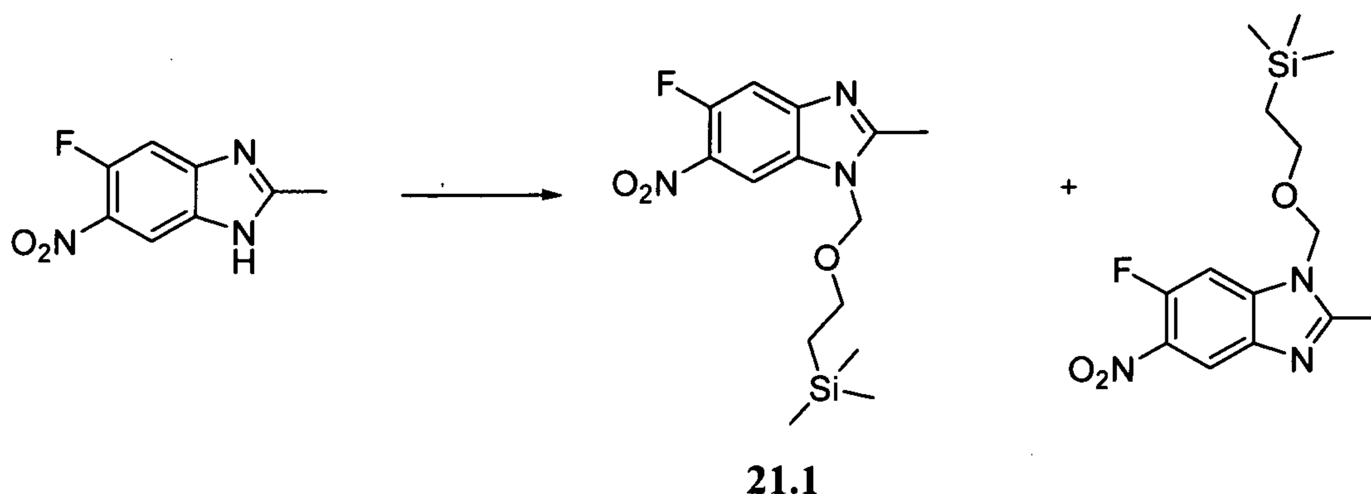
Scheme 21.1
