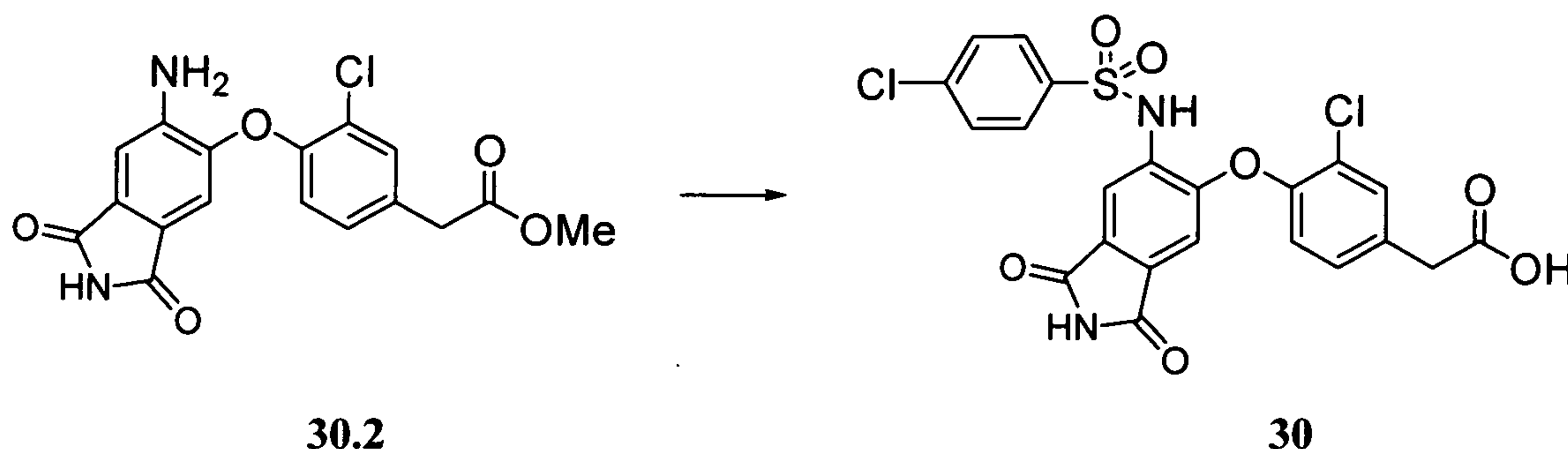
Scheme 30.3
