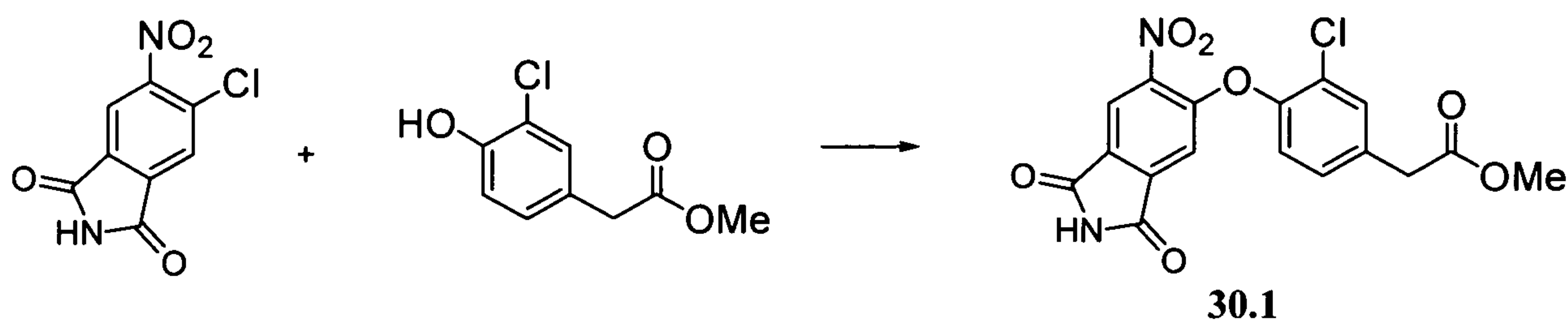
Scheme 30.1
