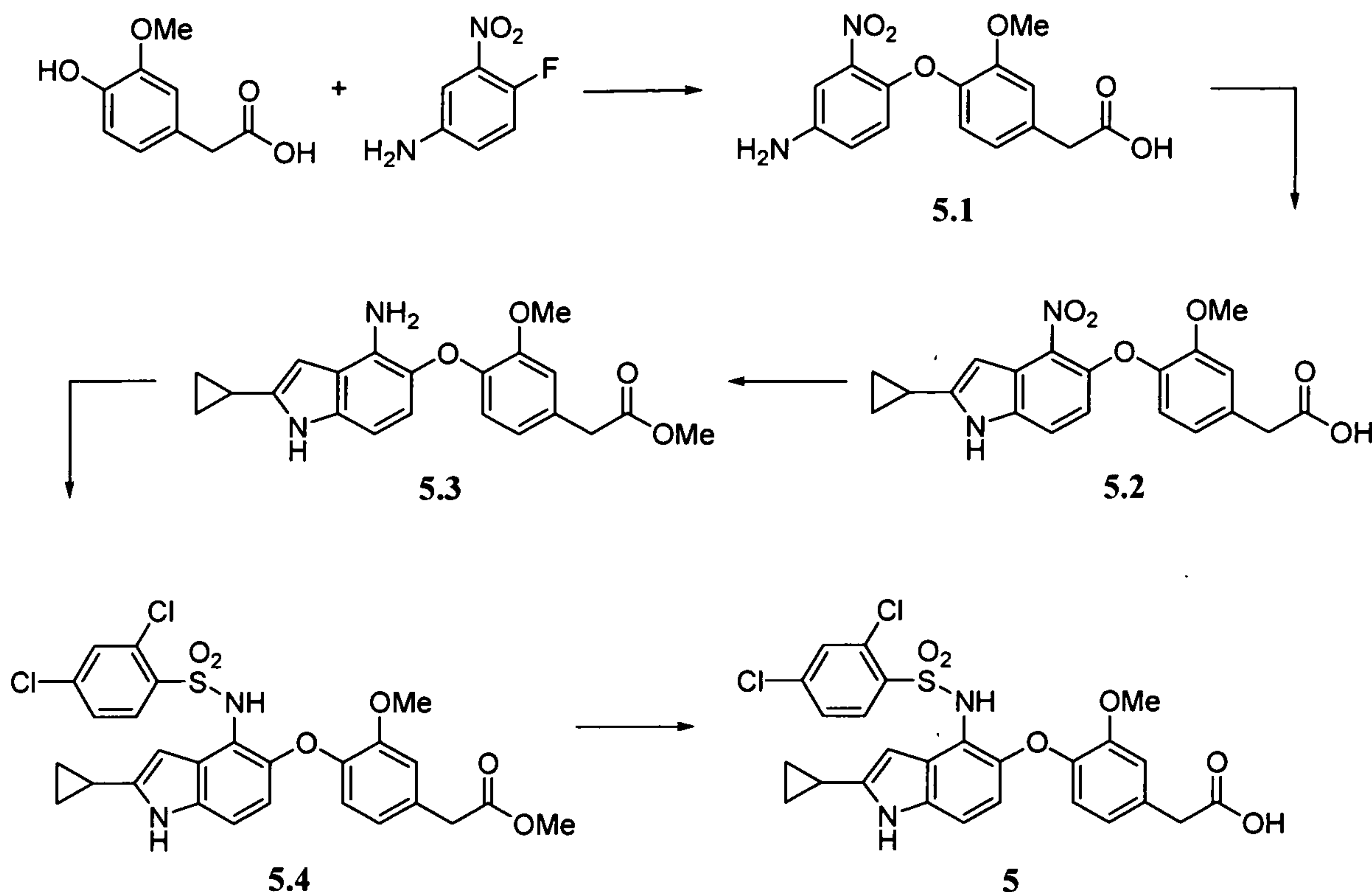
Scheme 5
