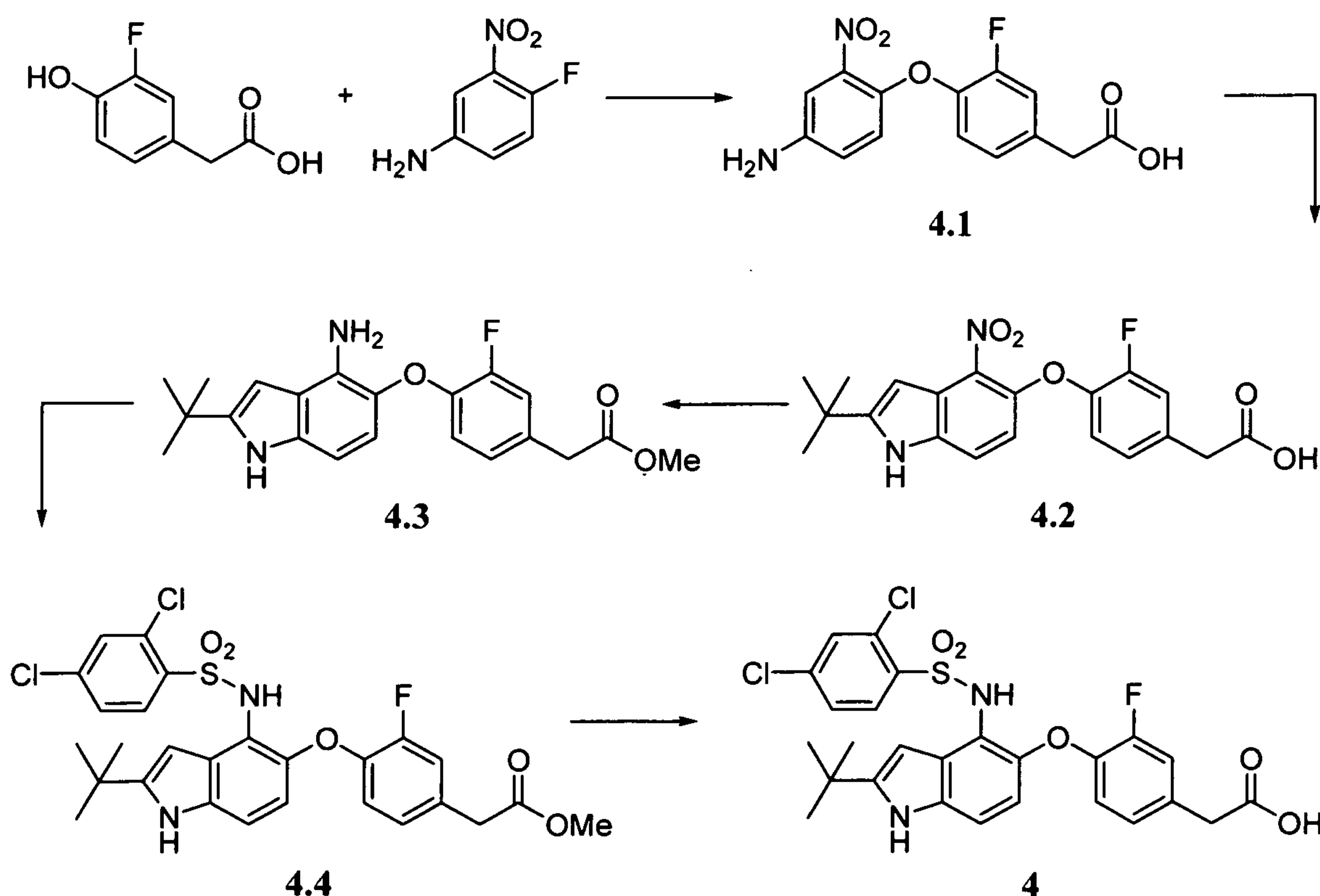
Scheme 4
