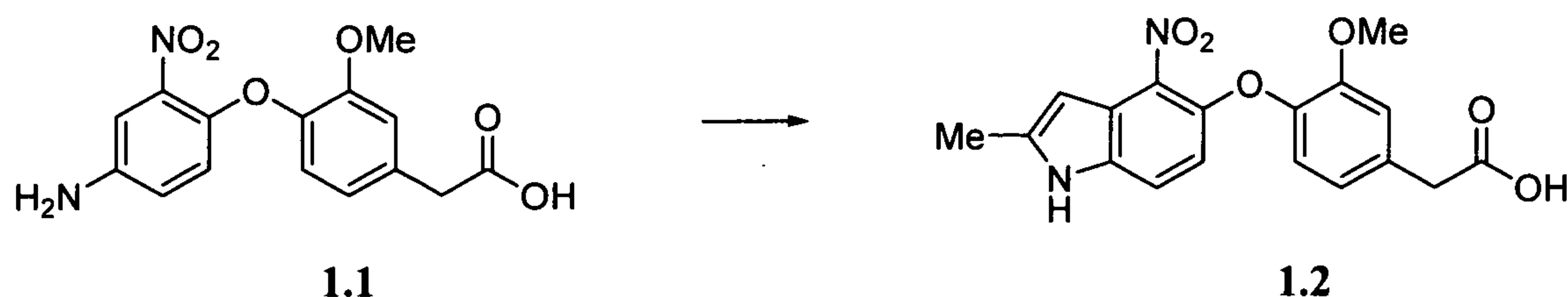
Scheme 1.2
