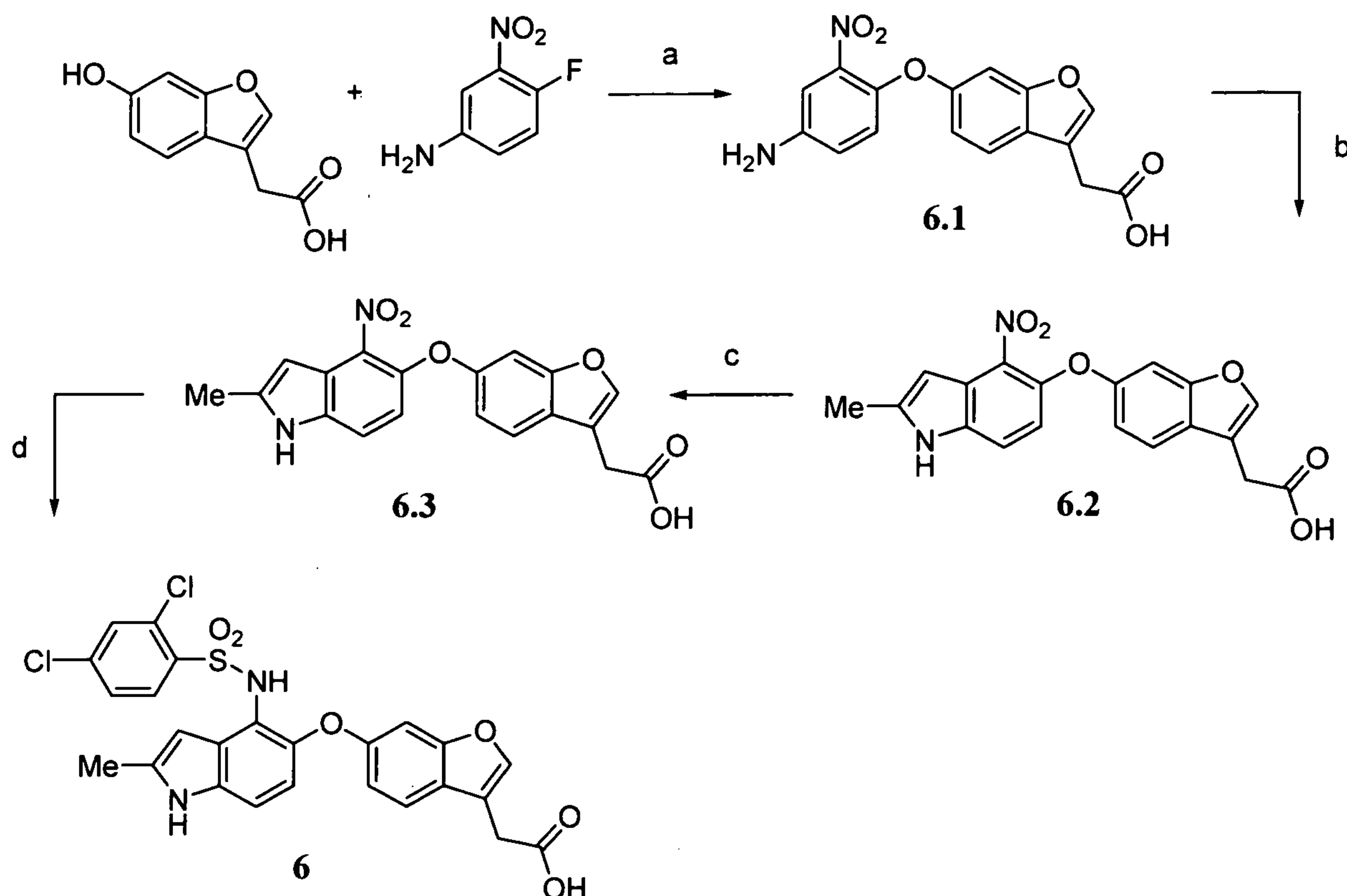
Scheme 6
