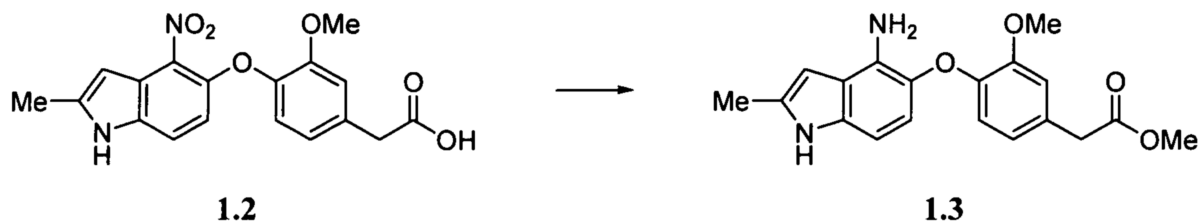
Scheme 1.3
