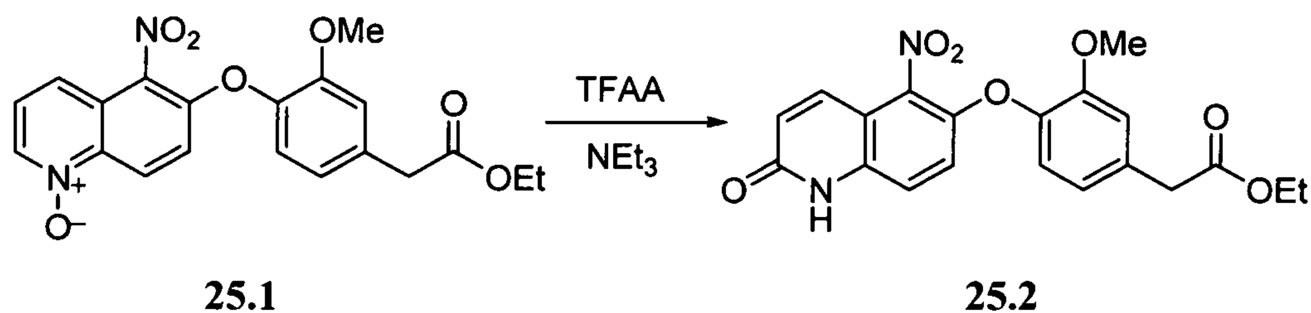
Scheme 25.2
