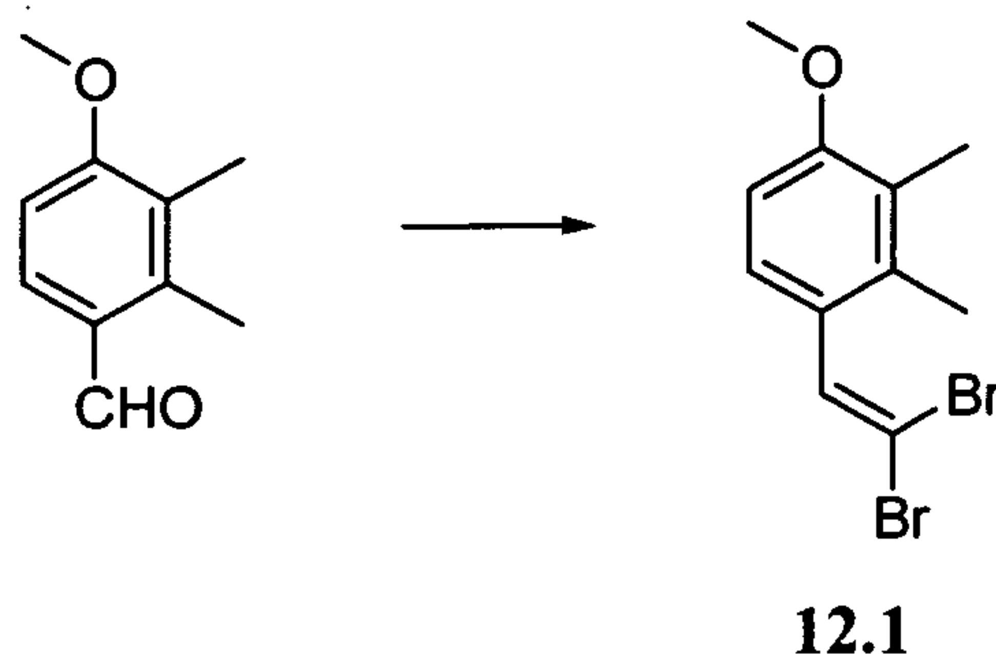
Scheme 12.1
