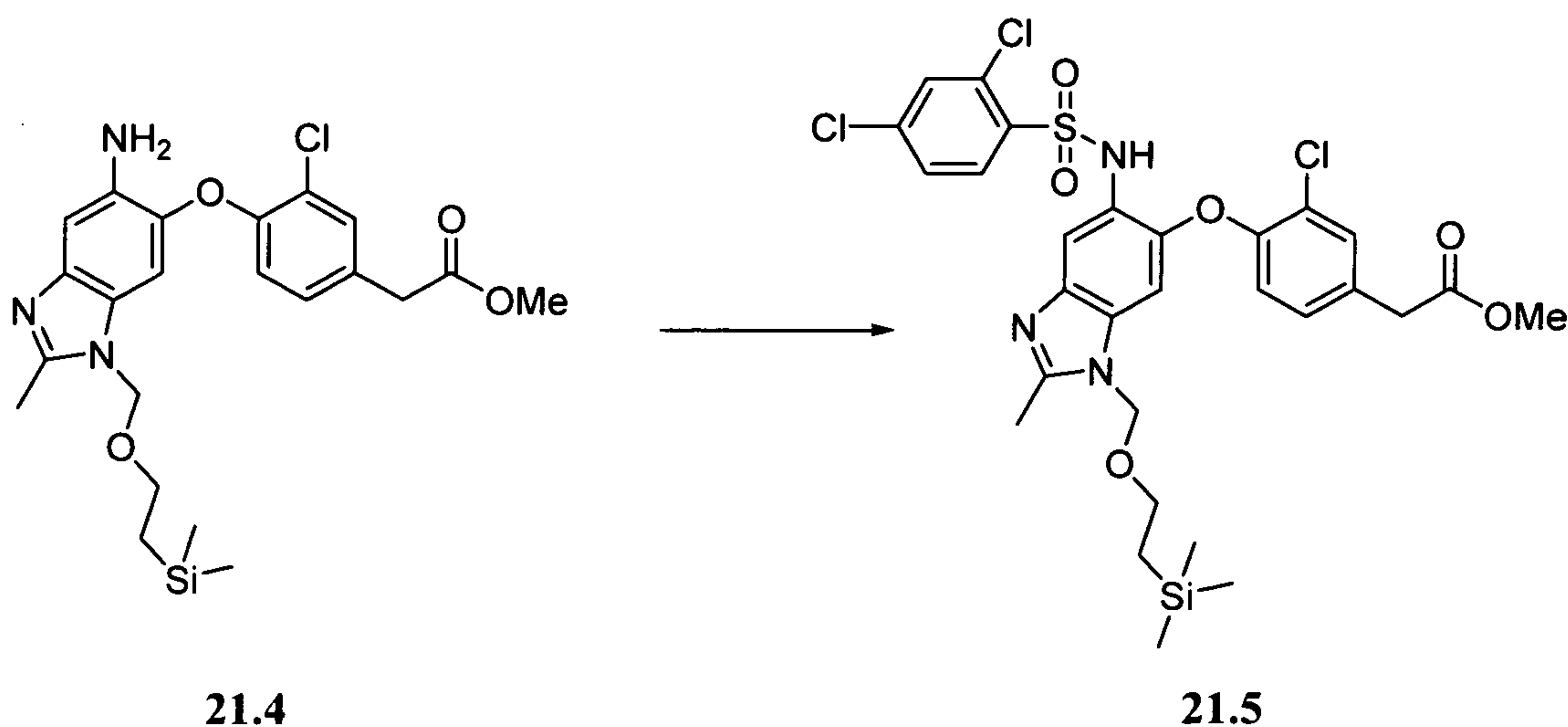
Scheme 21.5
