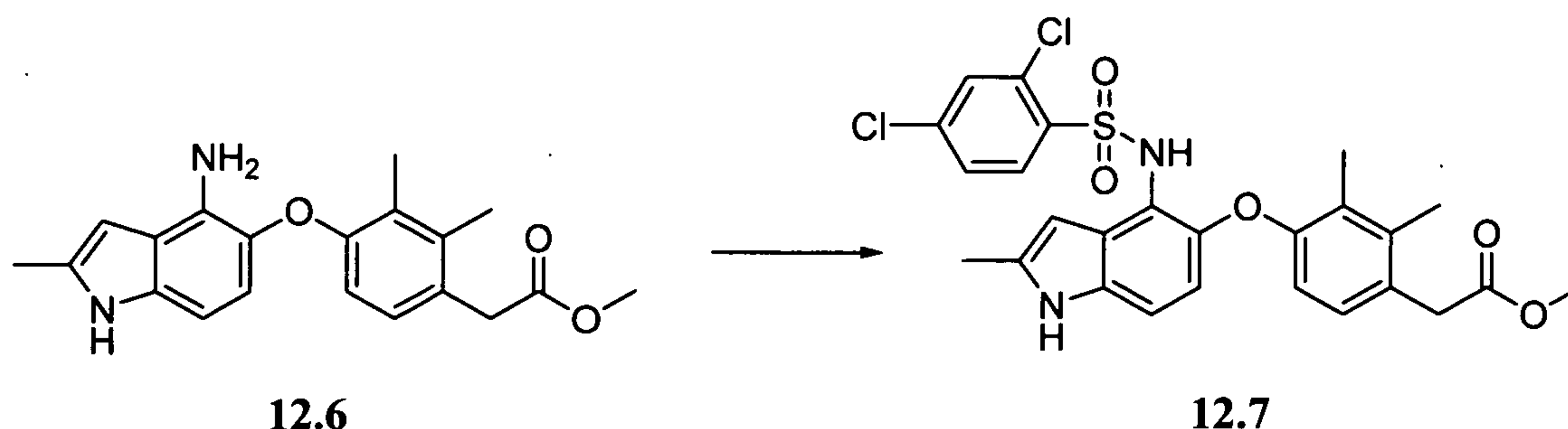
Scheme 12.7
