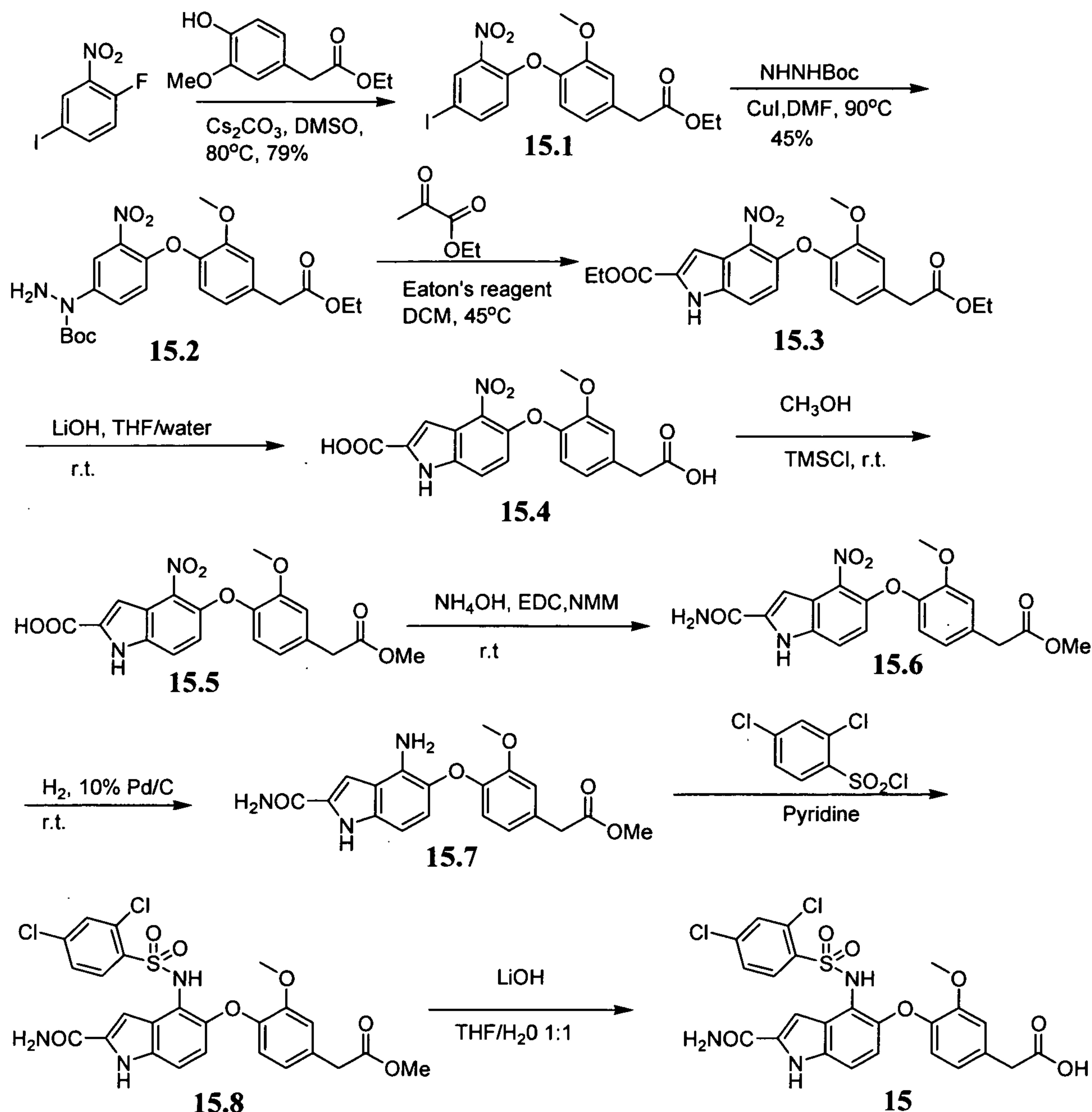
Scheme 15
