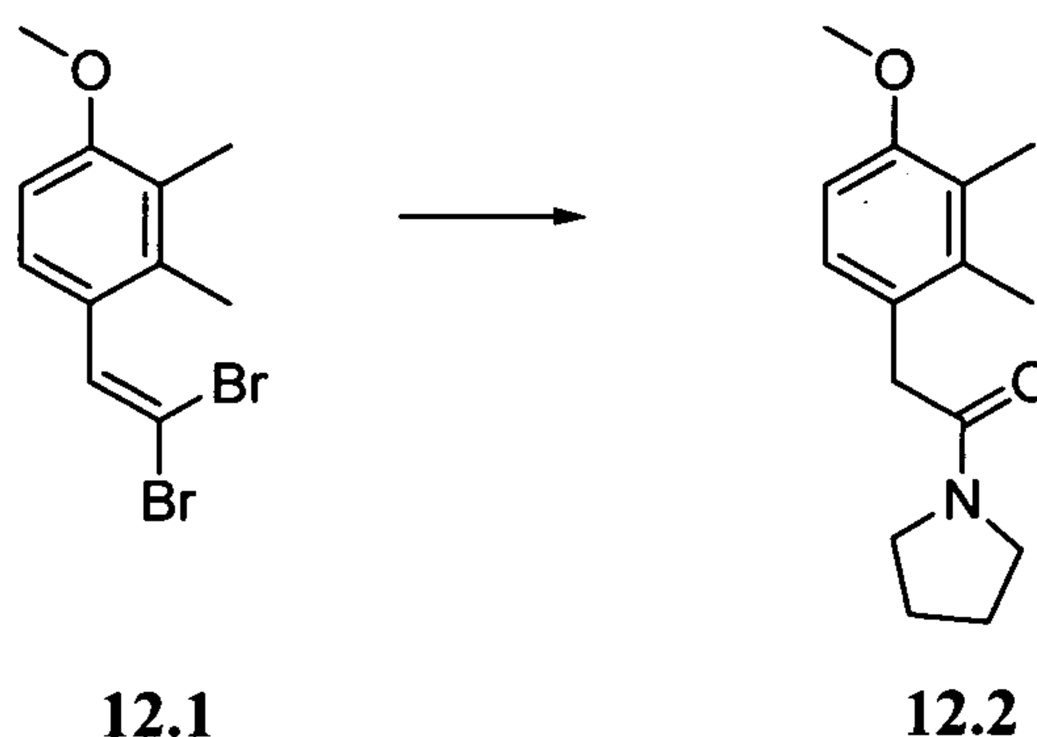
Scheme 12.2
