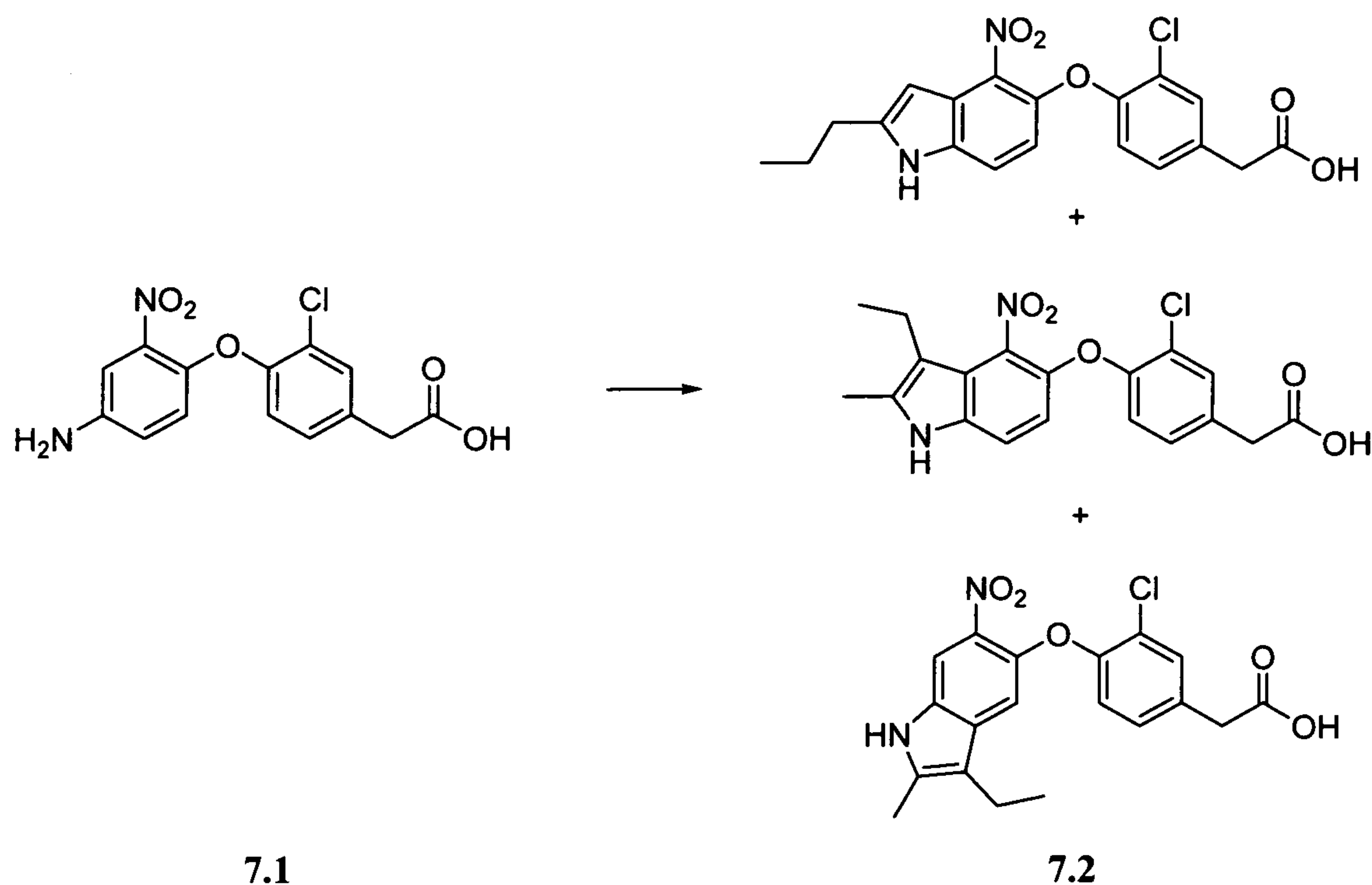
Scheme 7.2
