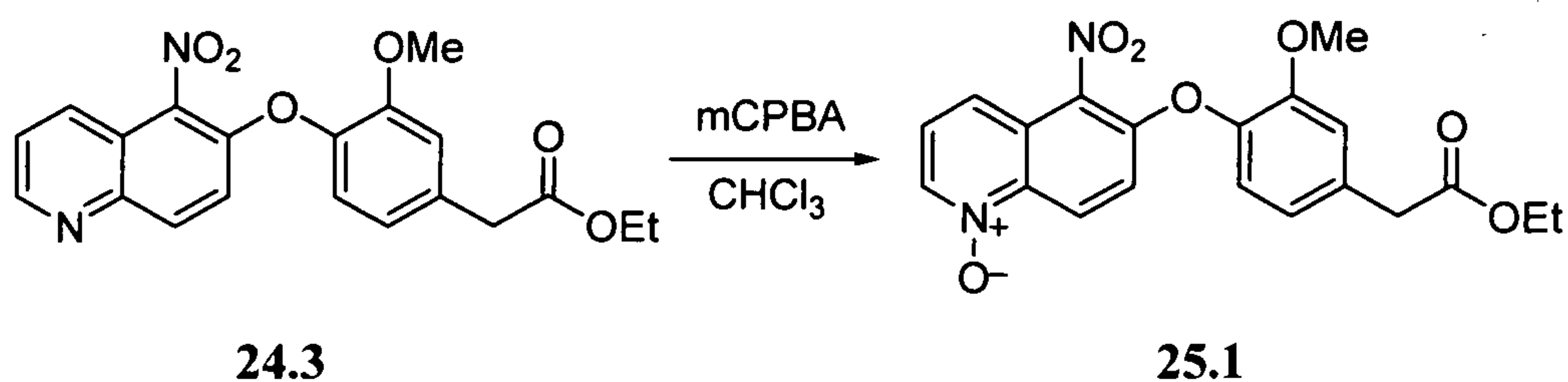
Scheme 25.1
