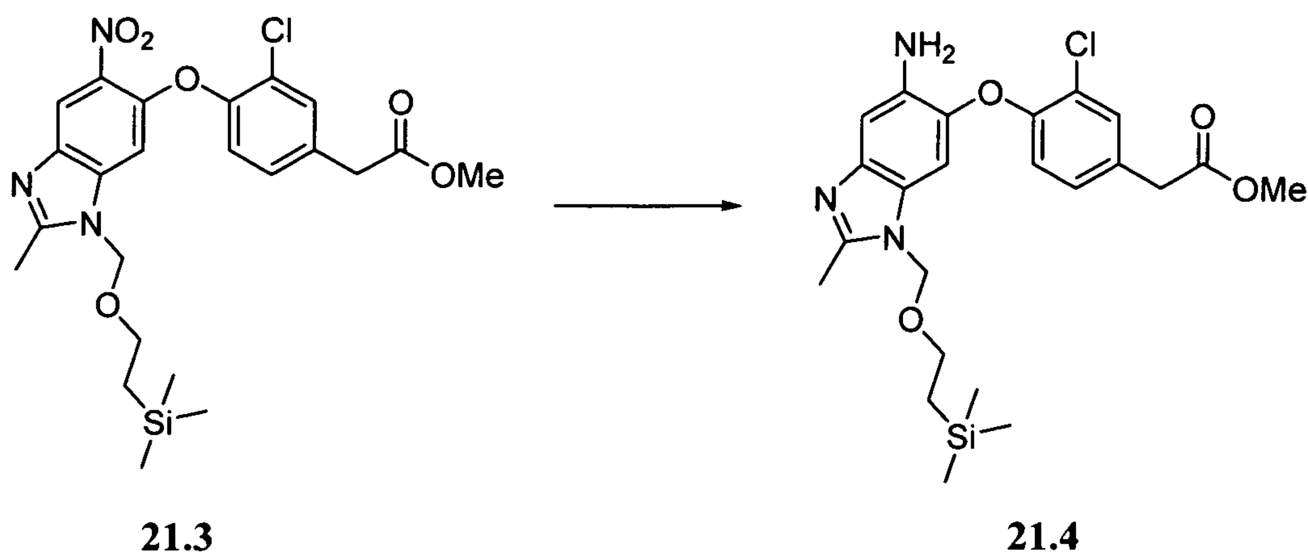
Scheme 21.4
