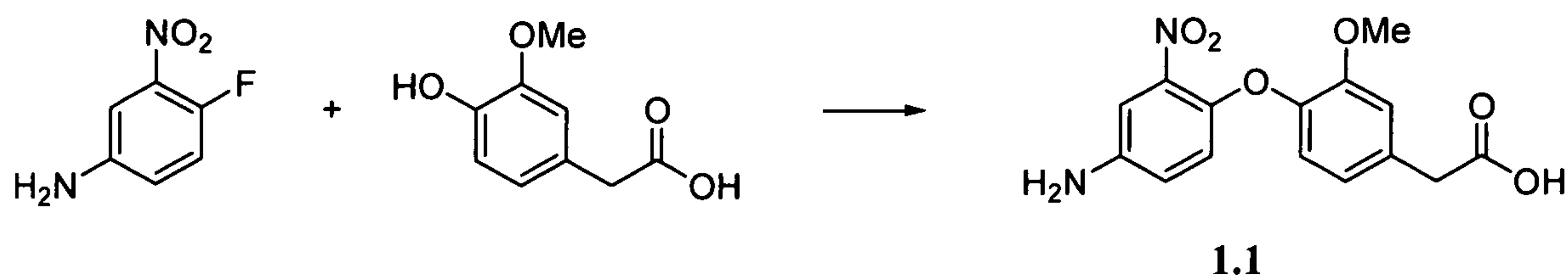
Scheme 1.1
