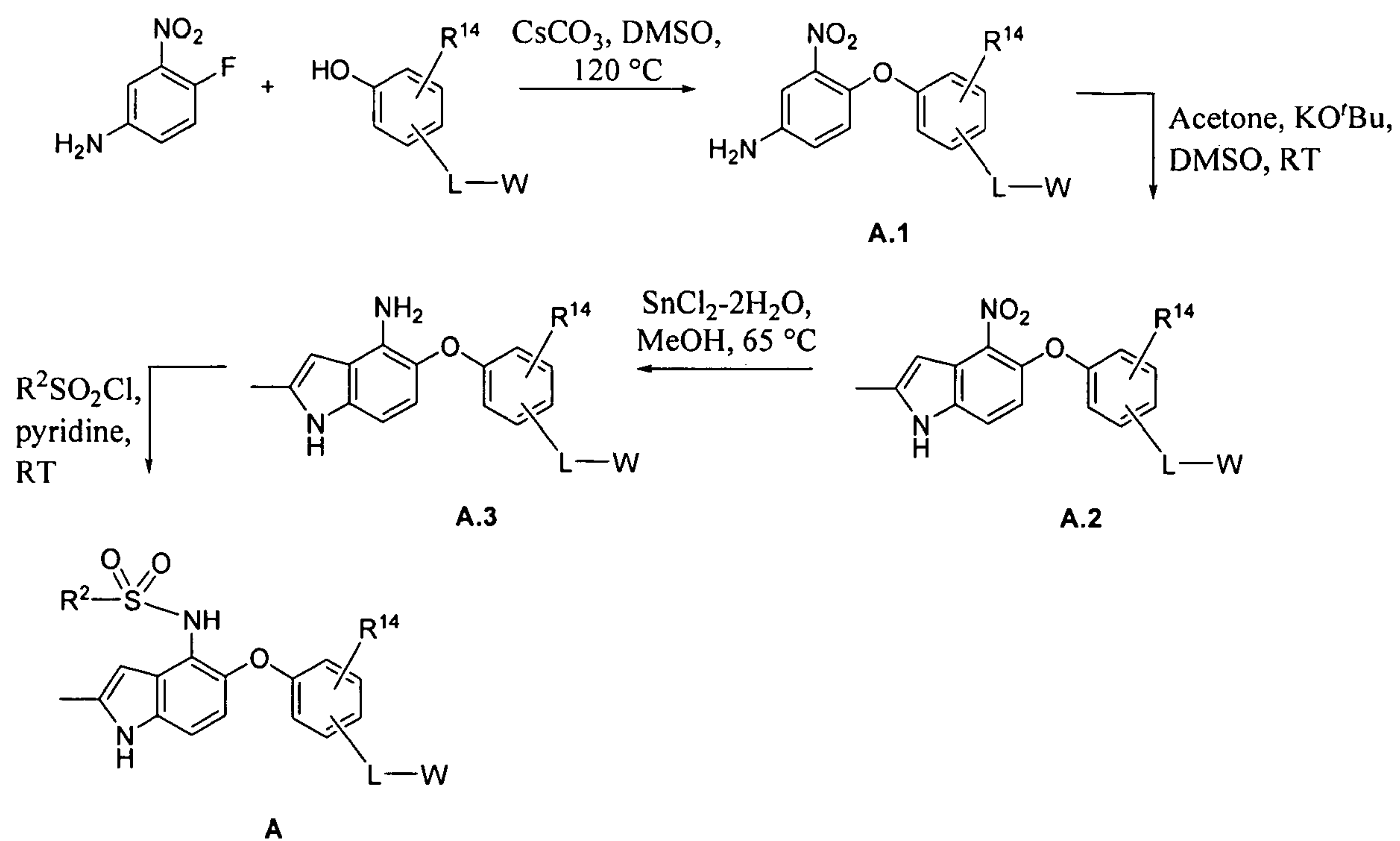
Scheme A
