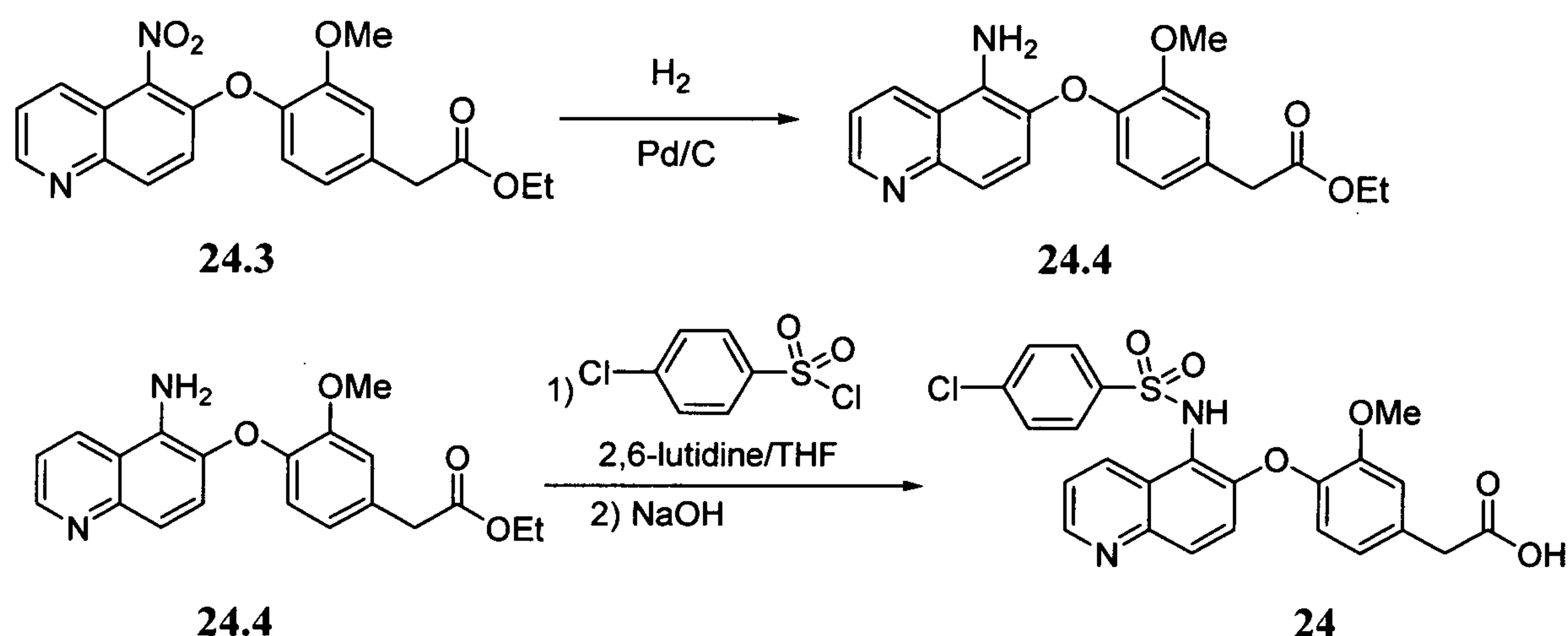
Scheme 24.3
