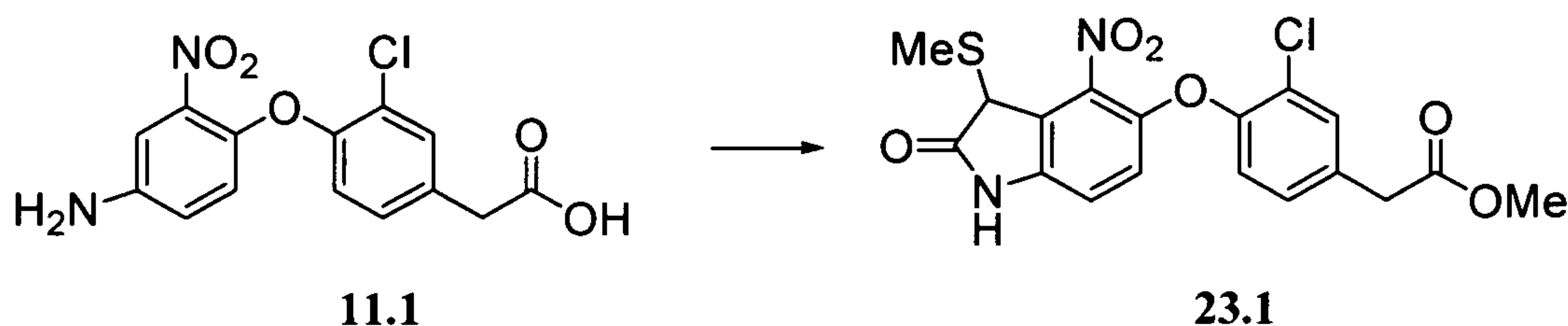
Scheme 23.1
