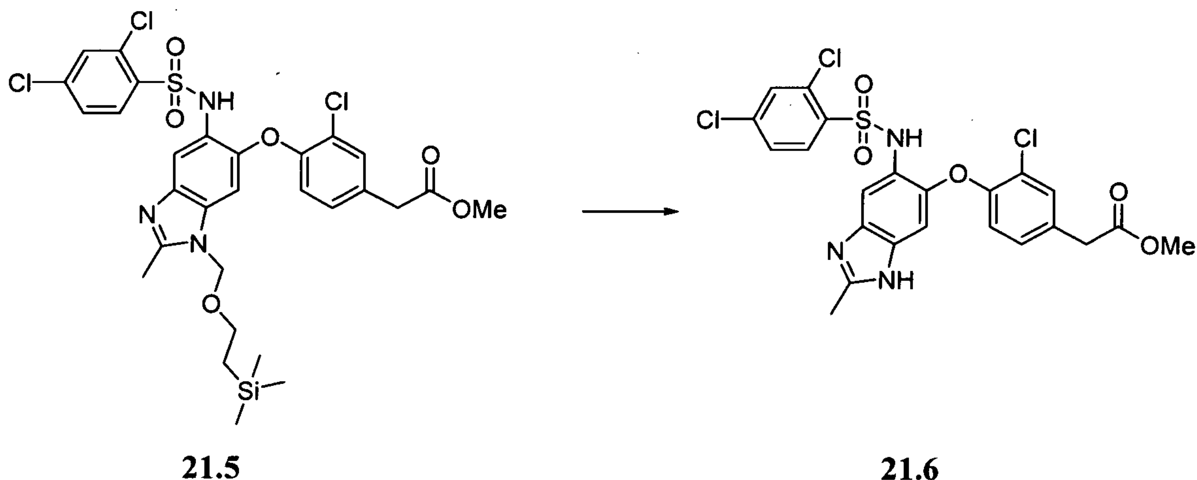
Scheme 21.6
