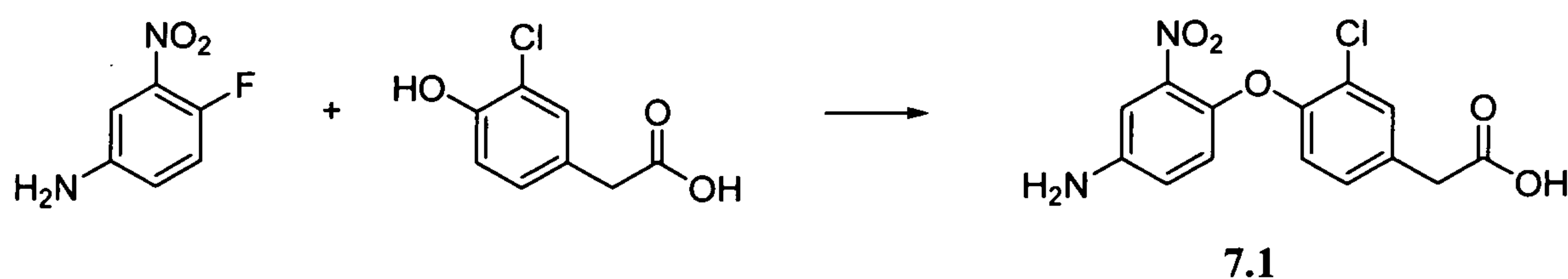
Scheme 7.1
