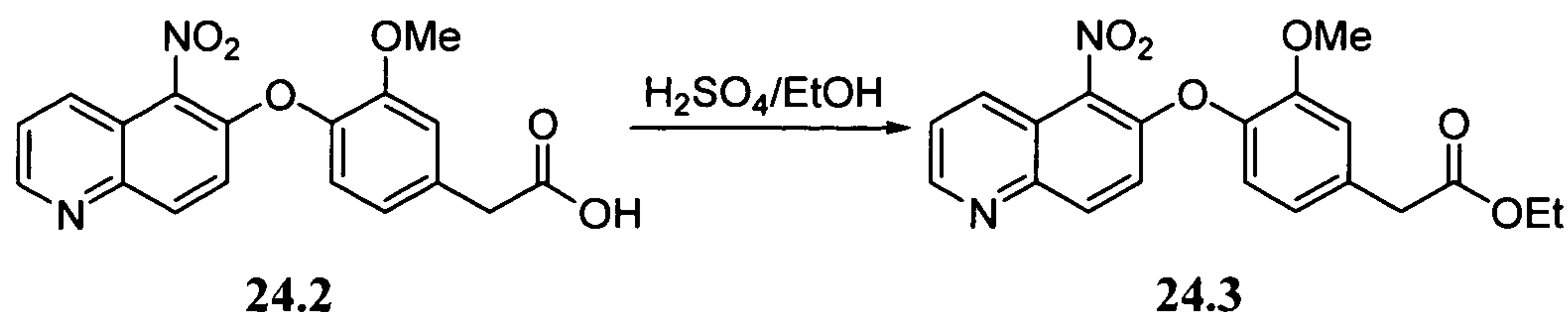
Scheme 24.2
