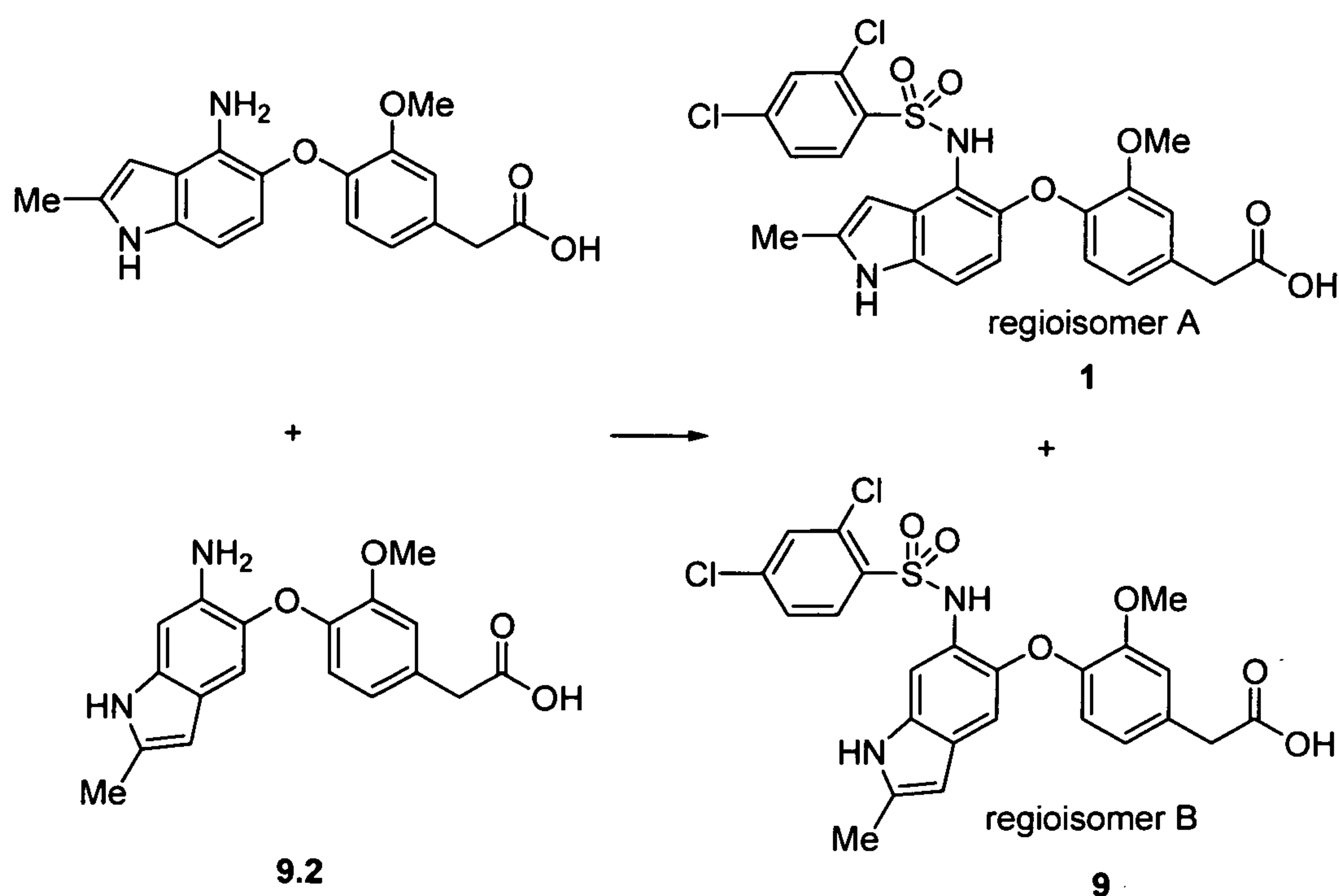
Scheme 9.2
