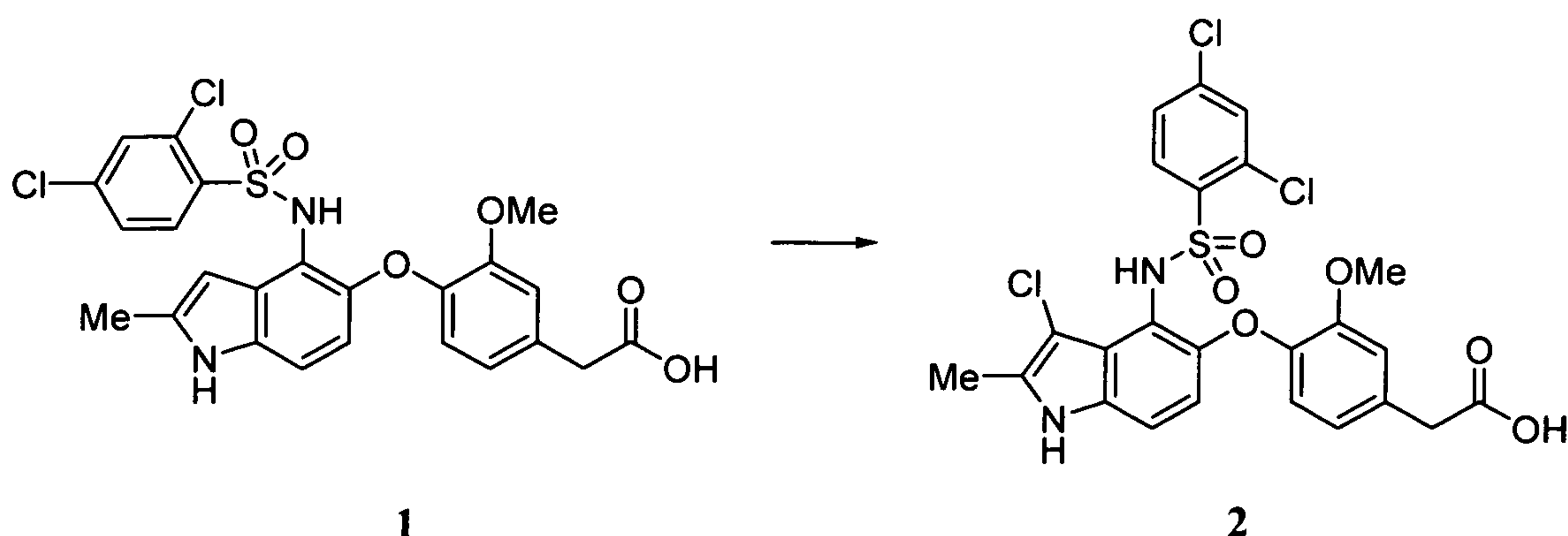
Scheme 2
