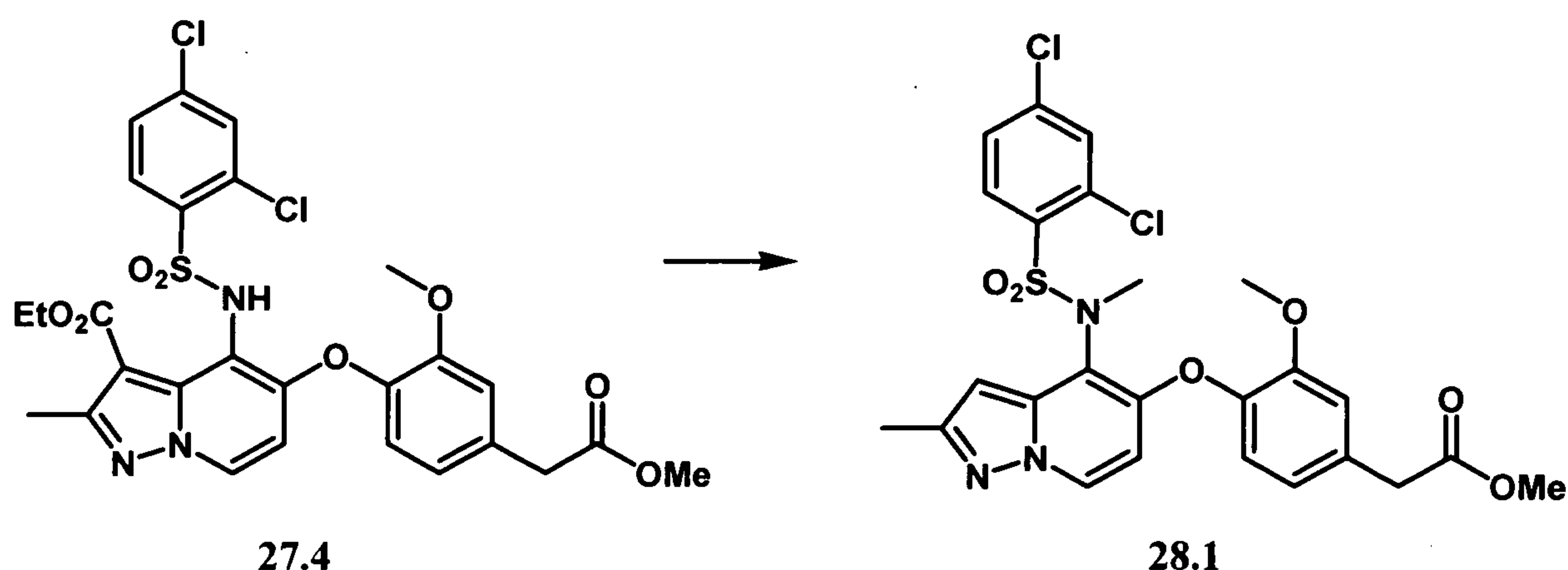
Scheme 28.1
