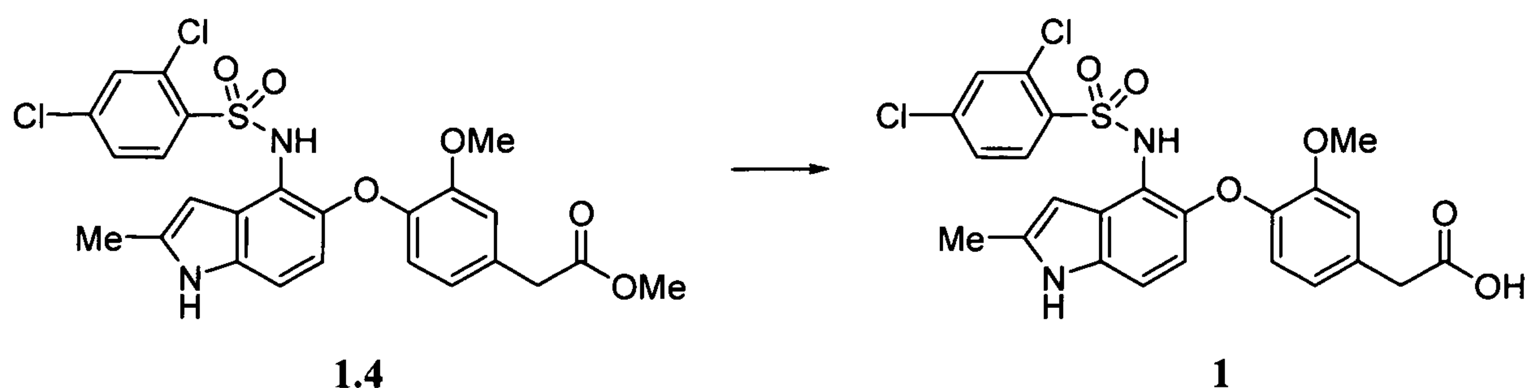
Scheme 1.5
