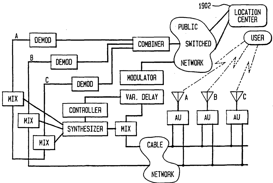
FIG. 19 LOCATION CENTER EXTERNAL TO COMMUNICAITON SYSTEM
