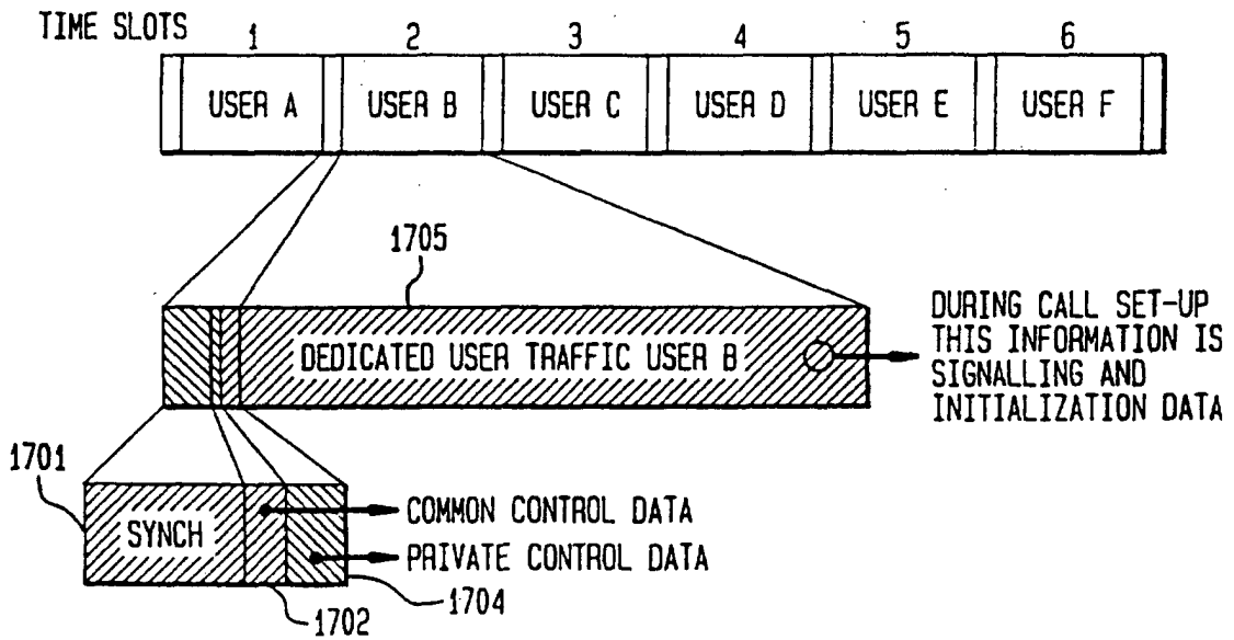
FIG. 17 SYNCH AND CONTROL CHANNEL STRUCTURE
