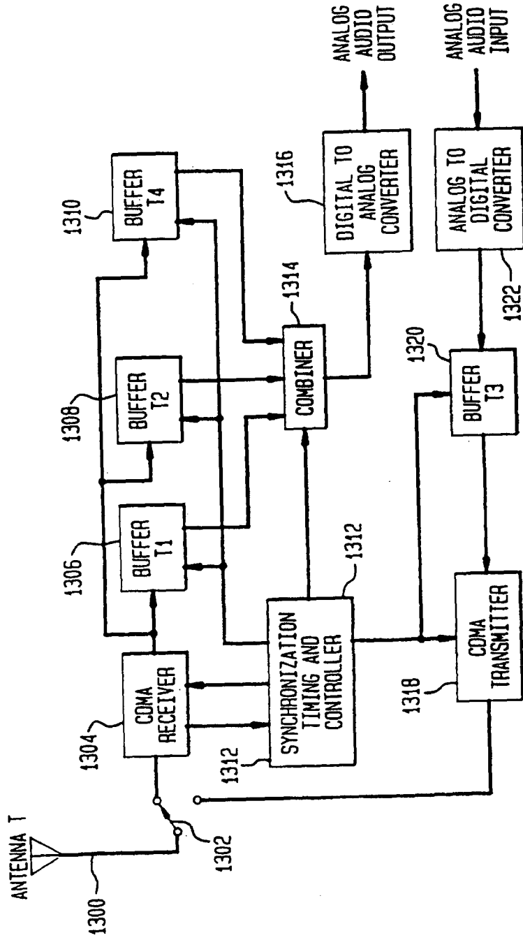
FIG. 13 SUBSCRIBER STATION
