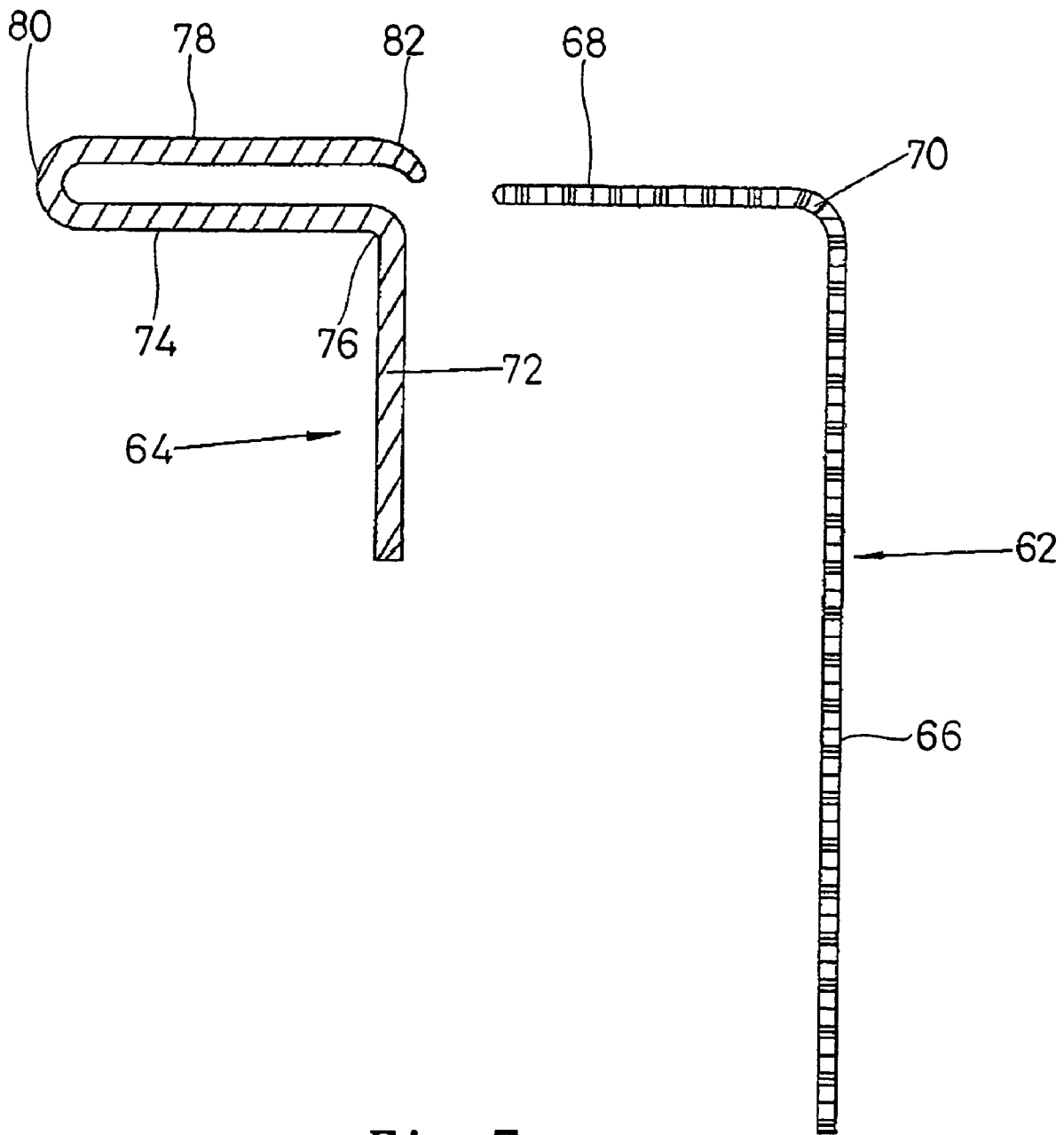
Fig. 7 PRIOR ART
