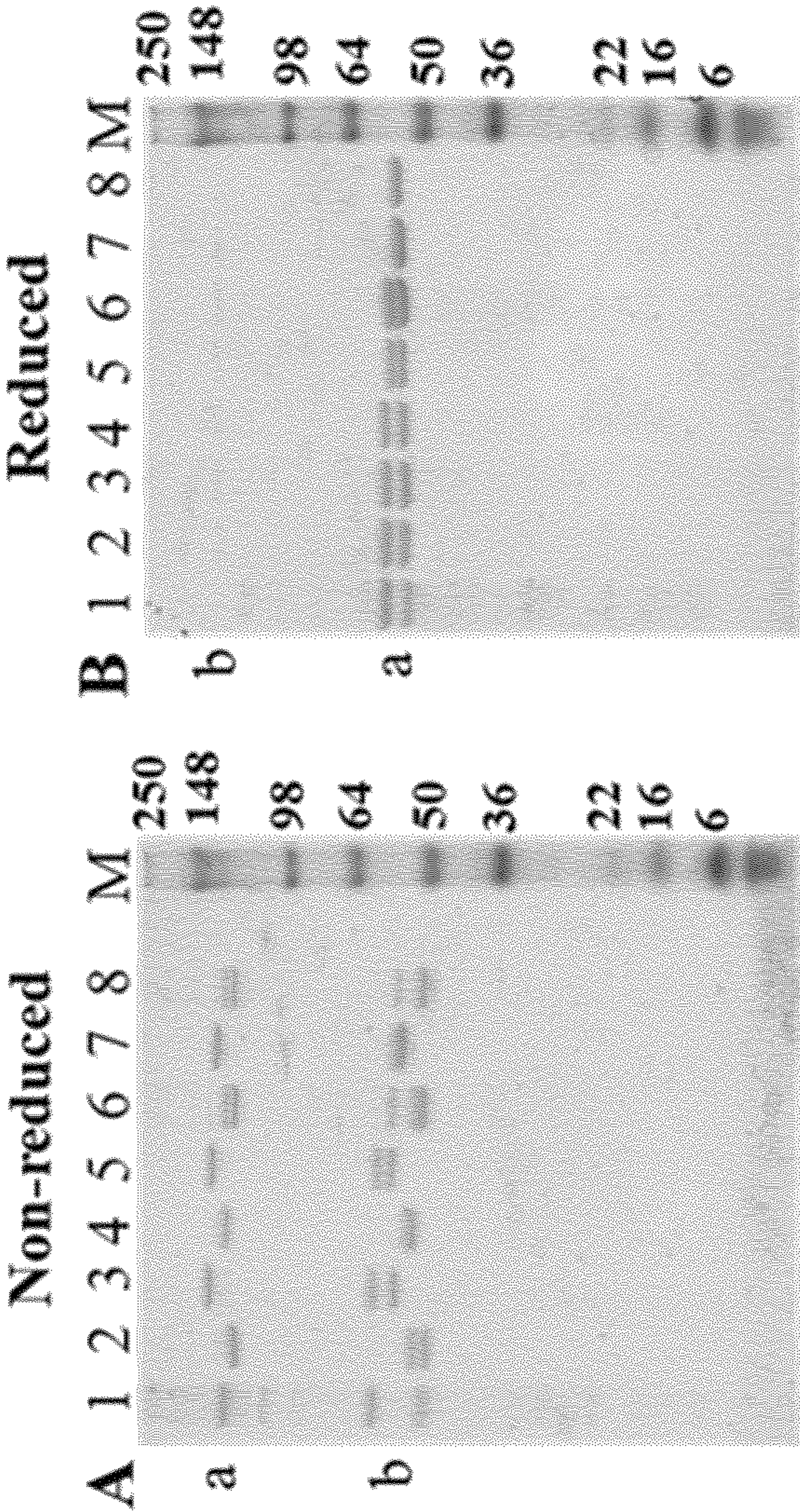
Figure 10 SDS-PAGE analysis of Protein-G purified, EXPiHEK expressed Fab-2xscFv and Fab-2xdsscFv formats
