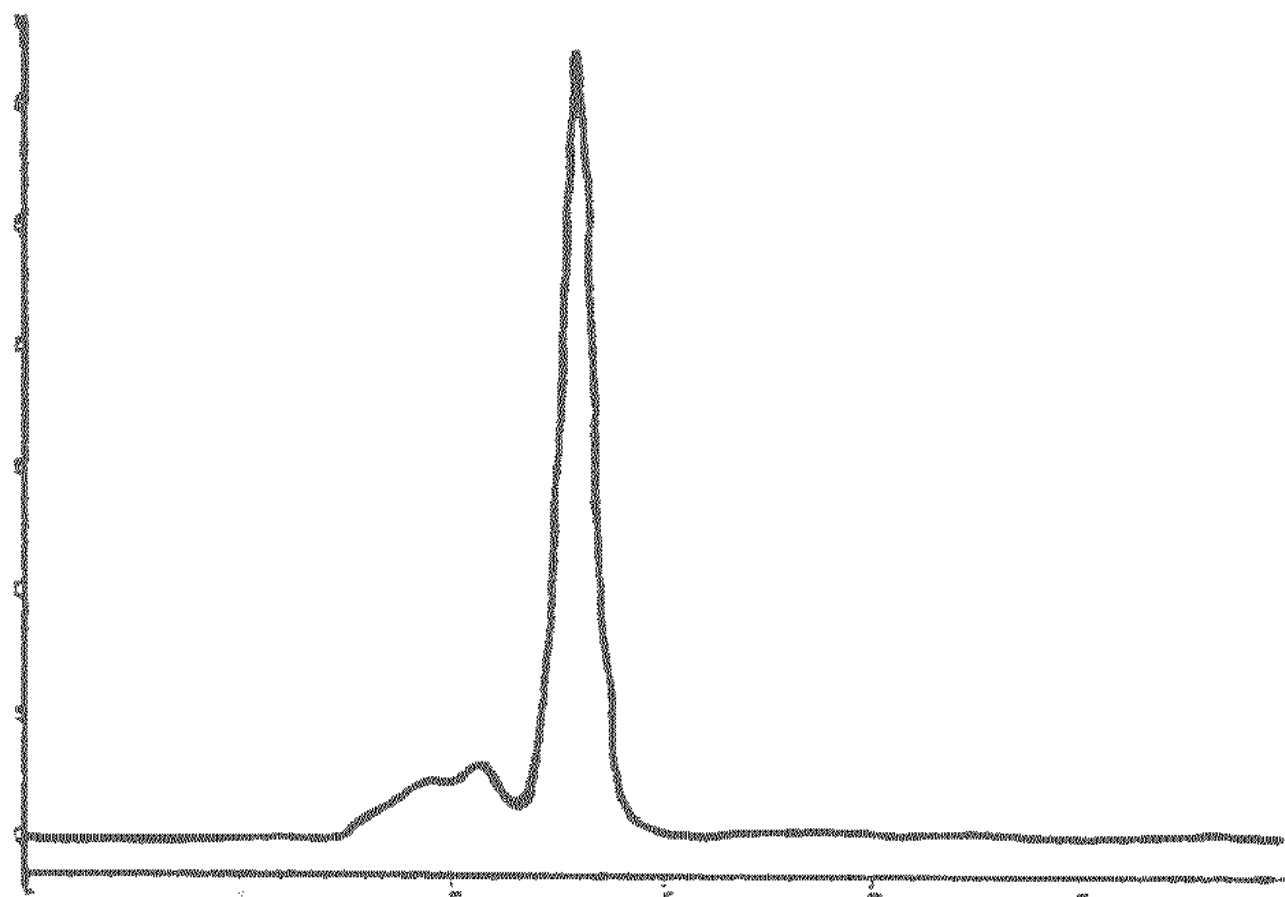
Figure 5: S200 SE HPLC analysis of purified, HEK293-expressed Fab-2xdsscFv#3 proteins
